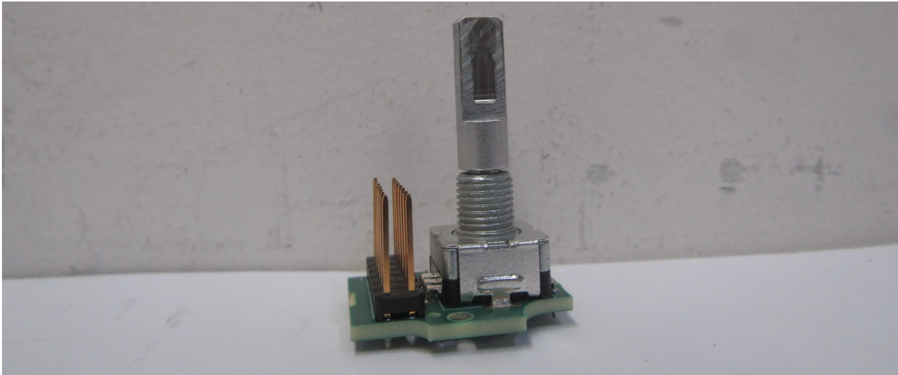
Photograph 7: Channel Mezzanine PCB top
