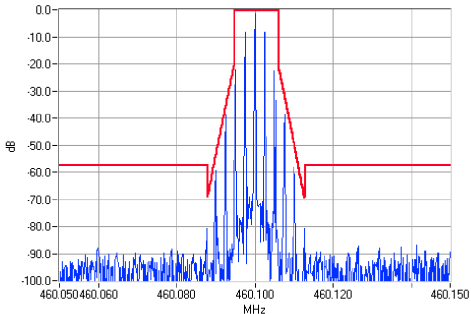
Analogue Modulation 460.1000MHz Mask D 5W Pass
