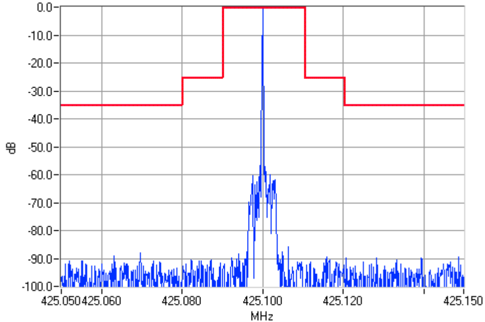
Unmodulated 425.1000MHz Mask B 50W Pass
