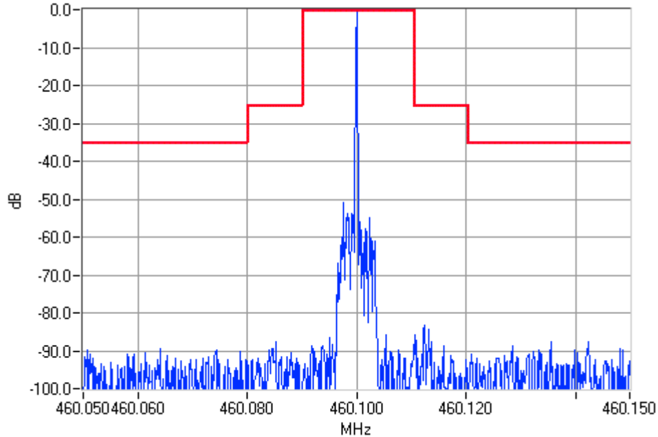
Unmodulated 460.1000MHz Mask B 5W Pass
