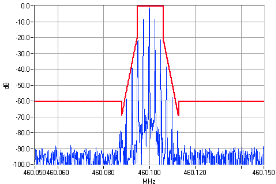
Analogue Modulation 460.1000MHz Mask D 10W Pass
