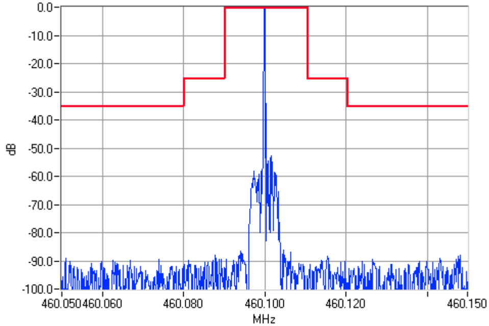
Unmodulated 460.1000MHz Mask B 100W Pass
