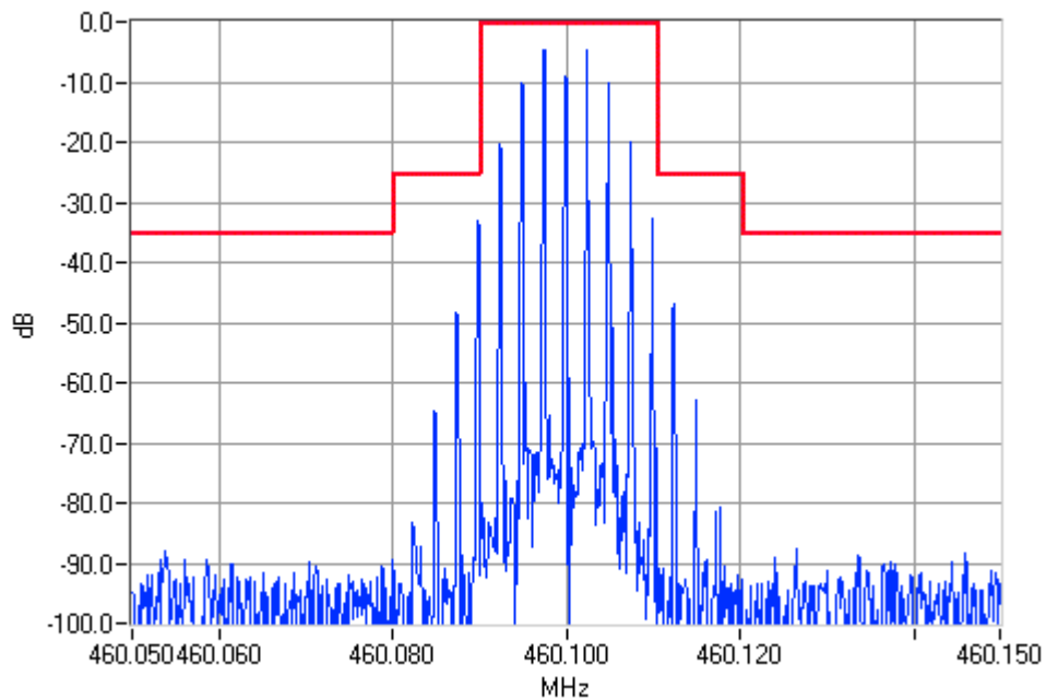
Analogue Modulation 460.1000MHz Mask B 100W Pass
