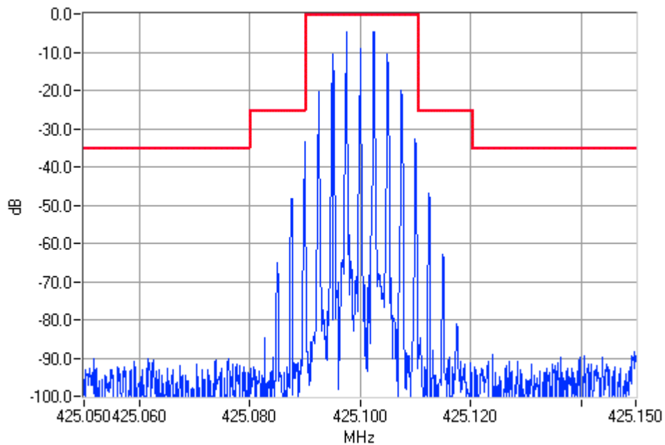
Analogue Modulation 425.1000MHz Mask B 5W Pass
