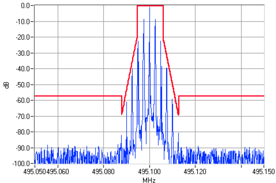
Analogue Modulation 495.1000MHz Mask D 5W Pass
