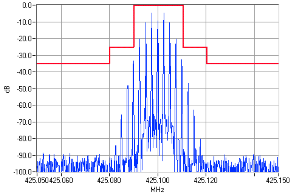
Analogue Modulation 425.1000MHz Mask B 10W Pass
