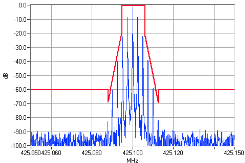
Analogue Modulation 425.1000MHz Mask D 10W Pass
