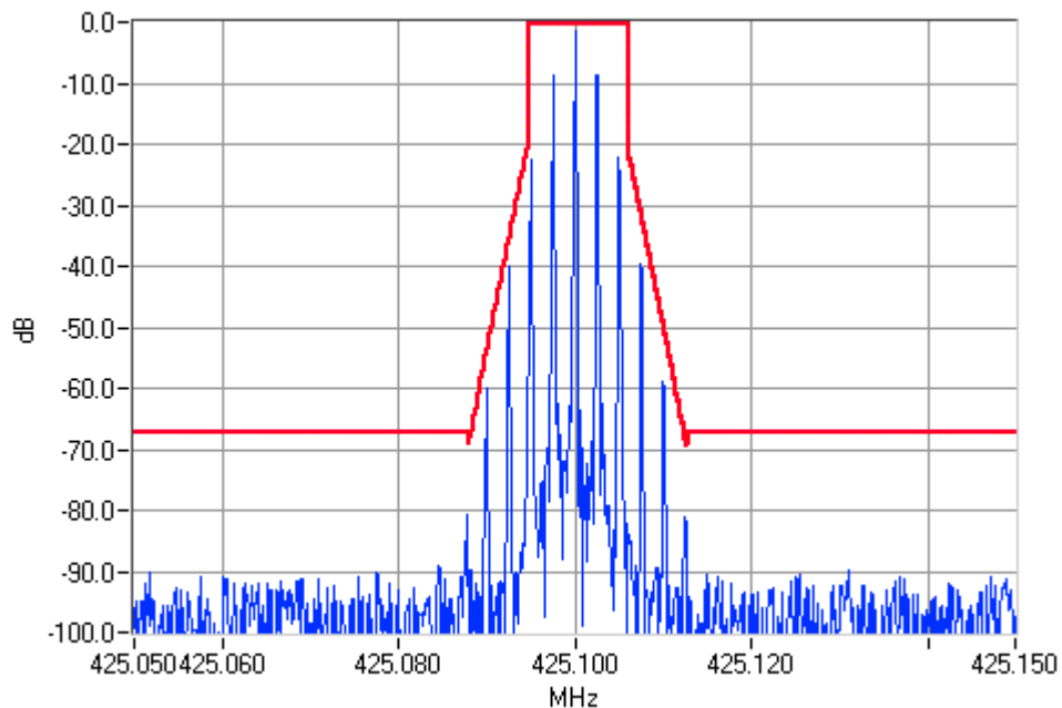
Analogue Modulation 425.1000MHz Mask D 50W Pass
