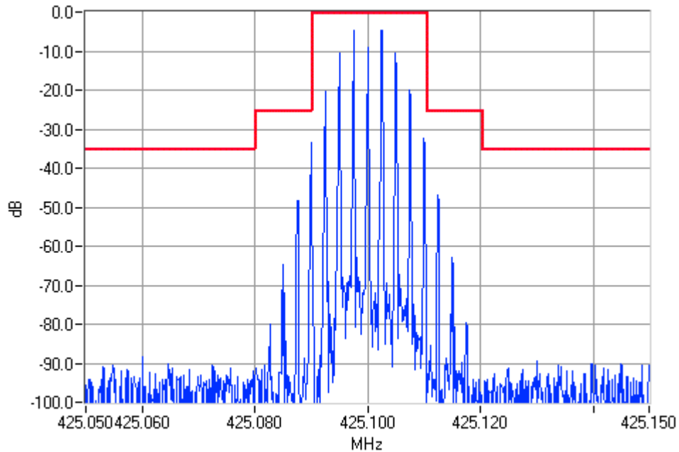
Analogue Modulation 425.1000MHz Mask B 50W Pass
