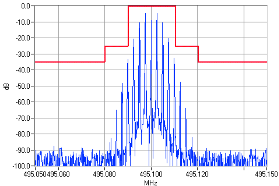
Analogue Modulation 495.1000MHz Mask B 5W Pass
