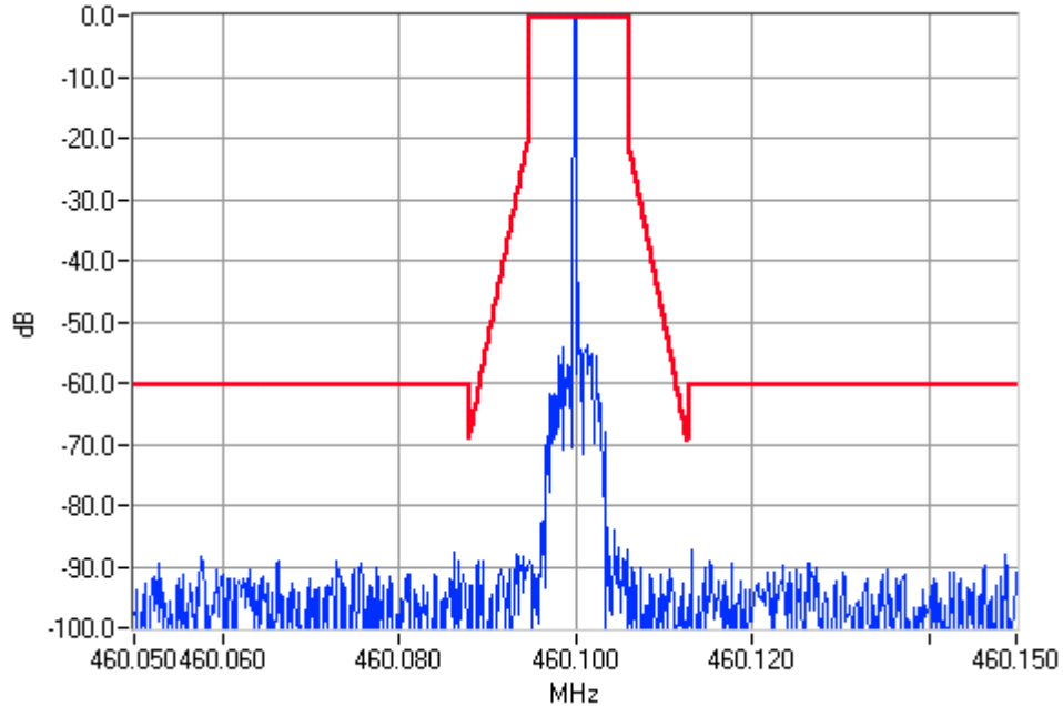
Unmodulated 460.1000MHz Mask D 10W Pass
