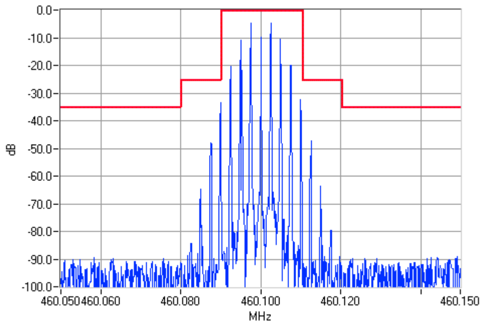
Analogue Modulation 460.1000MHz Mask B 5W Pass
