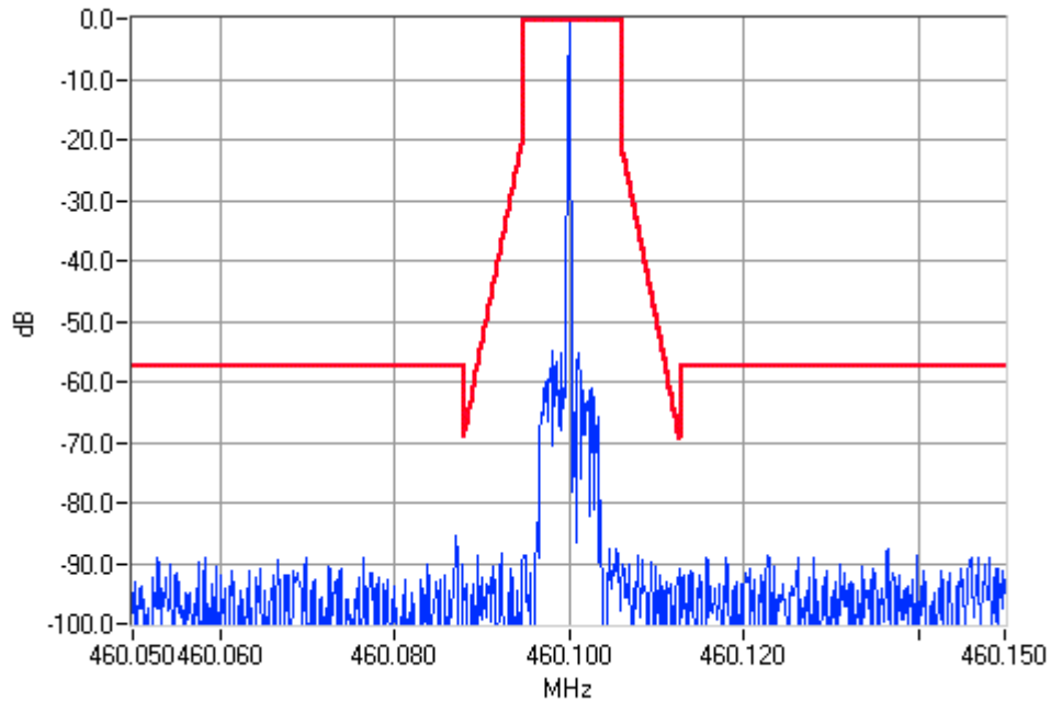
Unmodulated 460.1000MHz Mask D 5W Pass
