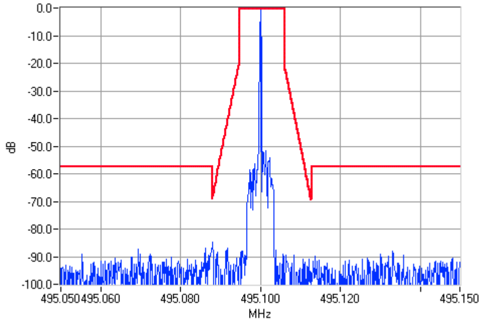
Unmodulated 495.1000MHz Mask D 5W Pass
