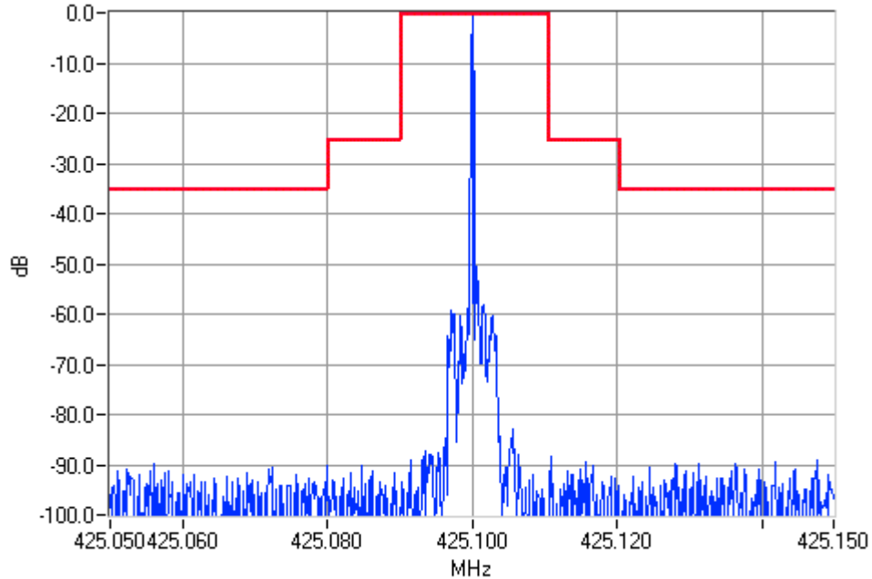
Unmodulated 425.1000MHz Mask B 10W Pass
