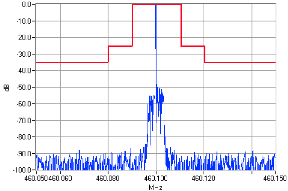
Unmodulated 460.1000MHz Mask B 10W Pass
