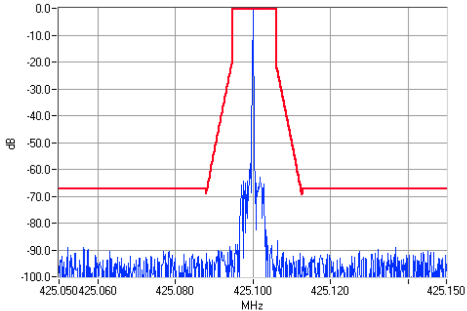
Unmodulated 425.1000MHz Mask D 50W Pass
