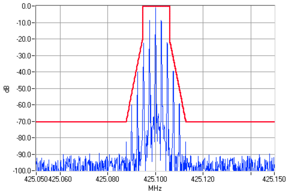
Analogue Modulation 425.1000MHz Mask D 100W Pass
