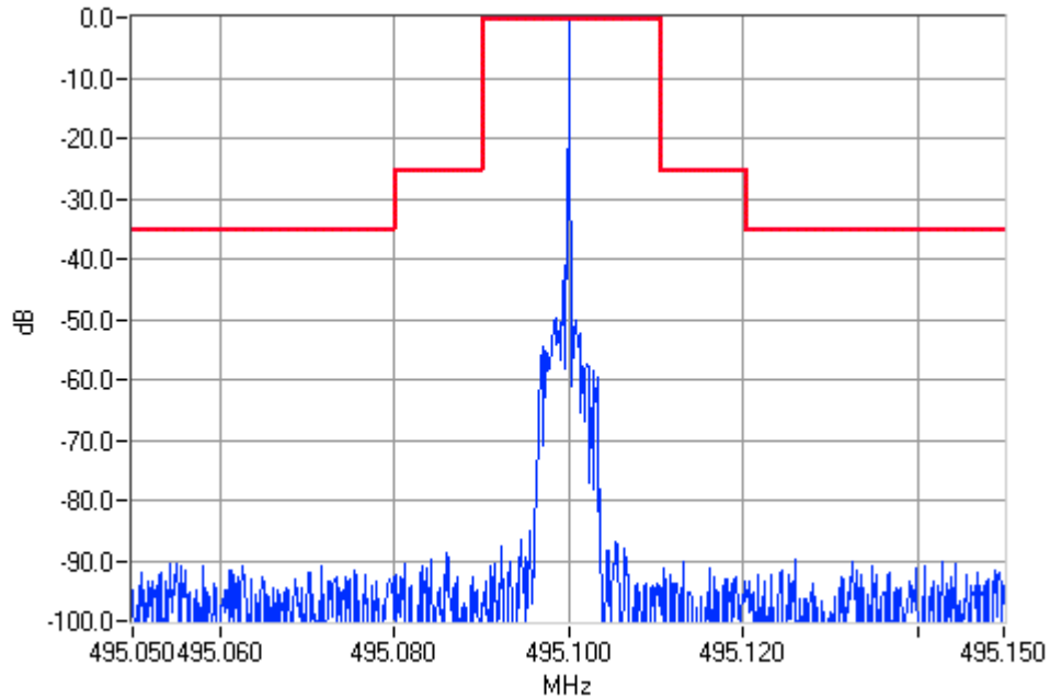
Unmodulated 495.1000MHz Mask B 50W Pass
