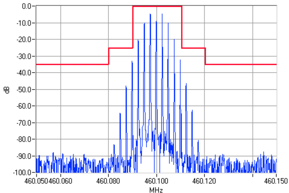
Analogue Modulation 460.1000MHz Mask B 10W Pass
