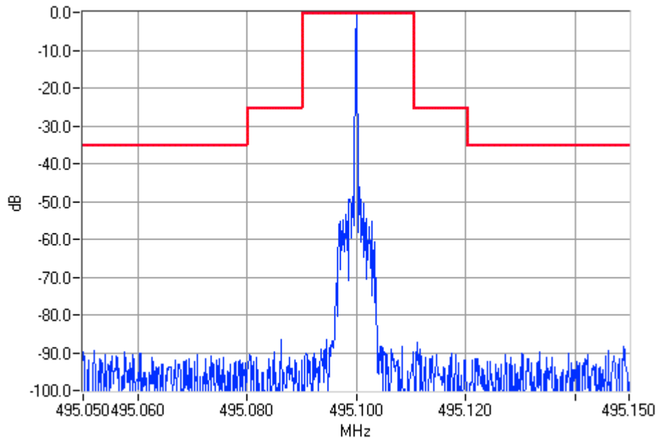
Unmodulated 495.1000MHz Mask B 5W Pass
