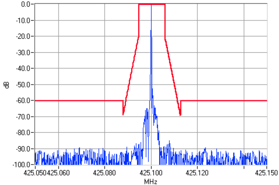
Unmodulated 425.1000MHz Mask D 10W Pass
