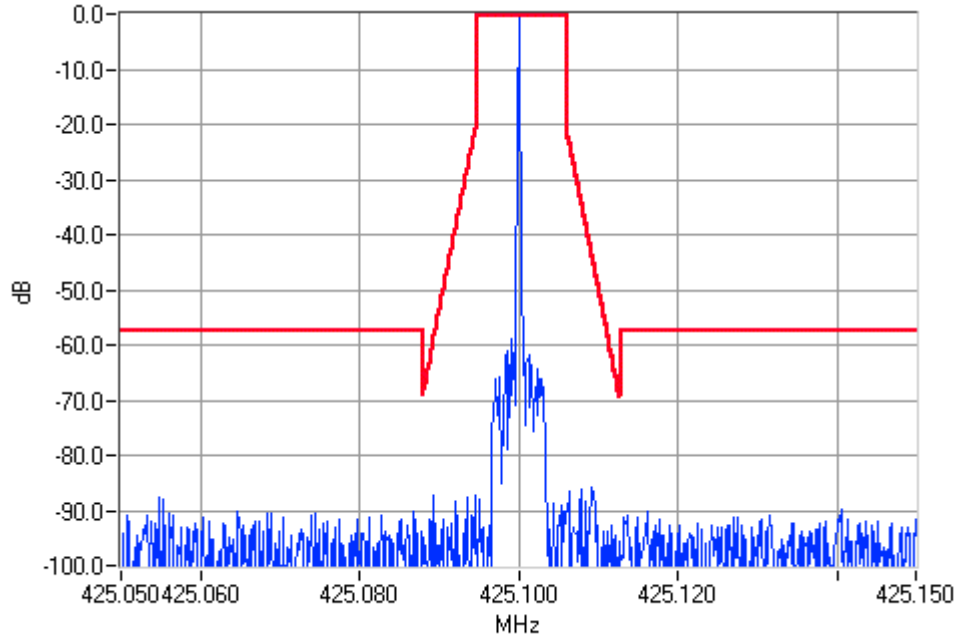
Unmodulated 425.1000MHz Mask D 5W Pass
