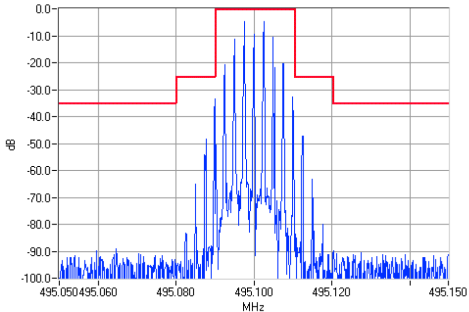
Analogue Modulation 495.1000MHz Mask B 50W Pass
