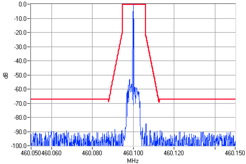
Unmodulated 460.1000MHz Mask D 50W Pass
