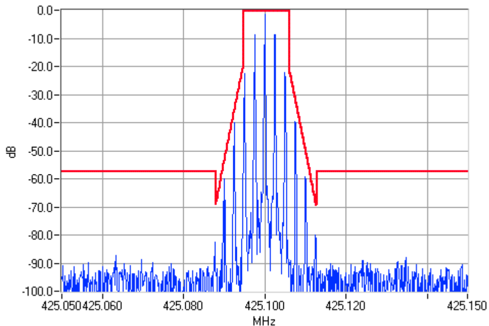
Analogue Modulation 425.1000MHz Mask D 5W Pass
