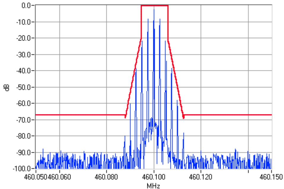
Analogue Modulation 460.1000MHz Mask D 50W Pass
