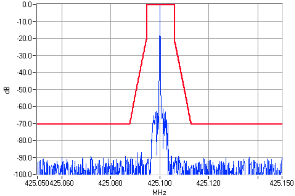
Unmodulated 425.1000MHz Mask D 100W Pass
