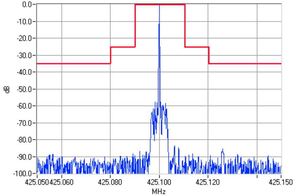
Unmodulated 425.1000MHz Mask B 5W Pass
