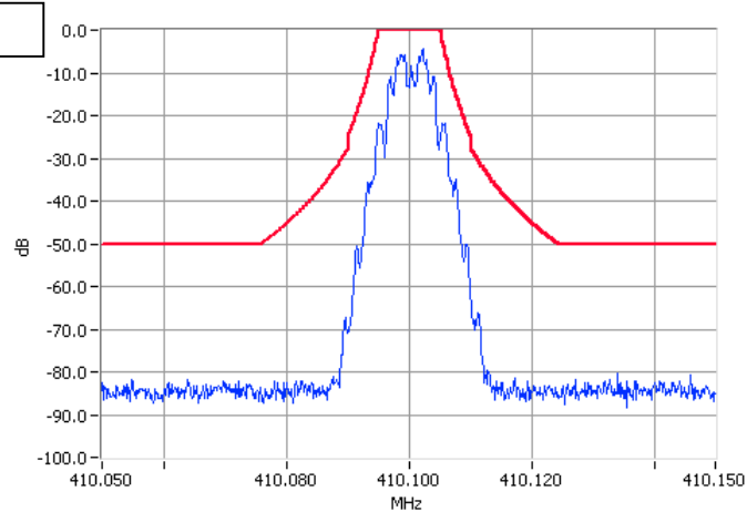
Digital Modulation 410.1000MHz Mask C 1W Pass RBW=300Hz VBW=3000Hz
