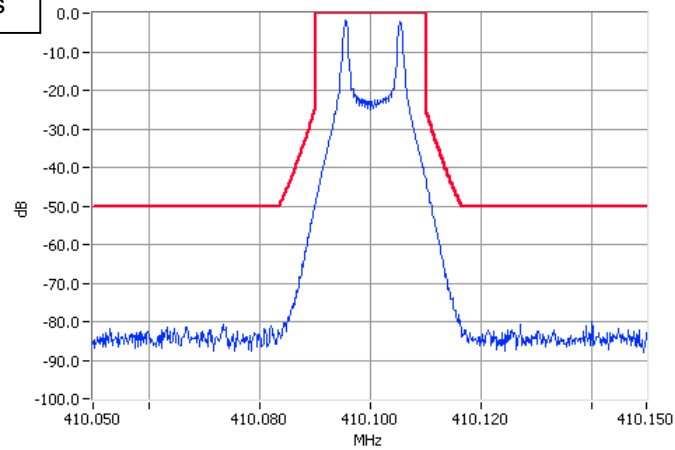
Paging Modulation 410.1000MHz Mask G 1W Pass RBW=300Hz VBW=3000Hz
