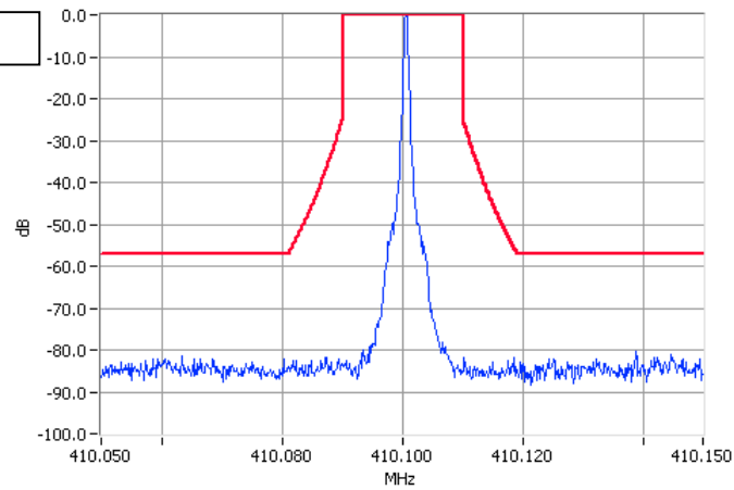
Unmodulated 410.1000MHz Mask G 5W Pass RBW=300Hz VBW=3000Hz
