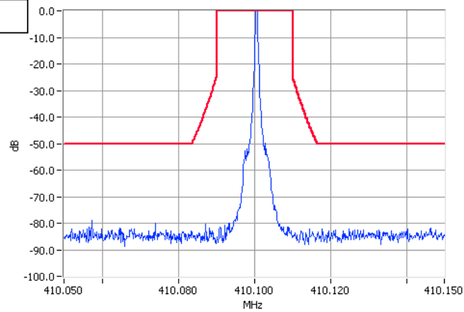
Unmodulated 410.1000MHz Mask G 1W Pass RBW=300Hz VBW=3000Hz
