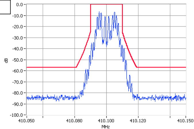
Paging Modulation 410.1000MHz Mask G 5W Pass RBW=300Hz VBW=3000Hz
