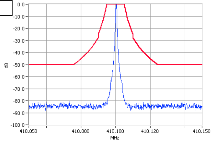
Unmodulated 410.1000MHz Mask C 1W Pass RBW=300Hz VBW=3000Hz
