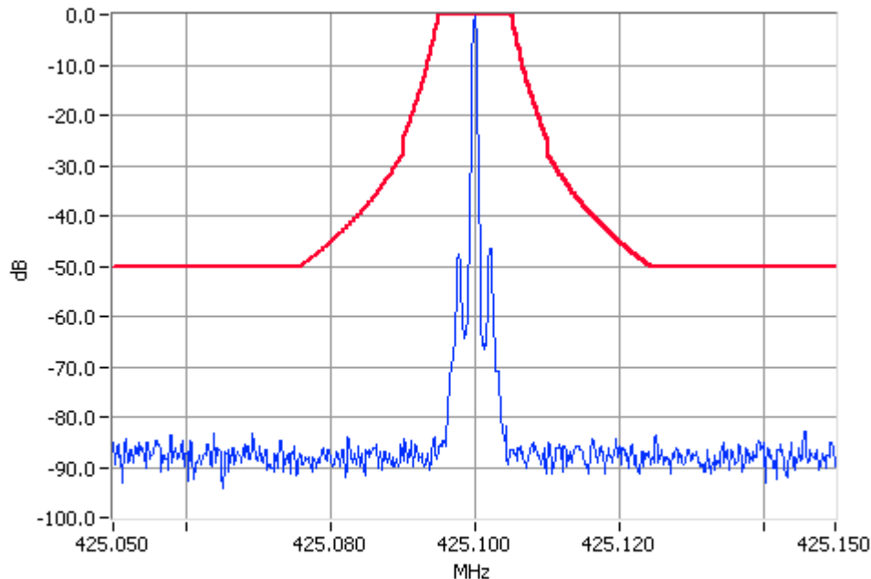
Unmodulated 425.1000MHz Mask C 100W Pass RBW=300Hz VBW=3000Hz
