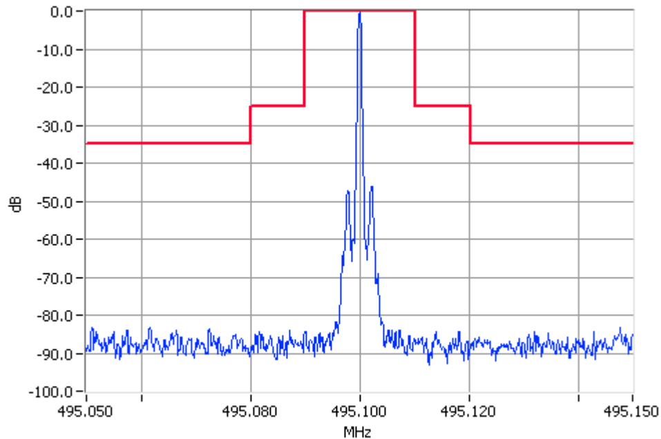
Unmodulated 495.1000MHz Mask B 100W Pass RBW=300Hz VBW=3000Hz
