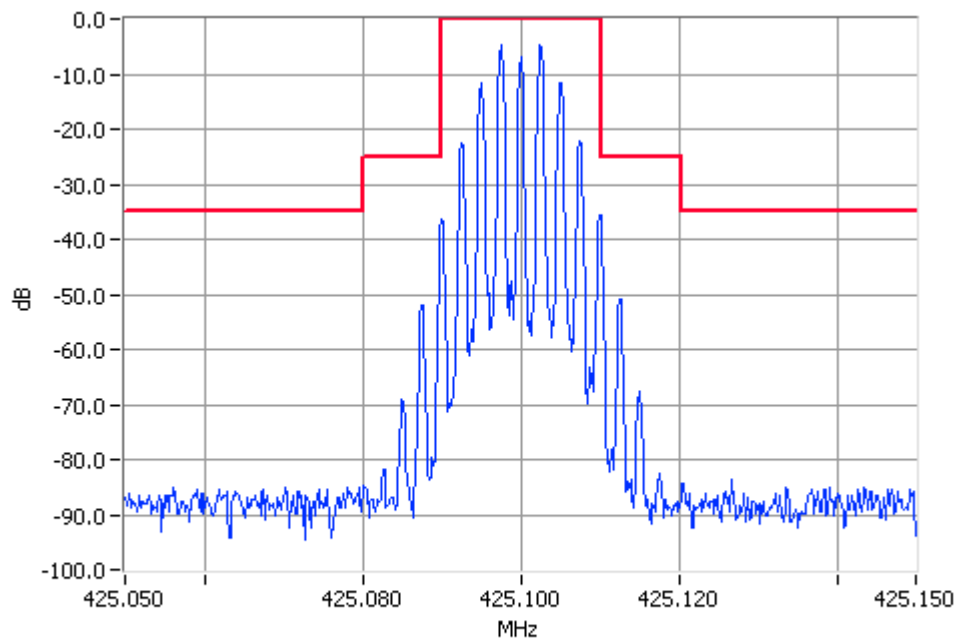
Analogue Modulation 425.1000MHz Mask B 100W Pass RBW=300Hz VBW=3000Hz
