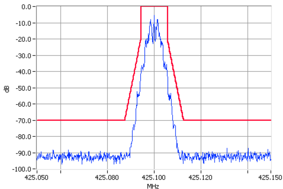
Digital Modulation 425.1000MHz Mask D 100W Pass RBW=100Hz VBW=1000Hz
