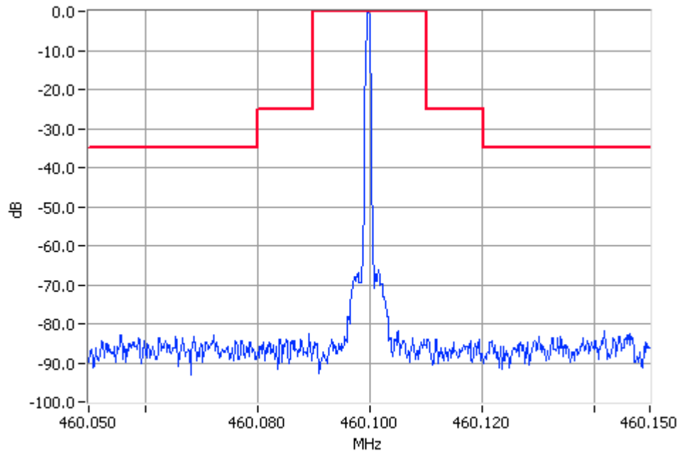
Unmodulated 460.1000MHz Mask B 100W Pass RBW=300Hz VBW=3000Hz
