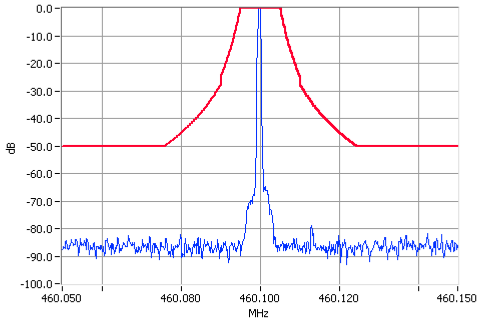
Unmodulated 460.1000MHz Mask C 100W Pass RBW=300Hz VBW=3000Hz
