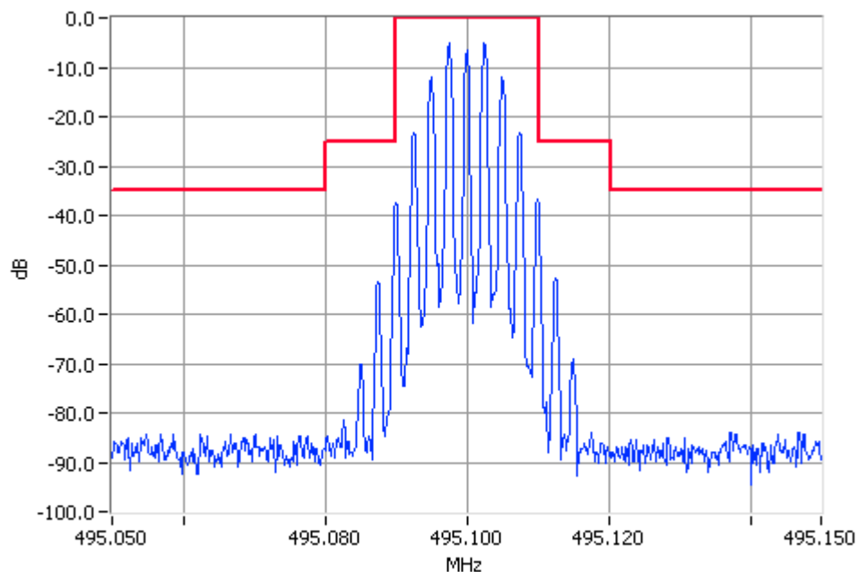
Analogue Modulation 495.1000MHz Mask B 100W Pass RBW=300Hz VBW=3000Hz
