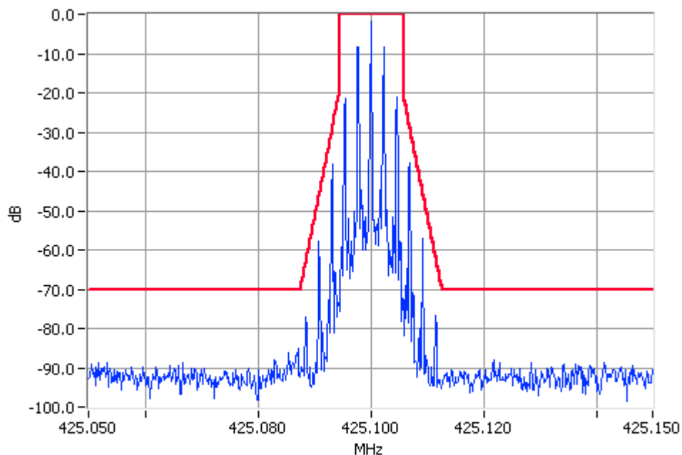
Analogue Modulation 425.1000MHz Mask D 100W Pass RBW=100Hz VBW=1000Hz
