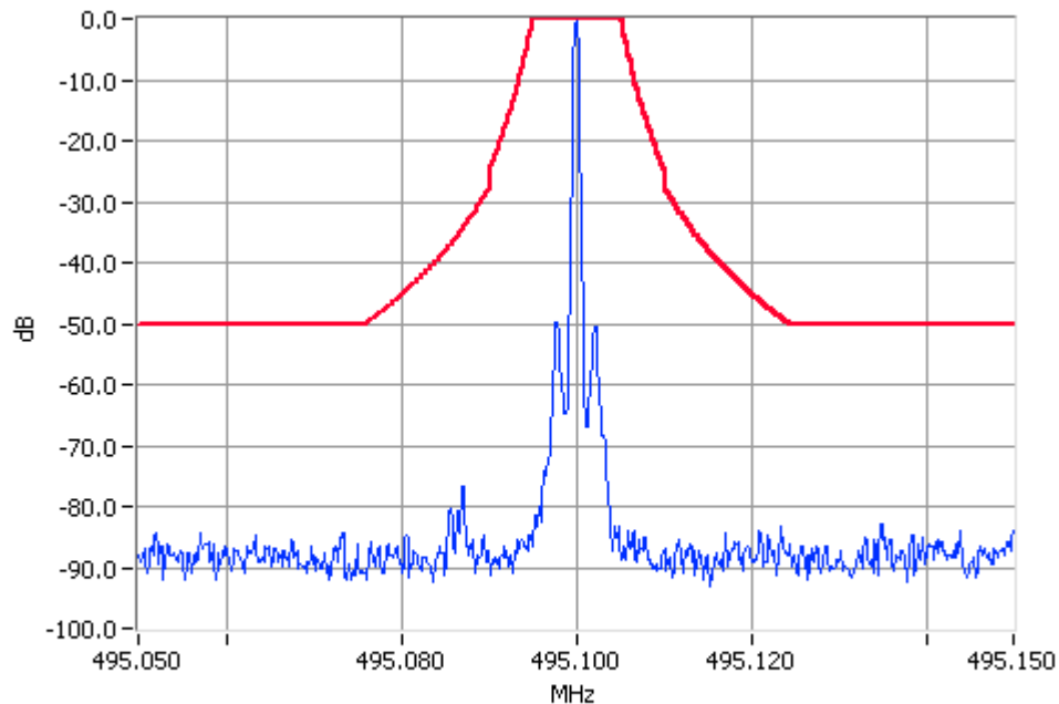
Unmodulated 495.1000MHz Mask C 100W Pass RBW=300Hz VBW=3000Hz
