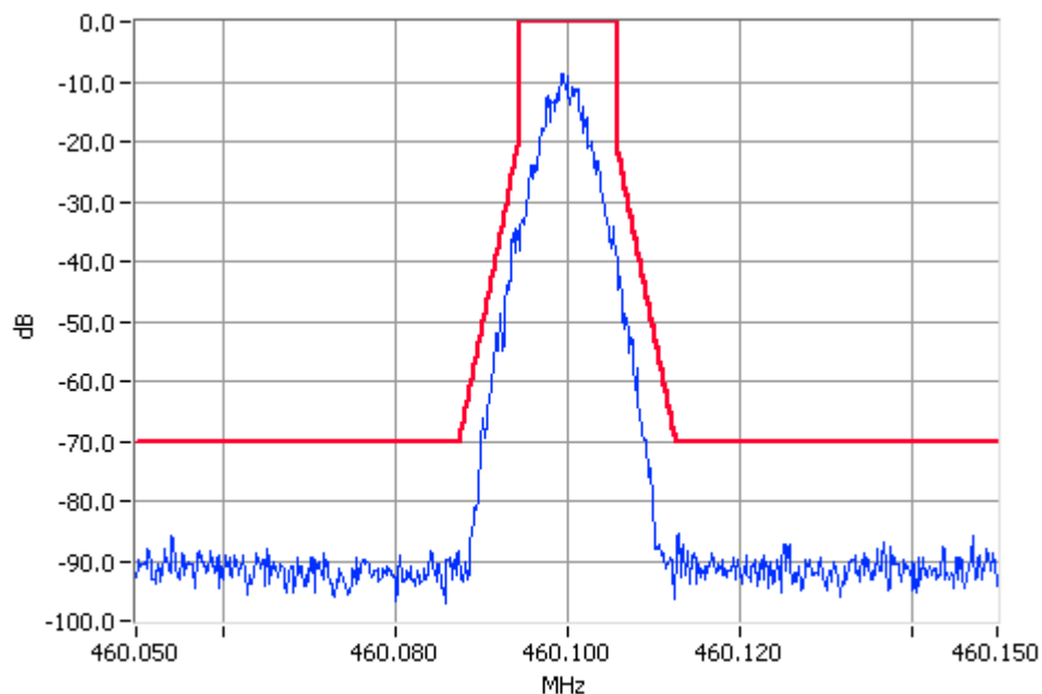
Digital Modulation 460.1000MHz Mask D 100W Pass RBW=100Hz VBW=1000Hz
