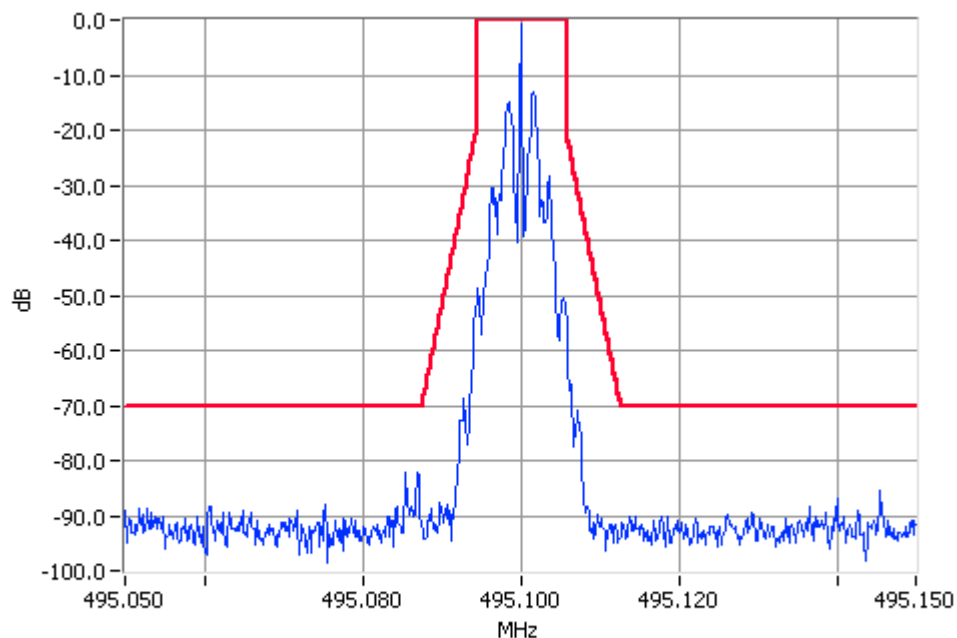
Digital Modulation 495.1000MHz Mask D 100W Pass RBW=100Hz VBW=1000Hz
