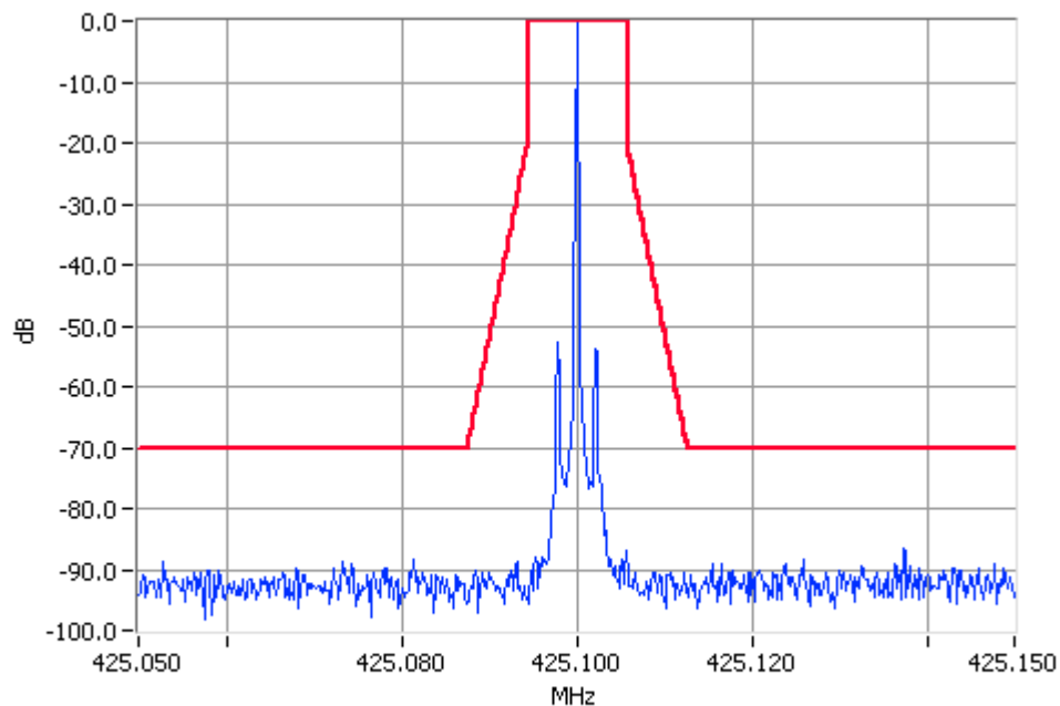
Unmodulated 425.1000MHz Mask D 100W Pass RBW=100Hz VBW=1000Hz
