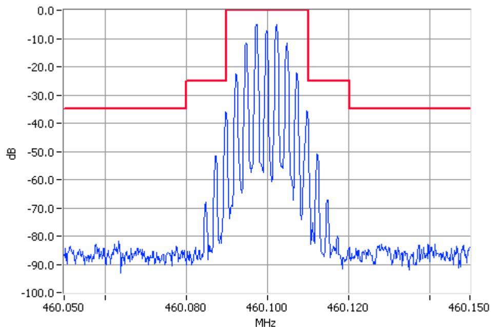
Analogue Modulation 460.1000MHz Mask B 100W Pass RBW=300Hz VBW=3000Hz
