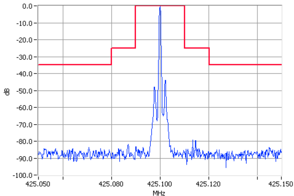
Unmodulated 425.1000MHz Mask B 100W Pass RBW=300Hz VBW=3000Hz
