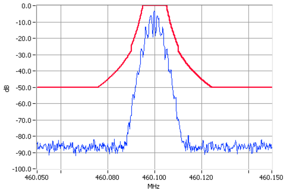
Digital Modulation 460.1000MHz Mask C 100W Pass RBW=300Hz VBW=3000Hz
