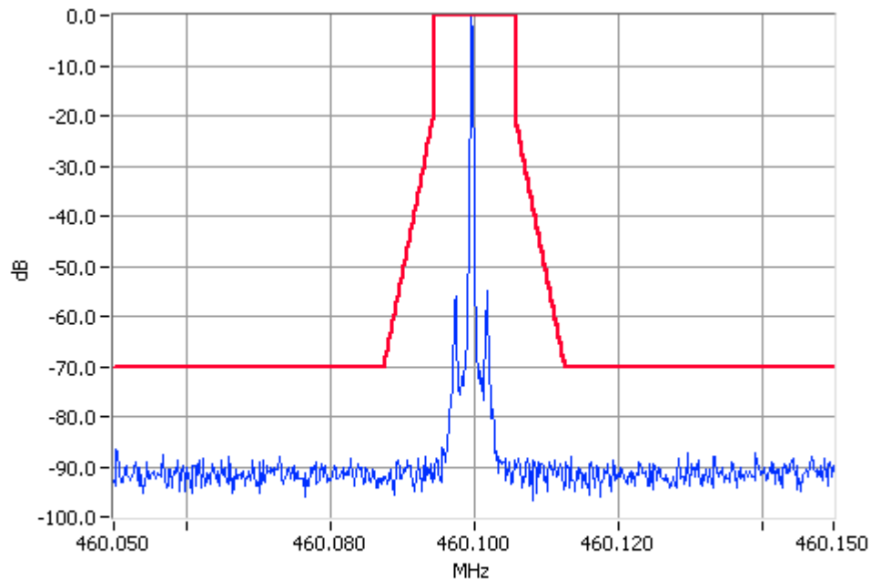
Unmodulated 460.1000MHz Mask D 100W Pass RBW=100Hz VBW=1000Hz
