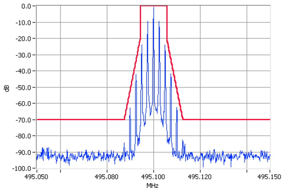
Analogue Modulation 495.1000MHz Mask D 100W Pass RBW=100Hz VBW=1000Hz
