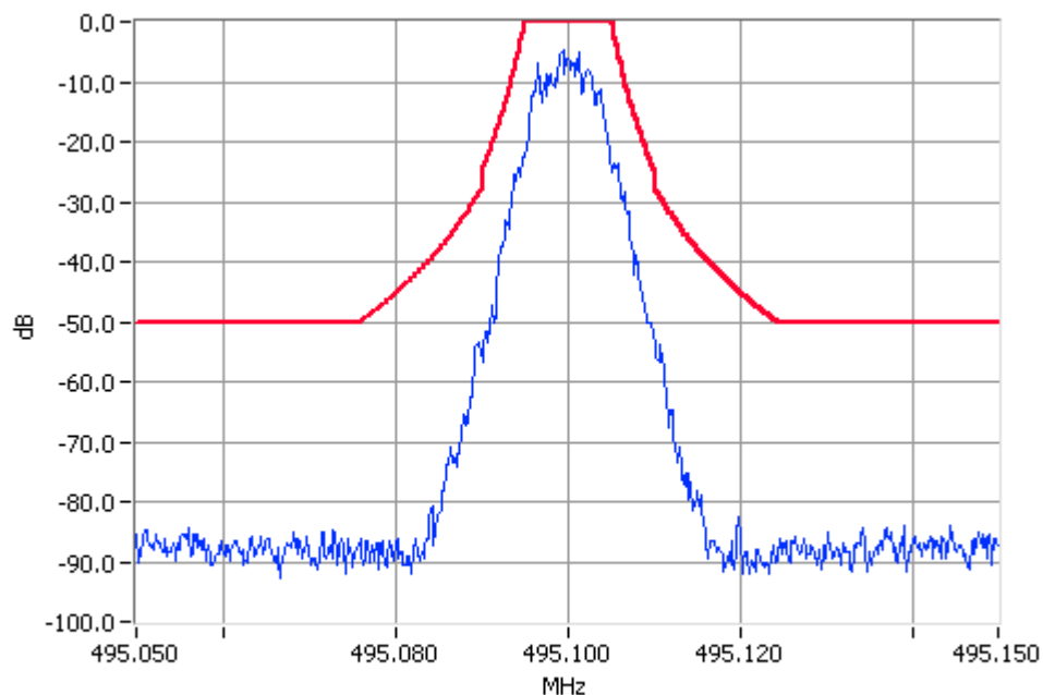
Digital Modulation 495.1000MHz Mask C 100W Pass RBW=300Hz VBW=3000Hz
