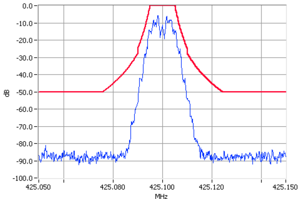
Digital Modulation 425.1000MHz Mask C 100W Pass RBW=300Hz VBW=3000Hz
