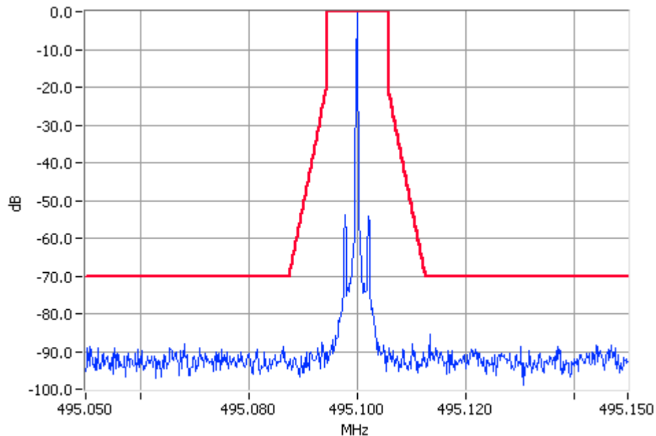
Unmodulated 495.1000MHz Mask D 100W Pass RBW=100Hz VBW=1000Hz
