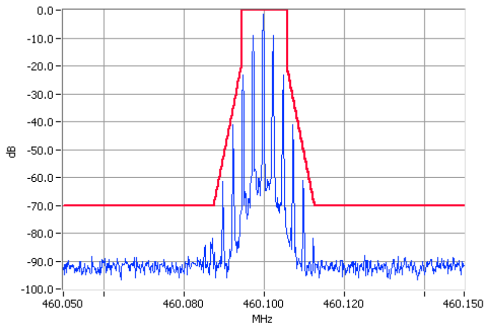
Analogue Modulation 460.1000MHz Mask D 100W Pass RBW=100Hz VBW=1000Hz
