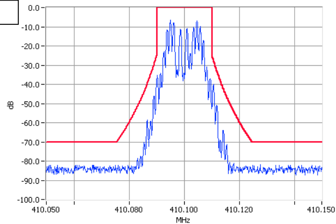
Paging Modulation 410.1000MHz Mask G 100W Pass RBW=300Hz VBW=3000Hz
