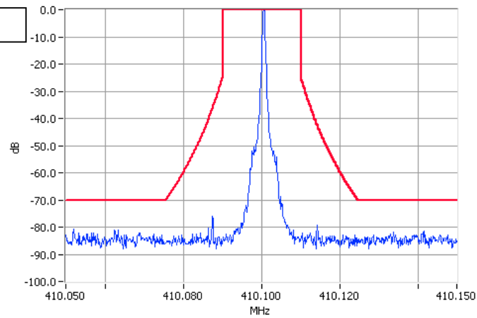
Unmodulated 410.1000MHz Mask G 100W Pass RBW=300Hz VBW=3000Hz
