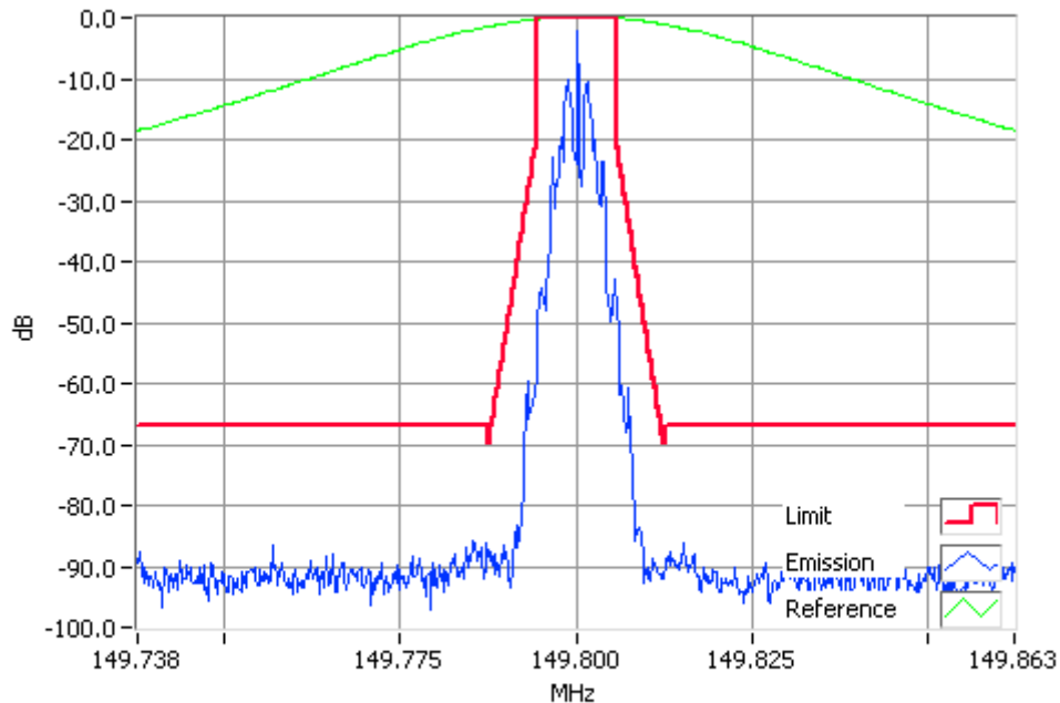
FFSK 149.8000MHz Mask D 50W RBW=100Hz, VBW=1000Hz, Detector Mode=Peak Result=Pass
