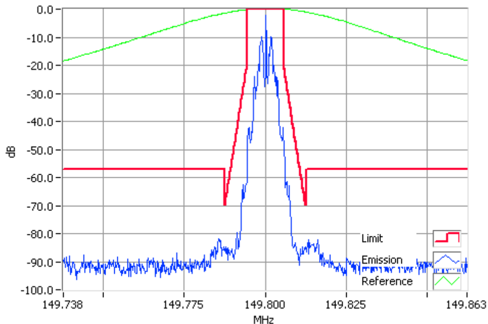
FFSK 149.8000MHz Mask D 5W RBW=100Hz, VBW=1000Hz, Detector Mode=Peak Result=Pass
