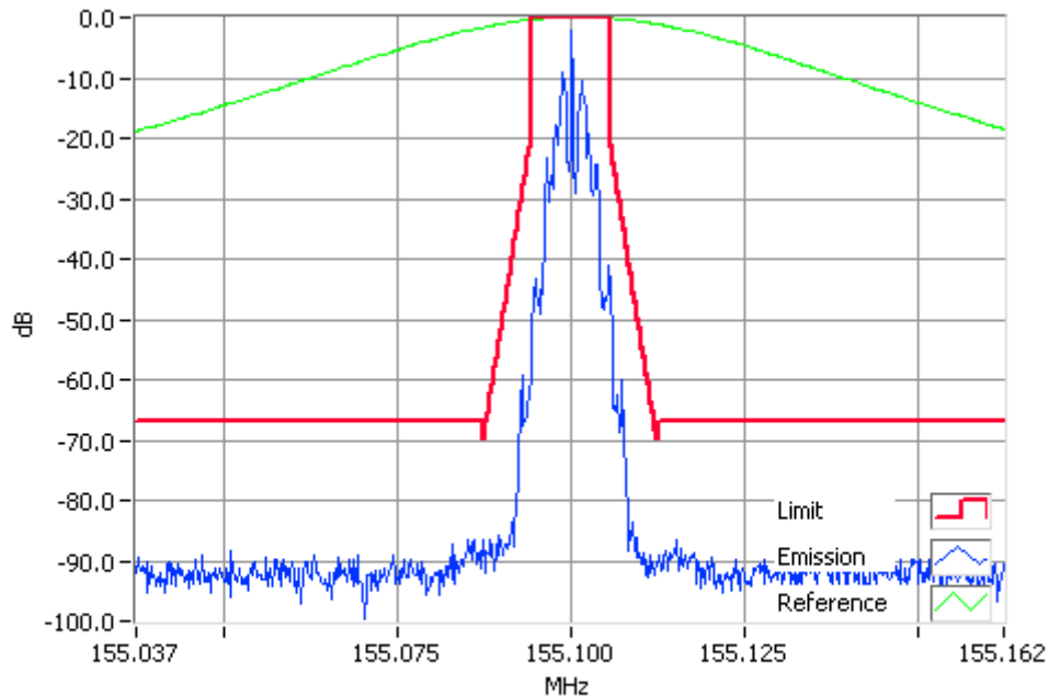
FFSK 155.1000MHz Mask D 50W RBW=100Hz, VBW=1000Hz, Detector Mode=Peak Result=Pass
