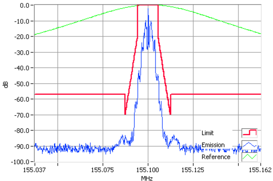
FFSK 155.1000MHz Mask D 5W RBW=100Hz, VBW=1000Hz, Detector Mode=Peak Result=Pass
