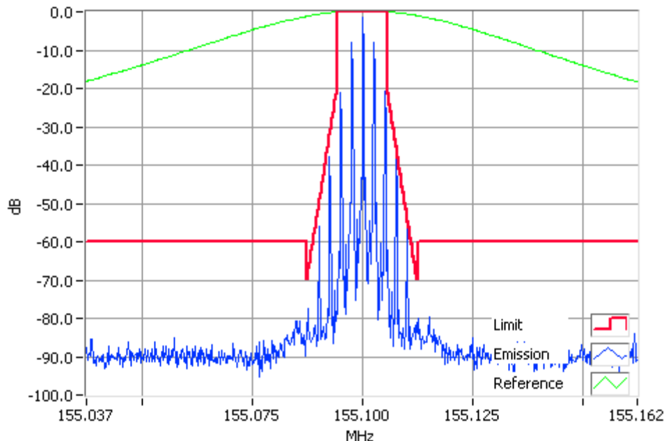
Analogue Modulation 155.1000MHz Mask D 10W RBW=100Hz, VBW=1000Hz, Detector Mode=Peak Result=Pass
