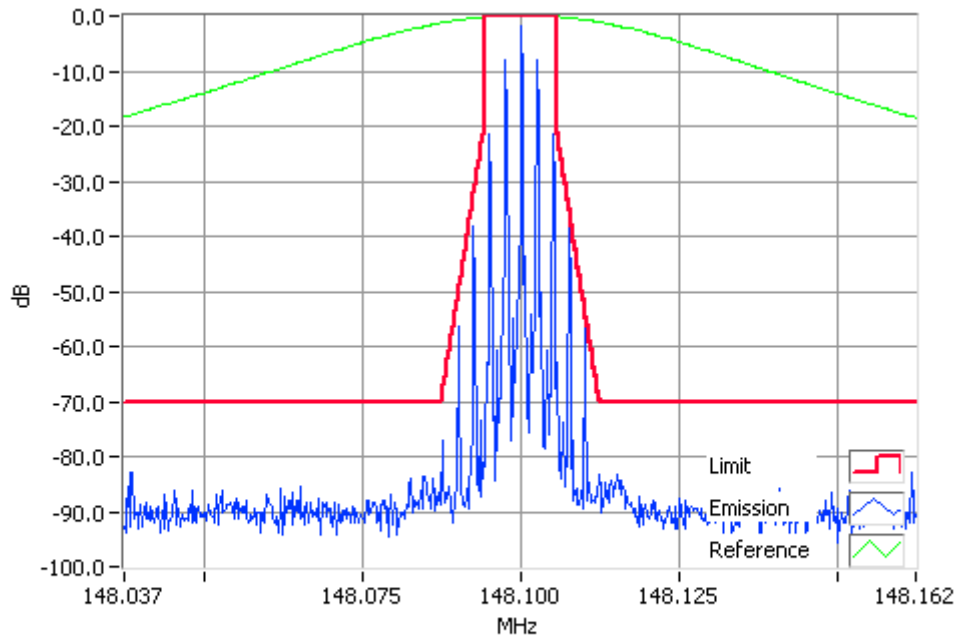
Analogue Modulation 148.1000MHz Mask D 100W RBW=100Hz, VBW=1000Hz, Detector Mode=Peak Result=Pass
