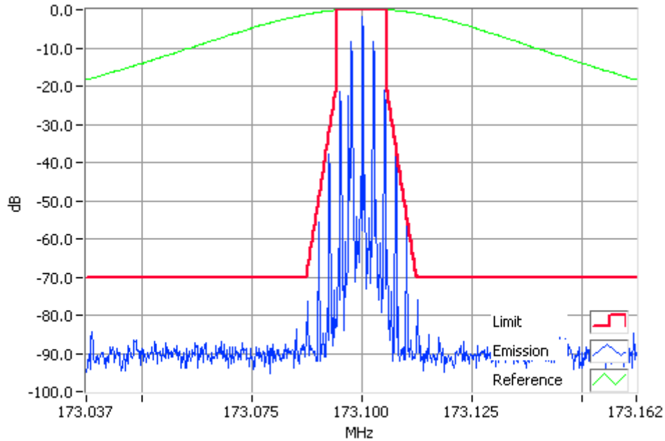
Analogue Modulation 173.1000MHz Mask D 100W RBW=100Hz, VBW=1000Hz, Detector Mode=Peak Result=Pass
