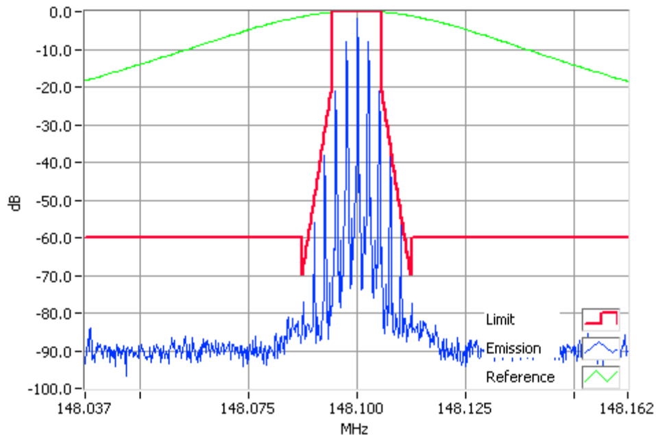
Analogue Modulation 148.1000MHz Mask D 10W RBW=100Hz, VBW=1000Hz, Detector Mode=Peak Result=Pass
