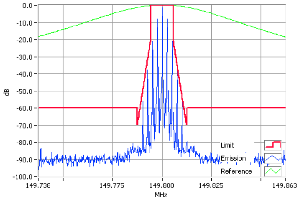
Analogue Modulation 149.8000MHz Mask D 10W RBW=100Hz, VBW=1000Hz, Detector Mode=Peak Result=Pass
