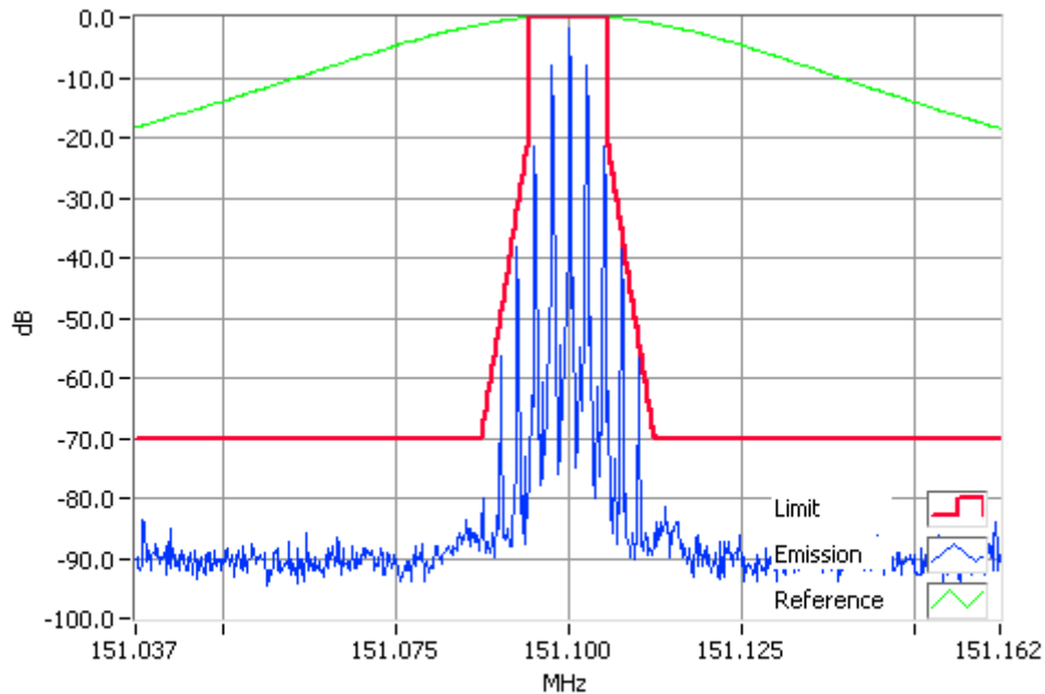
Analogue Modulation 151.1000MHz Mask D 100W RBW=100Hz, VBW=1000Hz, Detector Mode=Peak Result=Pass
