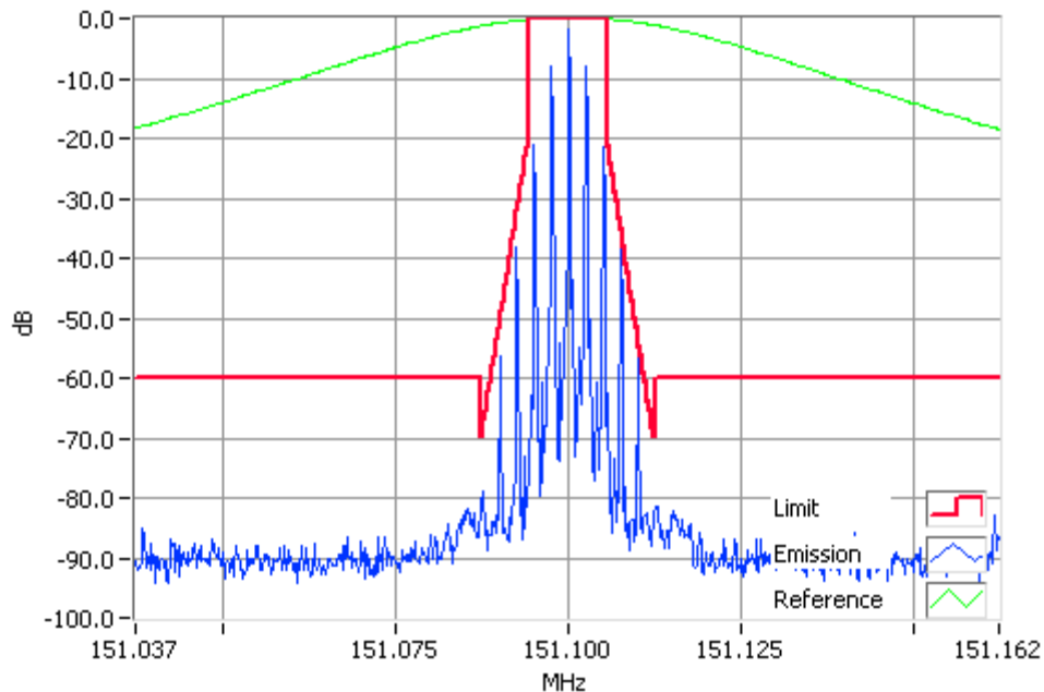
Analogue Modulation 151.1000MHz Mask D 10W RBW=100Hz, VBW=1000Hz, Detector Mode=Peak Result=Pass
