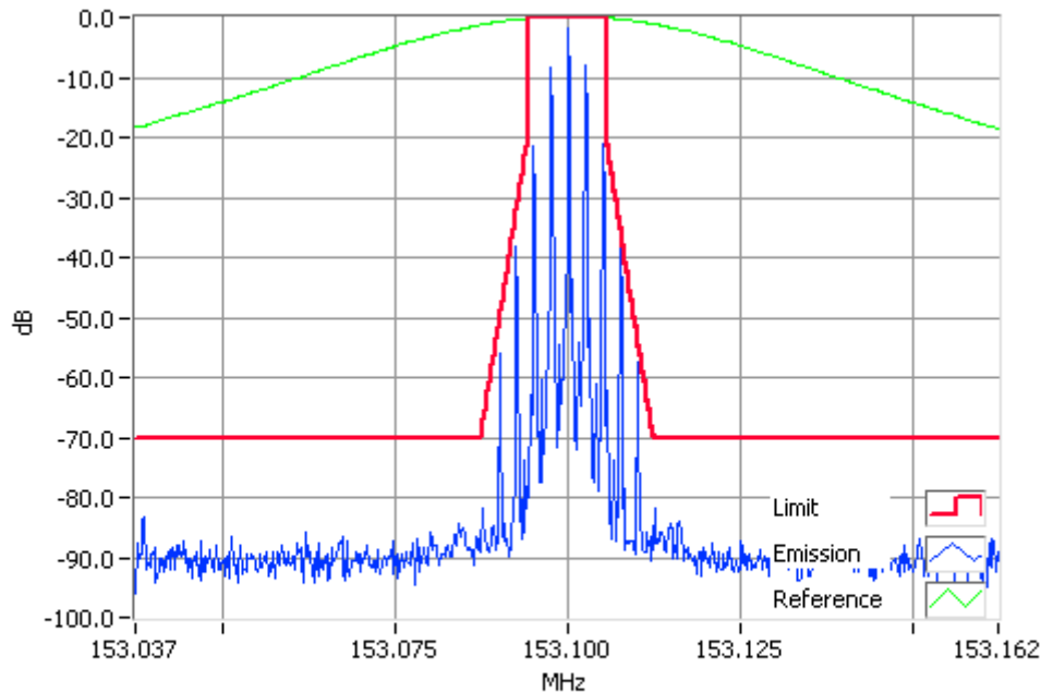
Analogue Modulation 153.1000MHz Mask D 100W RBW=100Hz, VBW=1000Hz, Detector Mode=Peak Result=Pass
