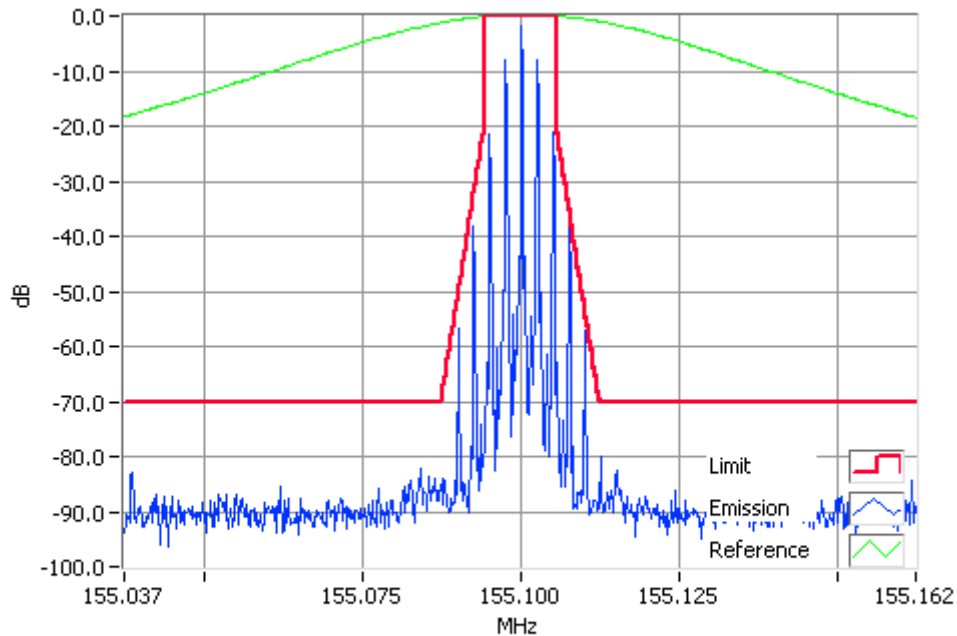
Analogue Modulation 155.1000MHz Mask D 100W RBW=100Hz, VBW=1000Hz, Detector Mode=Peak Result=Pass
