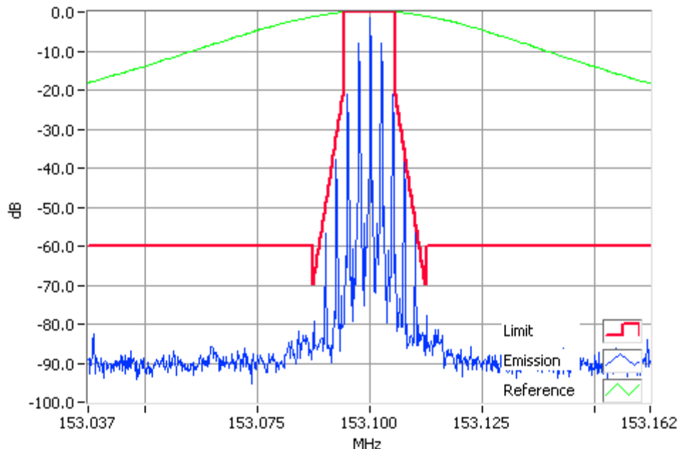
Analogue Modulation 153.1000MHz Mask D 10W RBW=100Hz, VBW=1000Hz, Detector Mode=Peak Result=Pass
