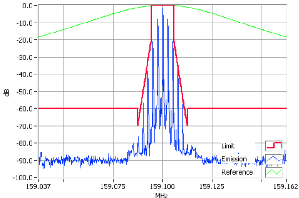
Analogue Modulation 159.1000MHz Mask D 10W RBW=100Hz, VBW=1000Hz, Detector Mode=Peak Result=Pass
