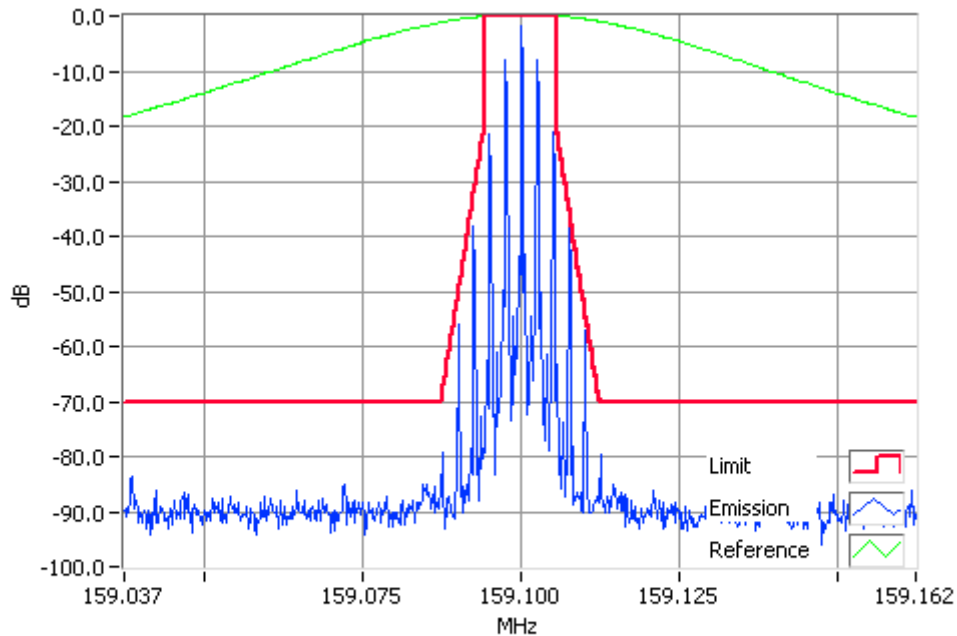
Analogue Modulation 159.1000MHz Mask D 100W RBW=100Hz, VBW=1000Hz, Detector Mode=Peak Result=Pass
