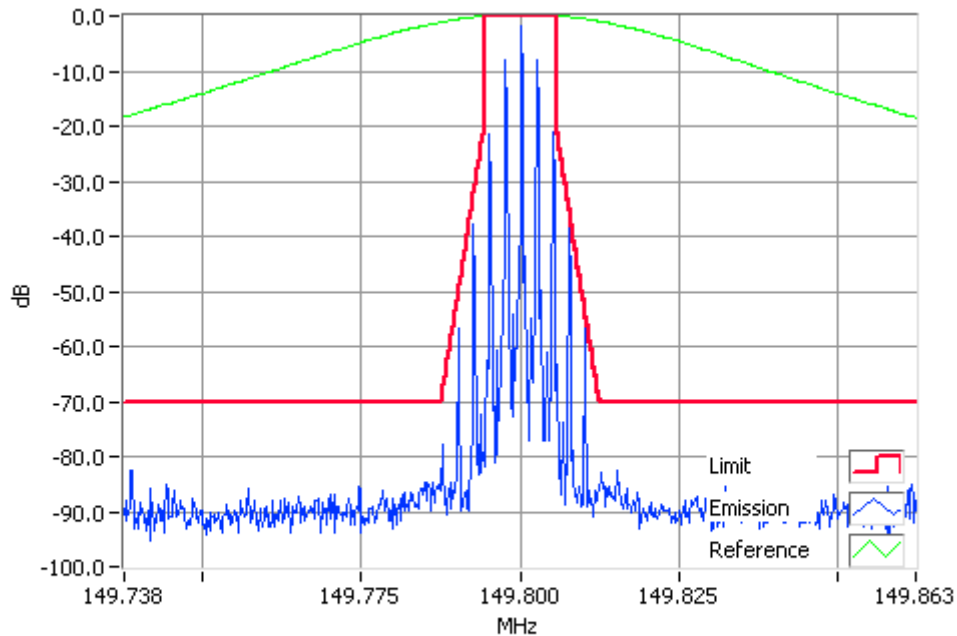
Analogue Modulation 149.8000MHz Mask D 100W RBW=100Hz, VBW=1000Hz, Detector Mode=Peak Result=Pass
