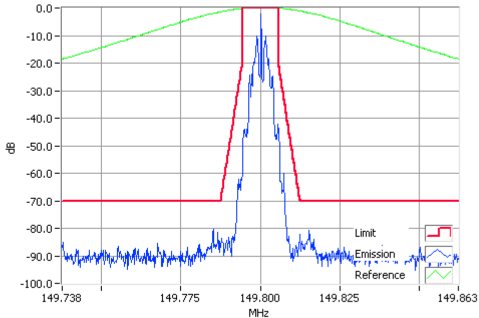
FFSK 149.8000MHz Mask D 100W RBW=100Hz, VBW=1000Hz, Detector Mode=Peak Result=Pass
