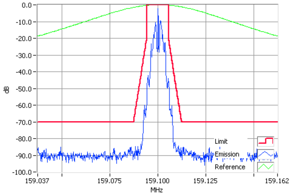
FFSK 159.1000MHz Mask D 100W RBW=100Hz, VBW=1000Hz, Detector Mode=Peak Result=Pass
