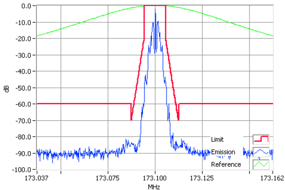
FFSK 173.1000MHz Mask D 10W RBW=100Hz, VBW=1000Hz, Detector Mode=Peak Result=Pass
