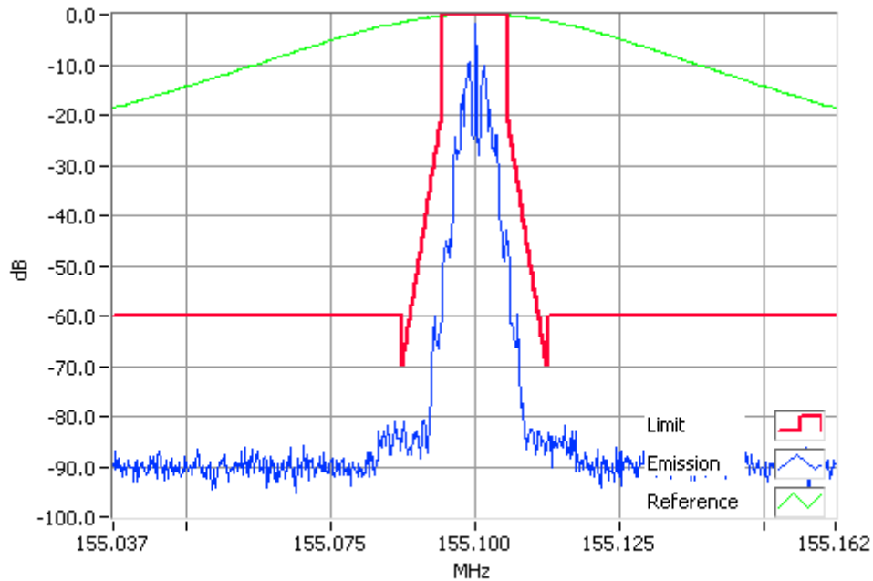
FFSK 155.1000MHz Mask D 10W RBW=100Hz, VBW=1000Hz, Detector Mode=Peak Result=Pass
