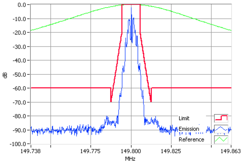
FFSK 149.8000MHz Mask D 10W RBW=100Hz, VBW=1000Hz, Detector Mode=Peak Result=Pass
