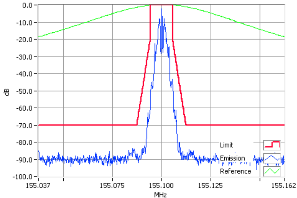
FFSK 155.1000MHz Mask D 100W RBW=100Hz, VBW=1000Hz, Detector Mode=Peak Result=Pass
