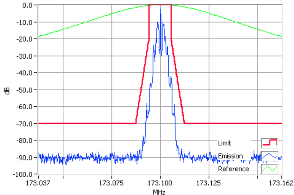
FFSK 173.1000MHz Mask D 100W RBW=100Hz, VBW=1000Hz, Detector Mode=Peak Result=Pass
