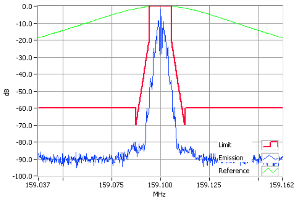
FFSK 159.1000MHz Mask D 10W RBW=100Hz, VBW=1000Hz, Detector Mode=Peak Result=Pass
