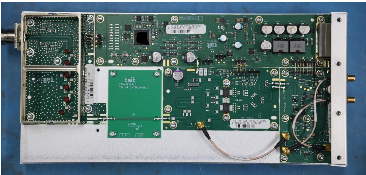
Photograph 20: PA PCB –Top (without cans)
