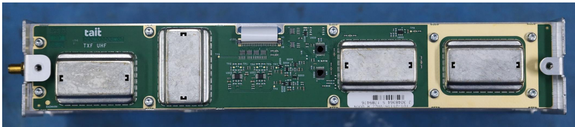
Photograph 11: Reciter TxF PCB - Top
