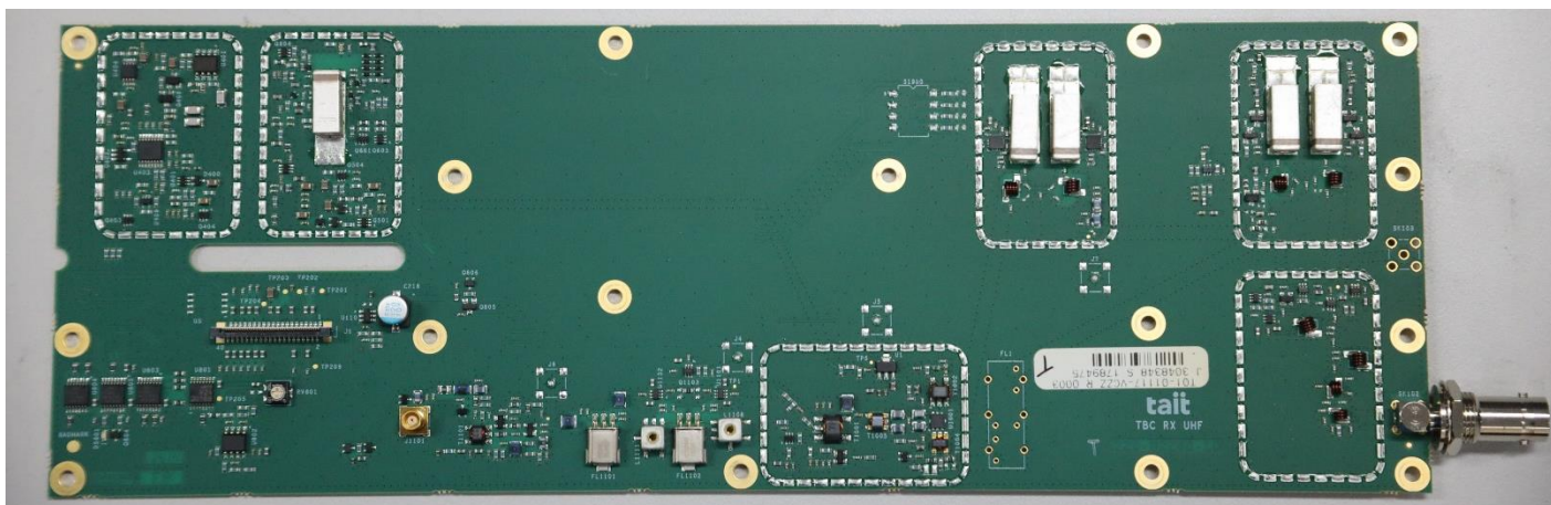
Photograph 9: Reciter Rx PCB – Top (without cans)
