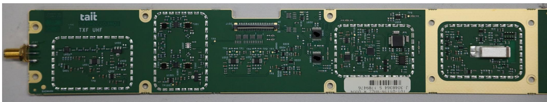
Photograph 12: Reciter TxF PCB – Top (without cans)
