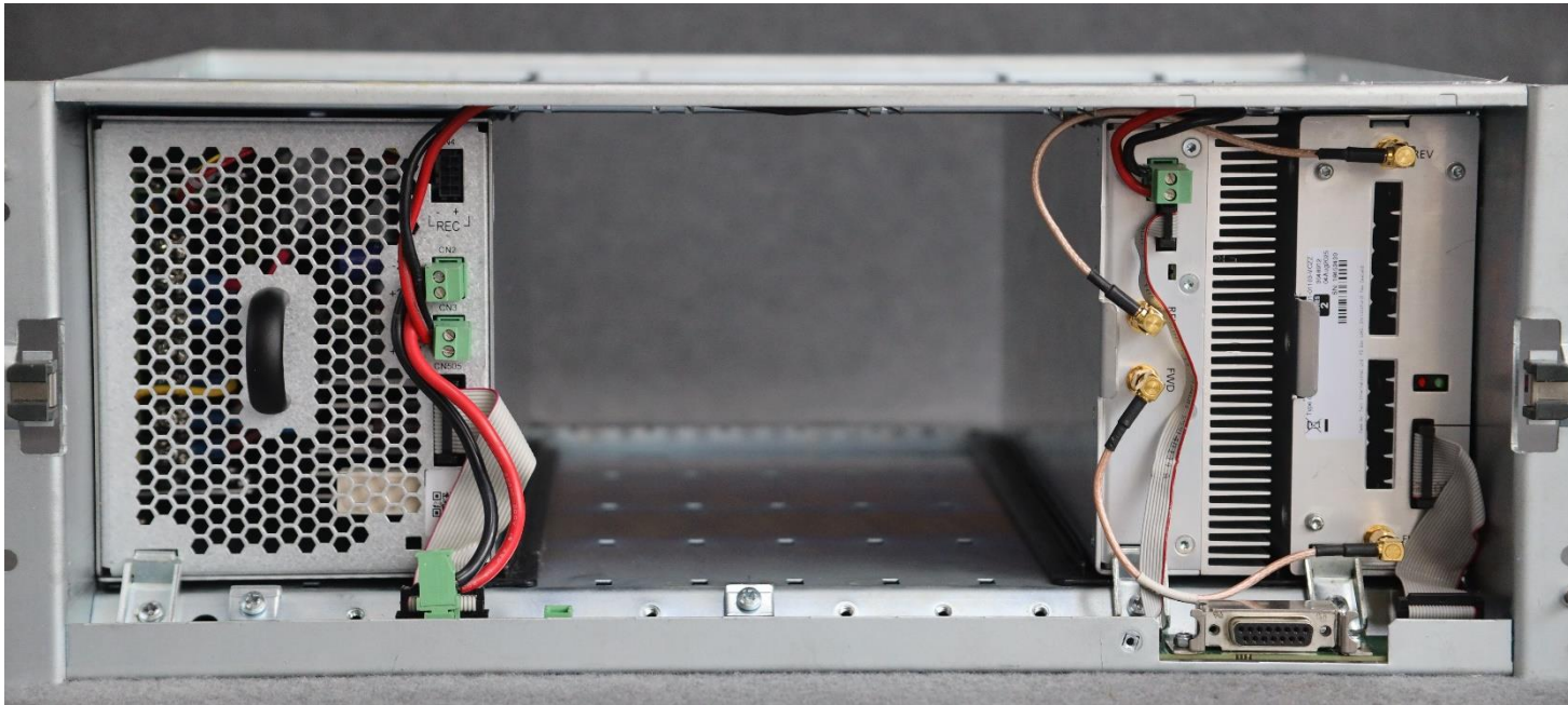
Photograph 01: Base station – Front view – Open
