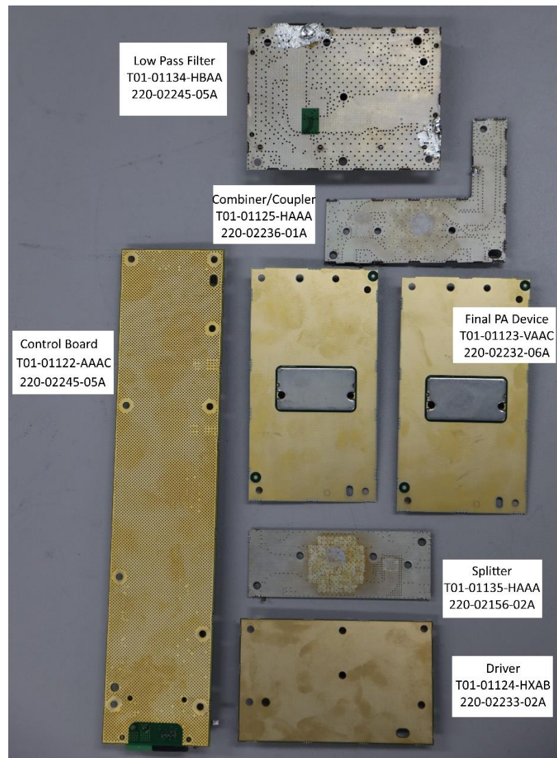
Photograph 21: PA PCB –Bottom
