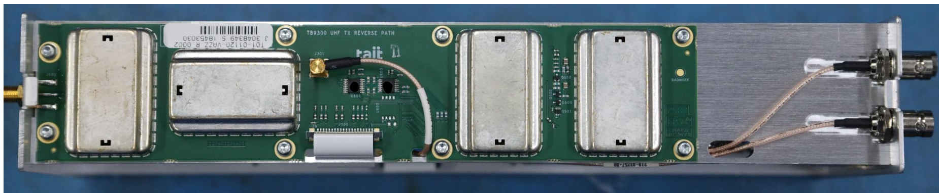
Photograph 14: Reciter Tx Reverse PCB – Top
