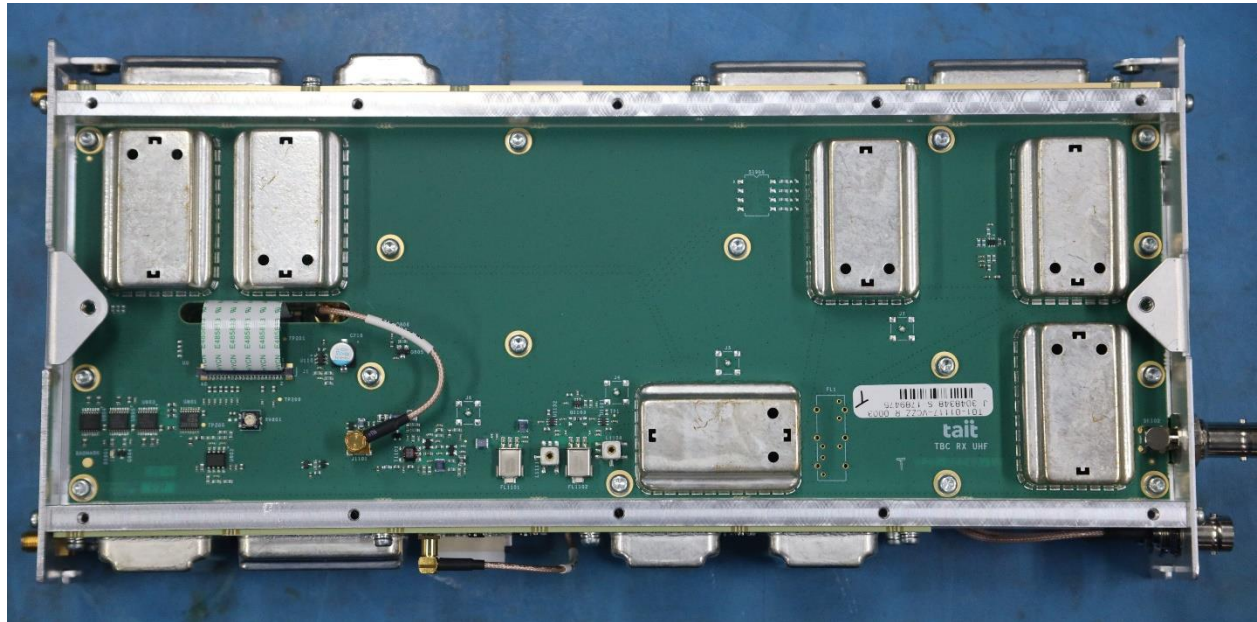
Photograph 8: Reciter Rx PCB – Top
