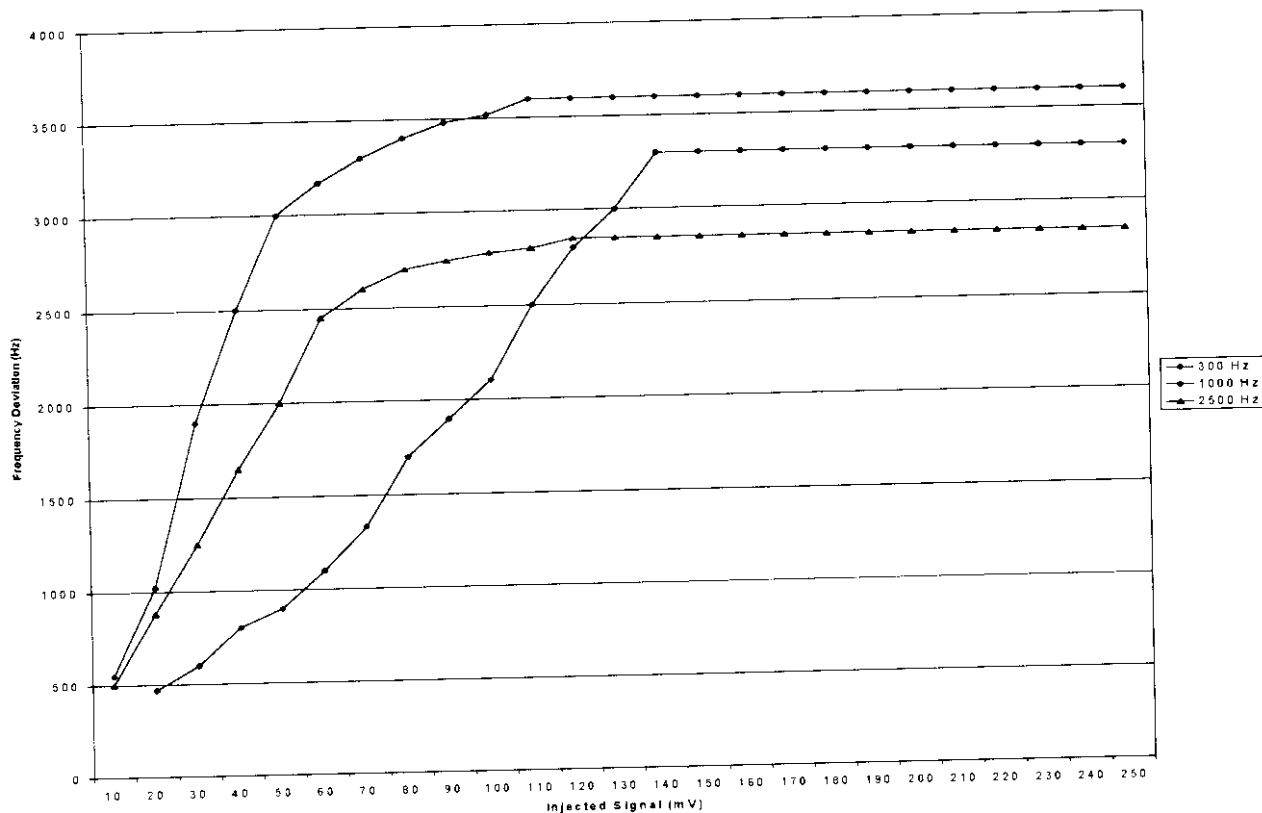
Modulation Limiting (Ch. 5 / 25 kHz channels)
