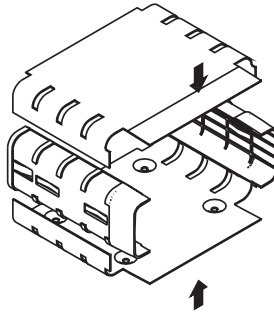
Figure 3: Cradle Reassembly
