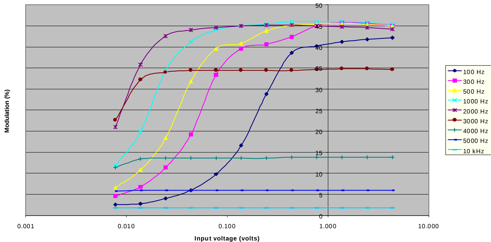
Modulation limiting characteristics (12.5 kHz)
