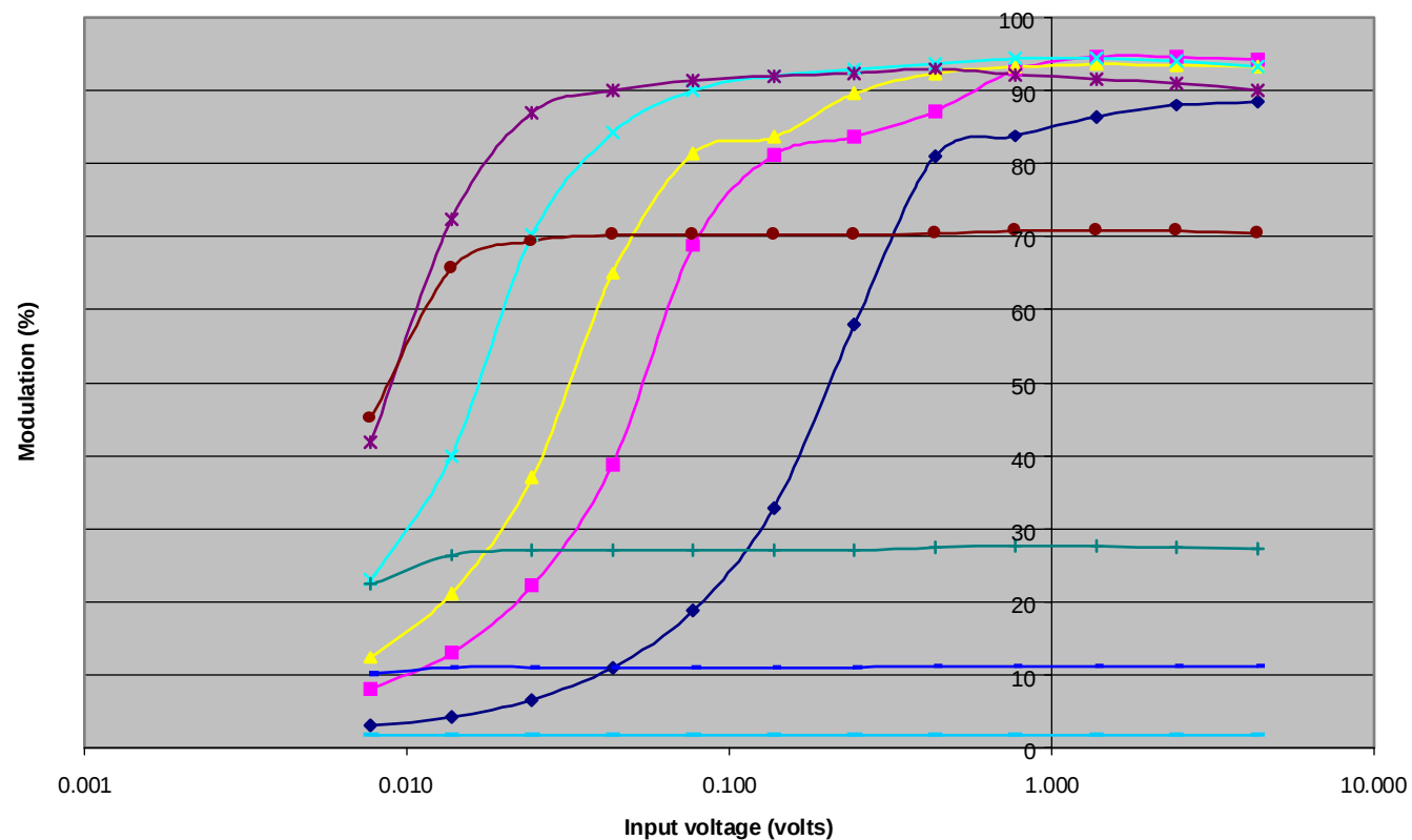
Modulation limiting characteristics (25 kHz)
