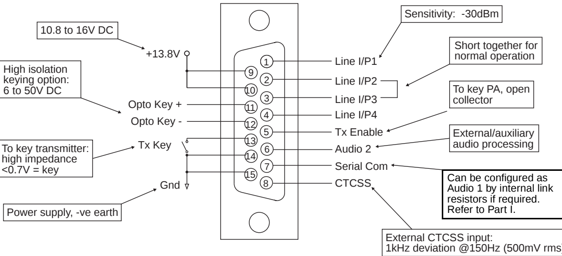
Figure 2.3 T836/837 D-Range 1 Wiring - Rear View
