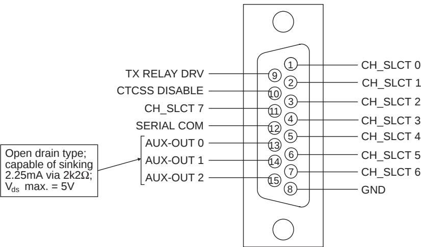
Figure 2.4 T836/837 D-Range 2 Wiring - Rear View (standard T800-03-0000 kit)
