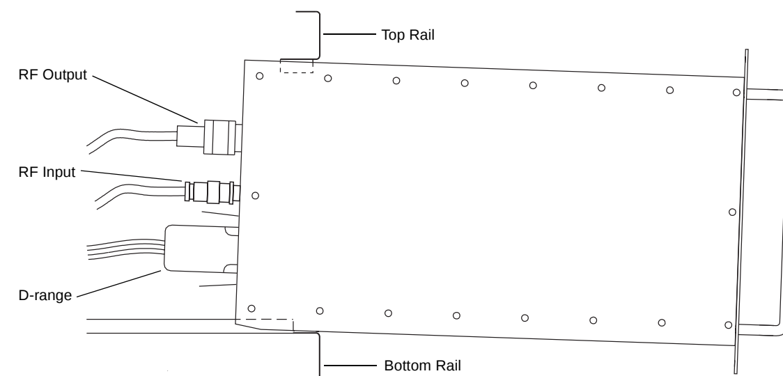
Figure 3.3 T858/859 PA In Latched Position
