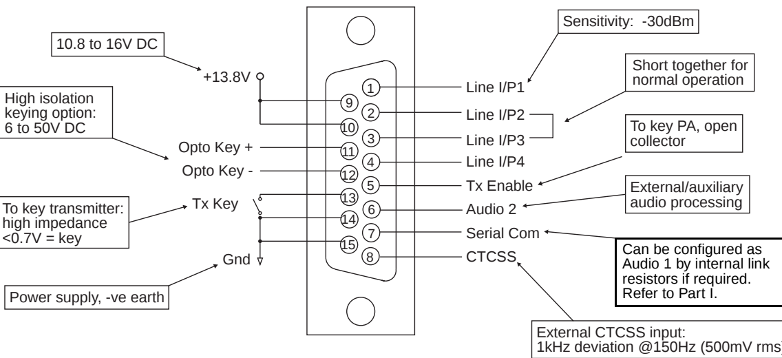
Figure 2.3 T856/857 D-Range 1 Wiring - Rear View
