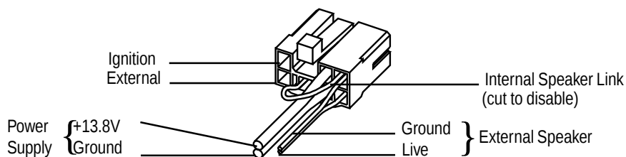
Figure 5: Power Connector Wiring
