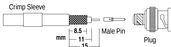
Figure 4: Antenna Connector Assembly
