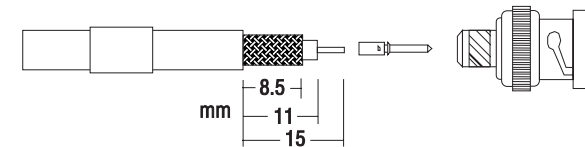
Figure 4 Antenna Connector Assembly
