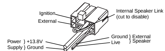
Figure 5 Power Connector Wiring
