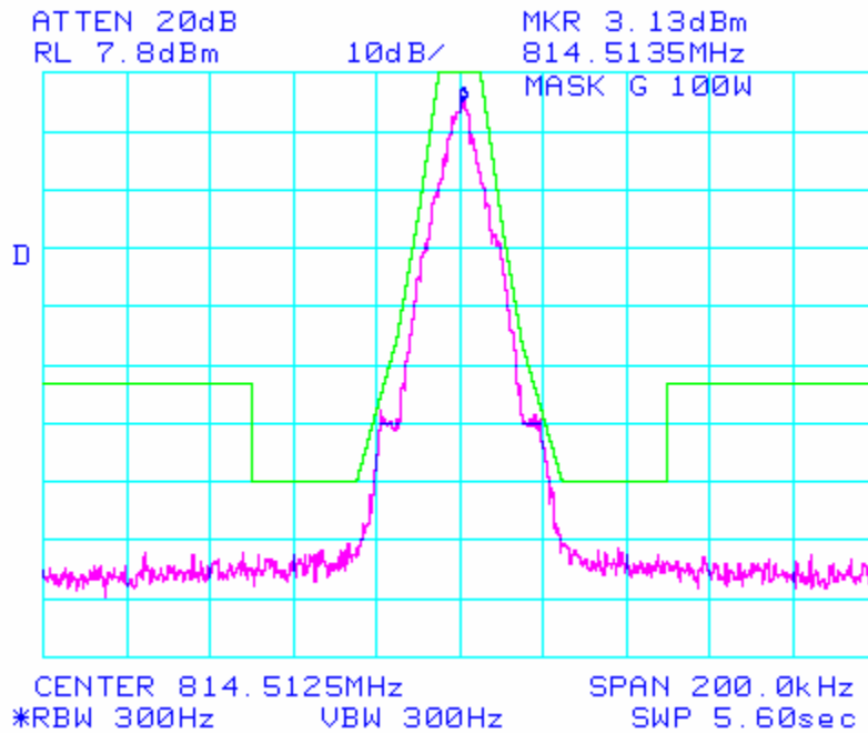
Plot 1b: MASK G, 13K0F1D, OUTPUT POWER: 5 Watts
