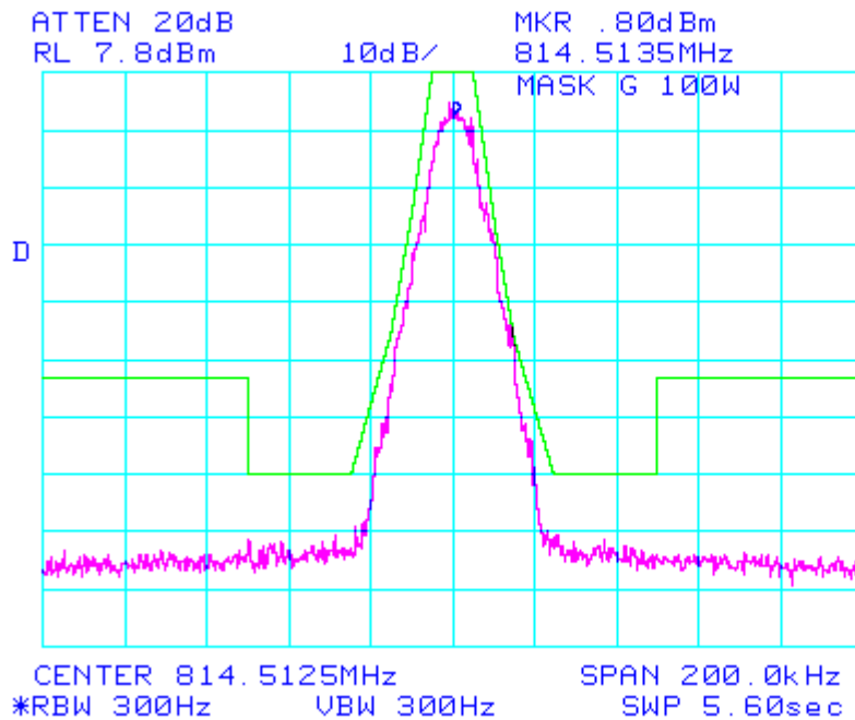
Plot 1b: MASK G, 14K0F1D, OUTPUT POWER: 5 Watts
