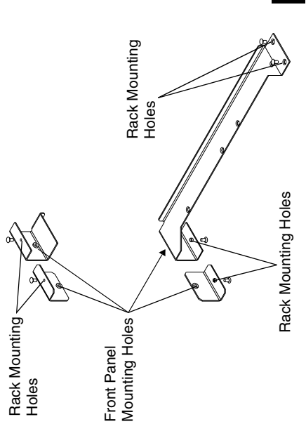
Figure 3.1 T800-45-0001 PA Guide Kit
