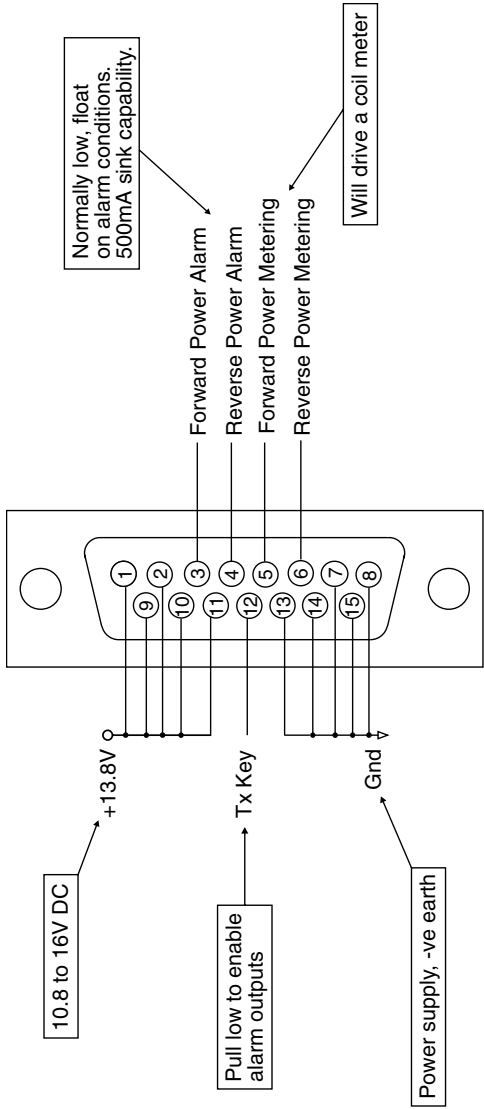
Figure 3.4 T858/859 D-Range Wiring - Rear View
