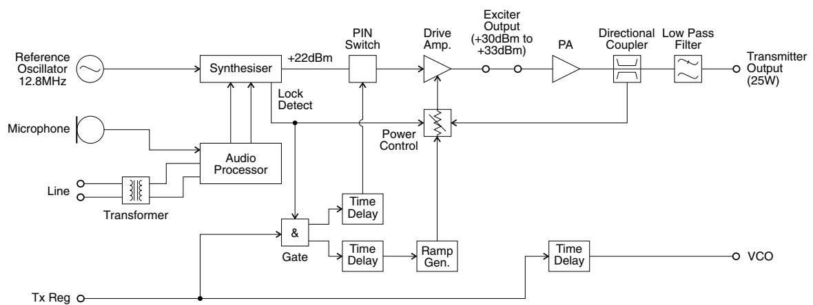
Figure 2.1 T854 High Level Block Diagram
