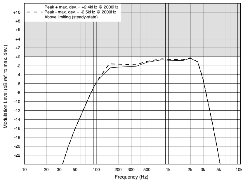
Figure 4.3 T854 Limiting Response
