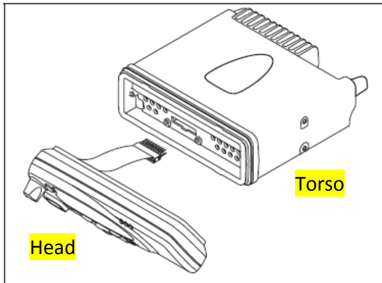
Figure 4.1 Mounting the control head
