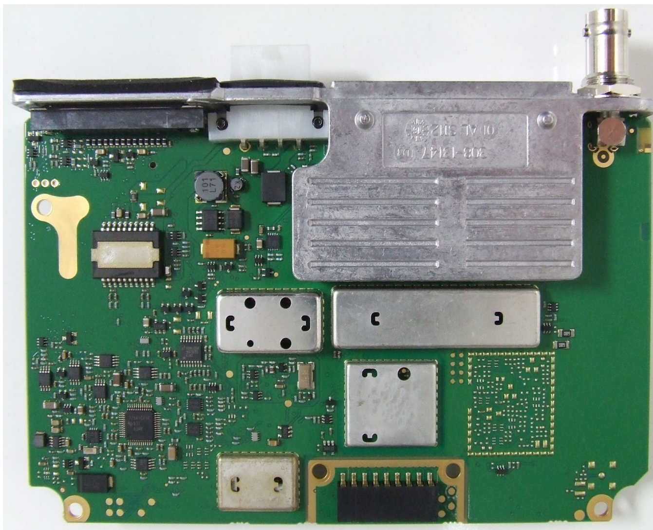
Photograph 04: Radio - Main PCB bottom with shields
