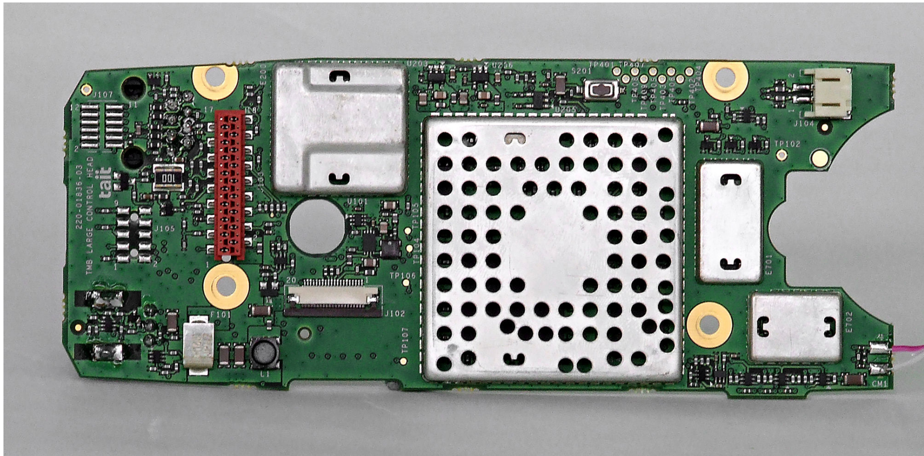
Photograph 09: Control Head - main PCB top with shields
