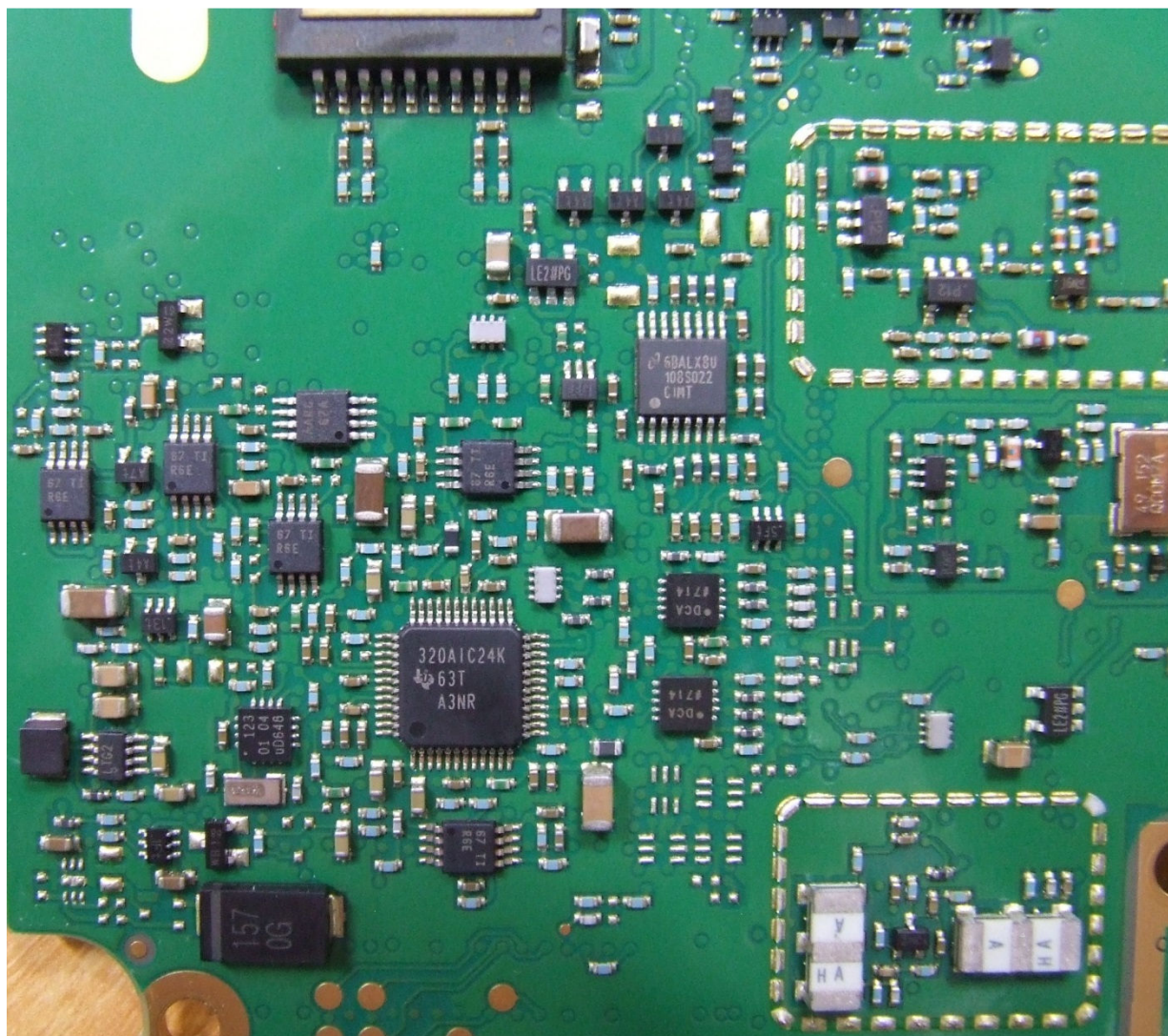
Photograph 06: Radio – Main PCB bottom without shields, close up of IC devices
