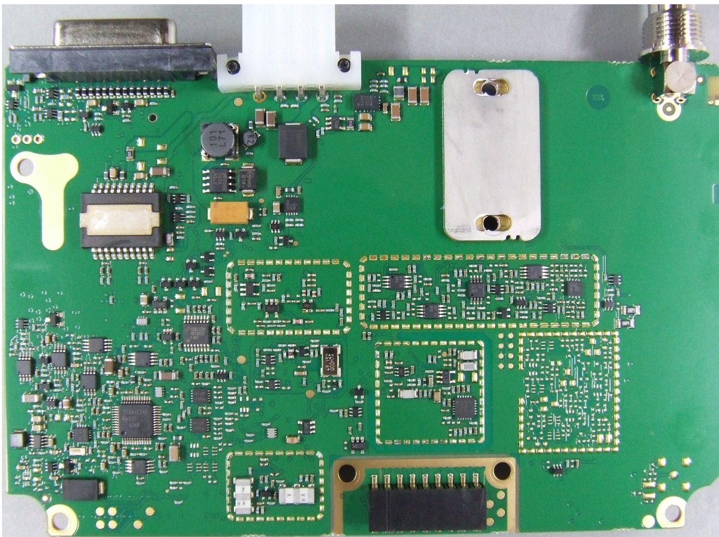
Photograph 05: Radio - Main PCB bottom without shields
