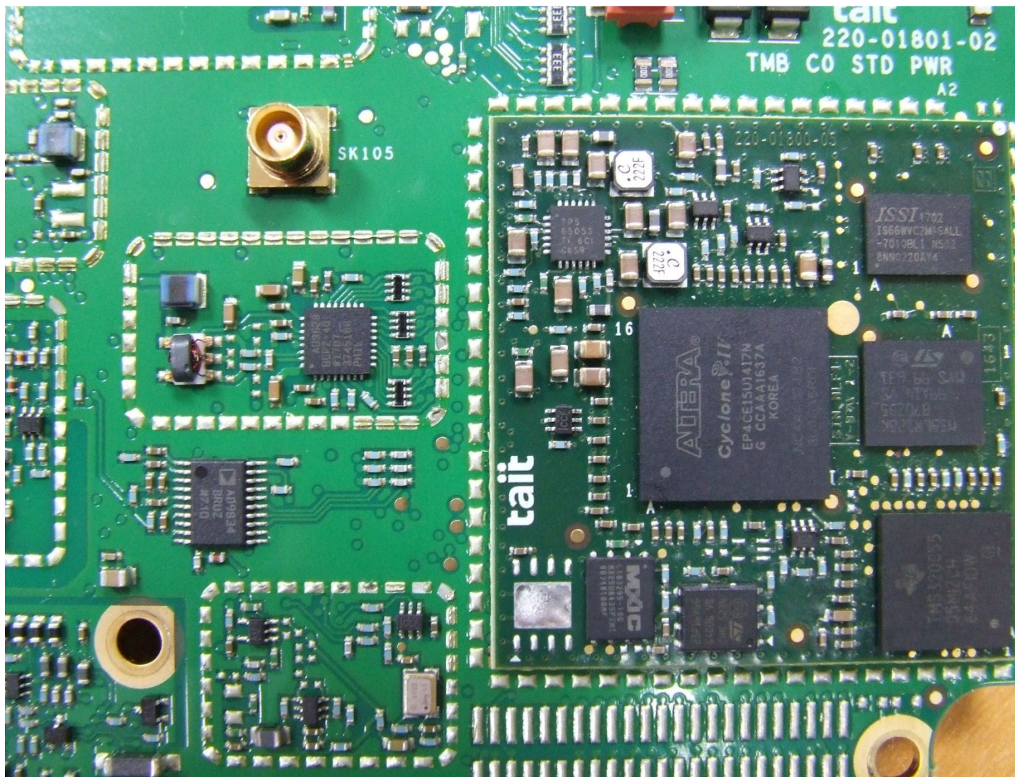
Photograph 03: Radio – Main PCB top without shields, close up of IC devices
