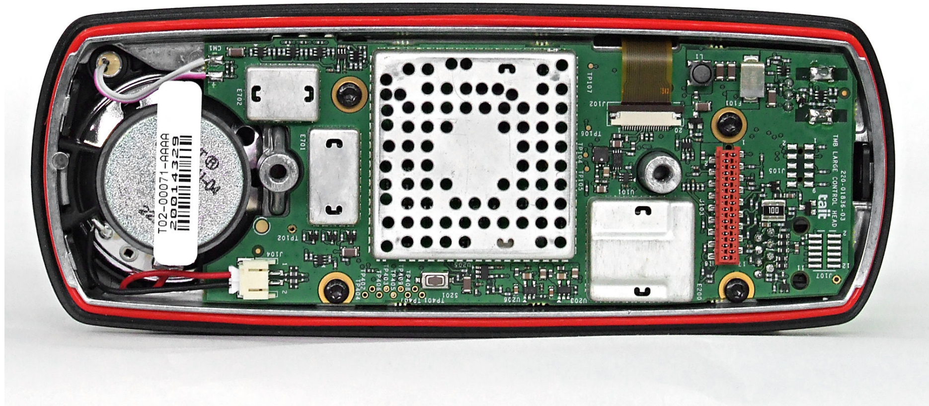
Photograph 07: Control Head - internal
