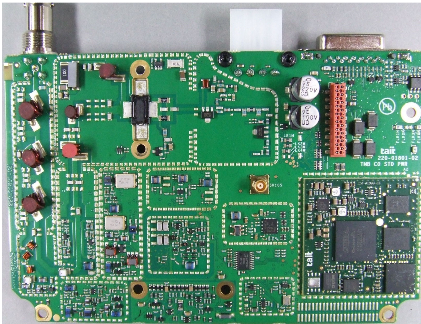
Photograph 02: Radio - Main PCB top without shields
