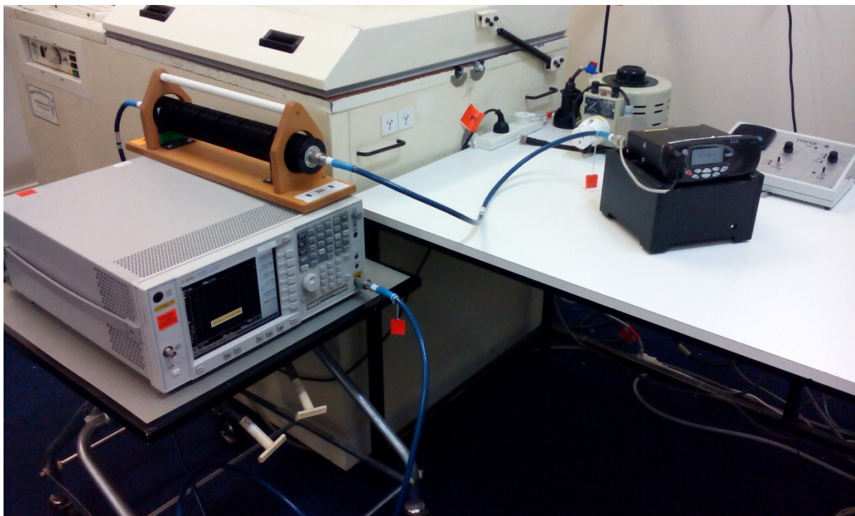
Photo: Conducted Emissions Test Setup
