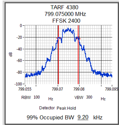
799.075 MHz, 30 W
