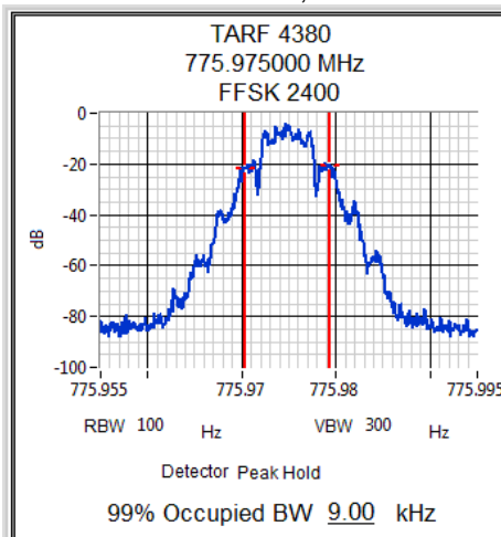
775.975 MHz, 30 W
