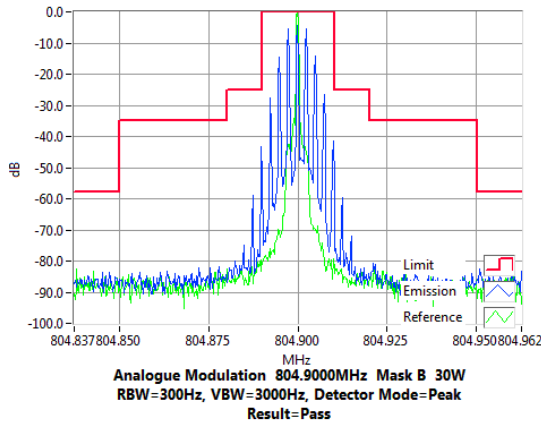
804.900 MHz, 20 kHz Channel Spacing, 30 W and 2 W Tx Power
