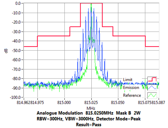
815.025 MHz, 20 kHz Channel Spacing, 35 W and 2 W Tx Power
