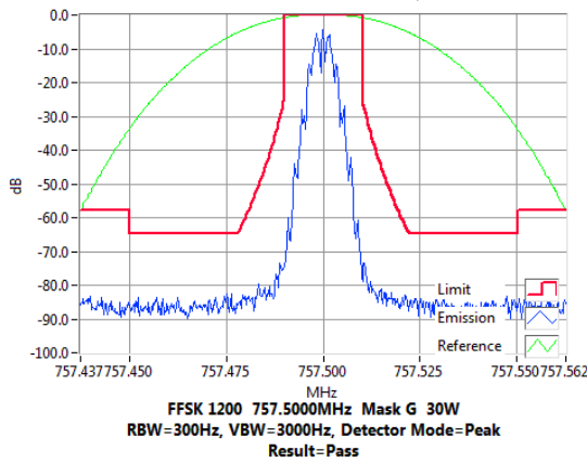
757.500 MHz, 20 kHz Channel Spacing, 30 W and 2 W Tx Power
