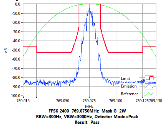
769.075 MHz, 20 kHz Channel Spacing, 30 W and 2 W Tx Power
