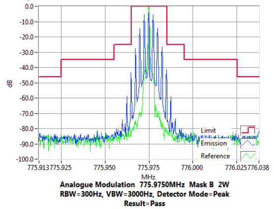
775.975 MHz, 20 kHz Channel Spacing, 30 W and 2 W Tx Power
