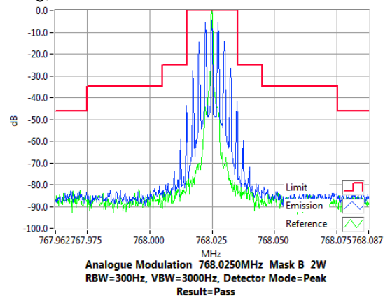
768.025 MHz, 20 kHz Channel Spacing, 30 W and 2 W Tx Power
