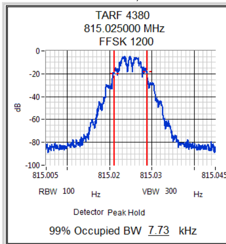
815.025 MHz, 35 W
