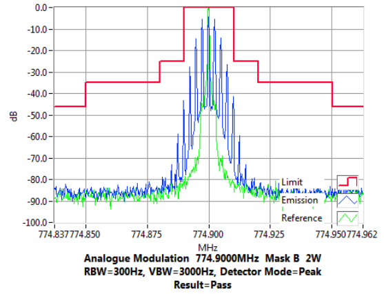
774.900 MHz, 20 kHz Channel Spacing, 30 W and 2 W Tx Power
