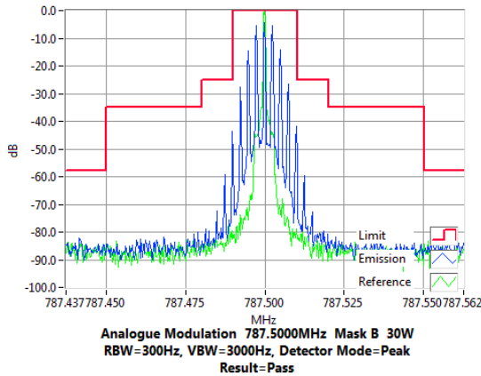
787.500 MHz, 20 kHz Channel Spacing, 30 W and 2 W Tx Power
