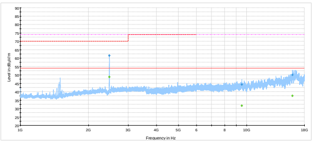
Figure 8.2-10: Spurious emissions above 1 GHz, high channel 802.11 n HT 40 WLP2458NGP
