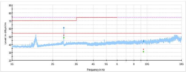
Figure 8.2-8: Spurious emissions above 1 GHz, low channel 802.11 n HT 40 WLP2458NGP
