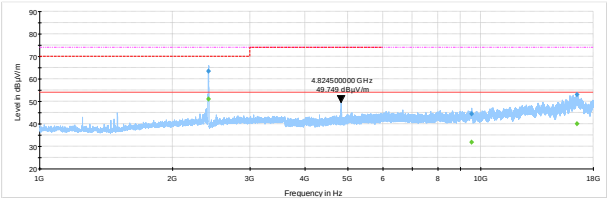
Figure 8.2-2: Spurious emissions above 1 GHz, low channel 802.11 b WLP2458NGP
