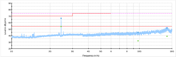
Figure 8.2-4: Spurious emissions above 1 GHz, high channel 802.11 b WLP2458NGP
