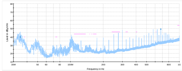
Figure 8.2-5: Spurious emissions below 1 GHz, mid channel 802.11 b WLP2458NGP
