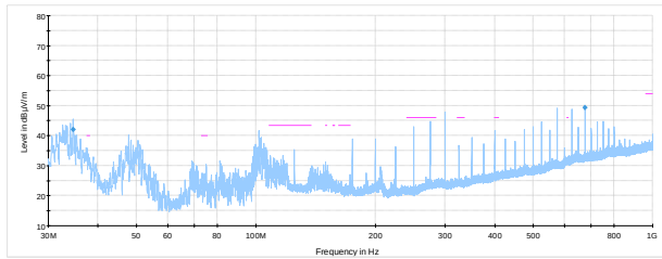
Figure 8.2-3: Spurious emissions below 1 GHz, high channel 802.11 b WLP2458NGP
