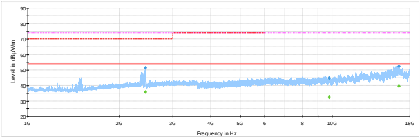
Figure 8.2-18: Spurious emissions above 1 GHz, low channel 802.11 n GPSD
