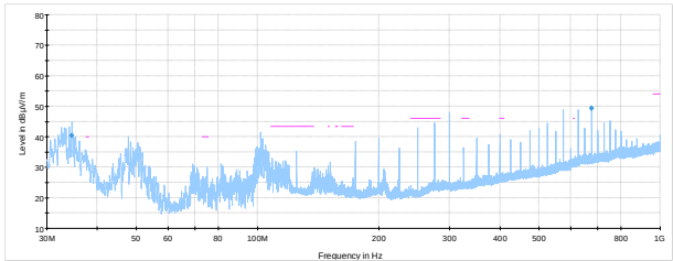
Figure 8.2-7: Spurious emissions below 1 GHz, low channel 802.11 n HT 40 WLP2458NGP
