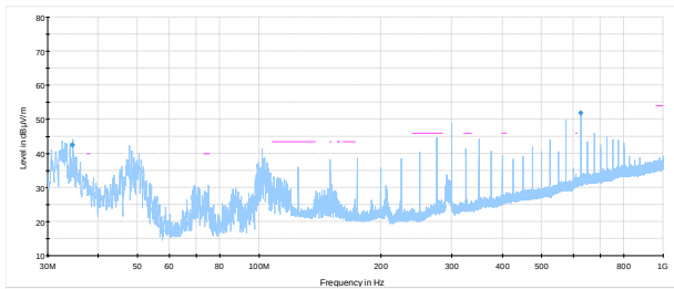
Figure 8.2-15: Spurious emissions below 1 GHz, mid channel 802.11 b GPSD
