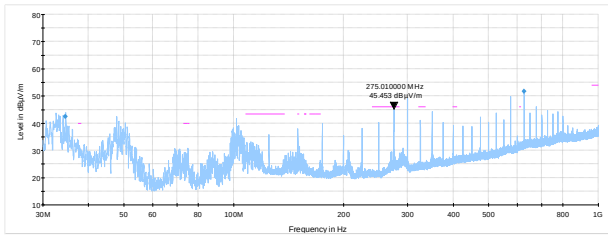
Figure 8.2-17: Spurious emissions below 1 GHz, low channel 802.11 n GPSD
