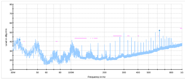
Figure 8.2-13: Spurious emissions below 1 GHz, high channel 802.11 b GPSD
