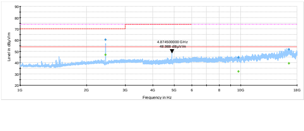
Figure 8.2-16: Spurious emissions above 1 GHz, mid channel 802.11 b GPSD
