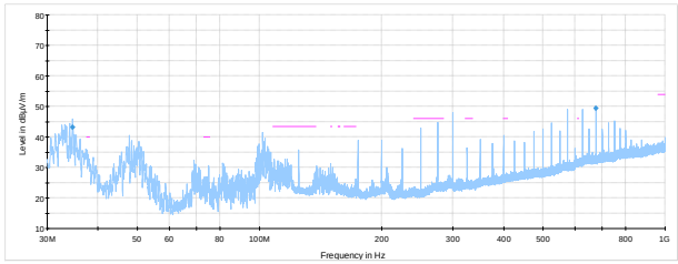
Figure 8.2-9: Spurious emissions below 1 GHz, high channel 802.11 n HT 40 WLP2458NGP
