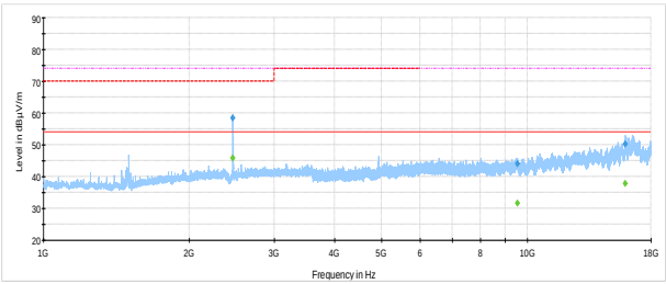
Figure 8.2-14: Spurious emissions above 1 GHz, high channel 802.11 b GPSD
