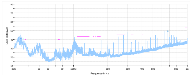
Figure 8.2-1: Spurious emissions below 1 GHz, low channel 802.11 b WLP2458NGP
