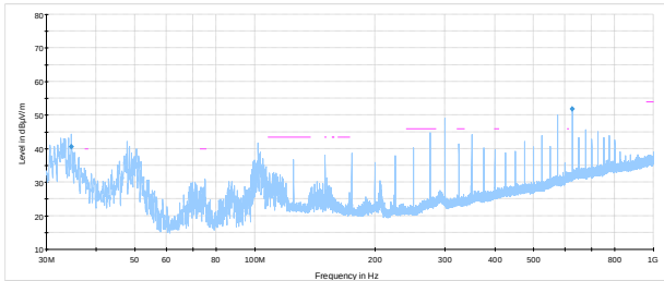
Figure 8.2-11: Spurious emissions below 1 GHz, low channel 802.11 b GPSD
