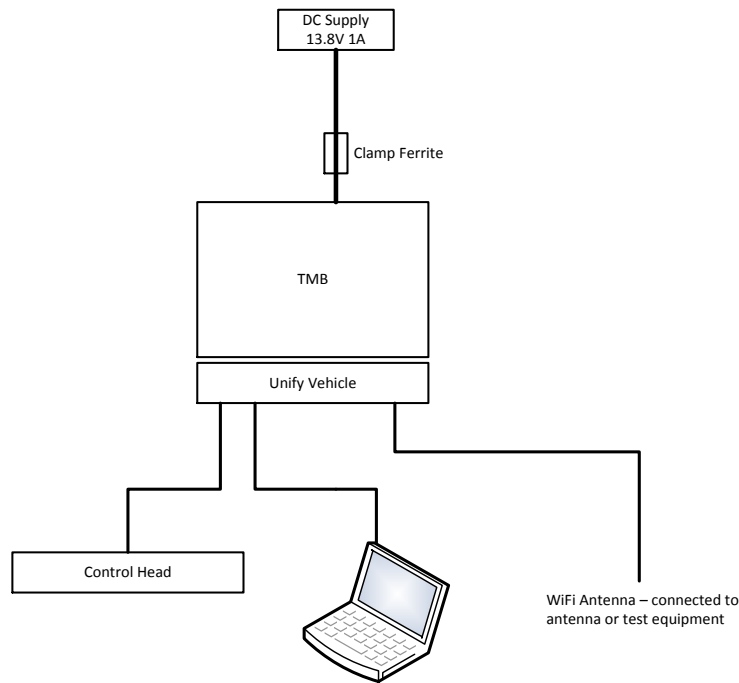
Figure 3.6-1: Setup diagram
