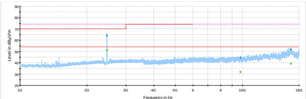
Figure 8.2-2: Spurious emissions above 1 GHz, low channel 802.11 b WLP2458NGP
