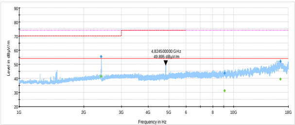
Figure 8.2-12: Spurious emissions above 1 GHz, low channel 802.11 b GPSD
