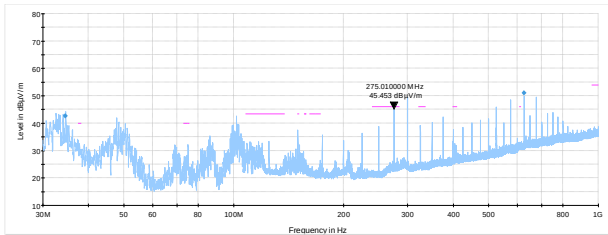
Figure 8.2-19: Spurious emissions below 1 GHz, high channel 802.11 n GPSD
