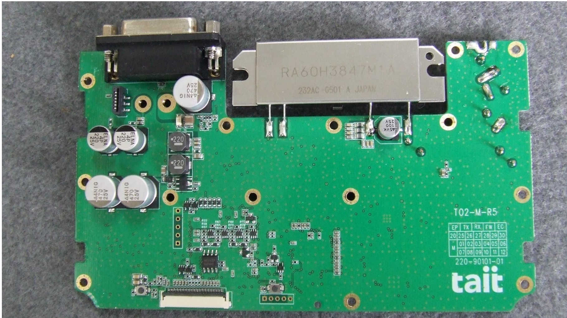
Photograph 1: Radio Main PCB 220-90101-01 top
