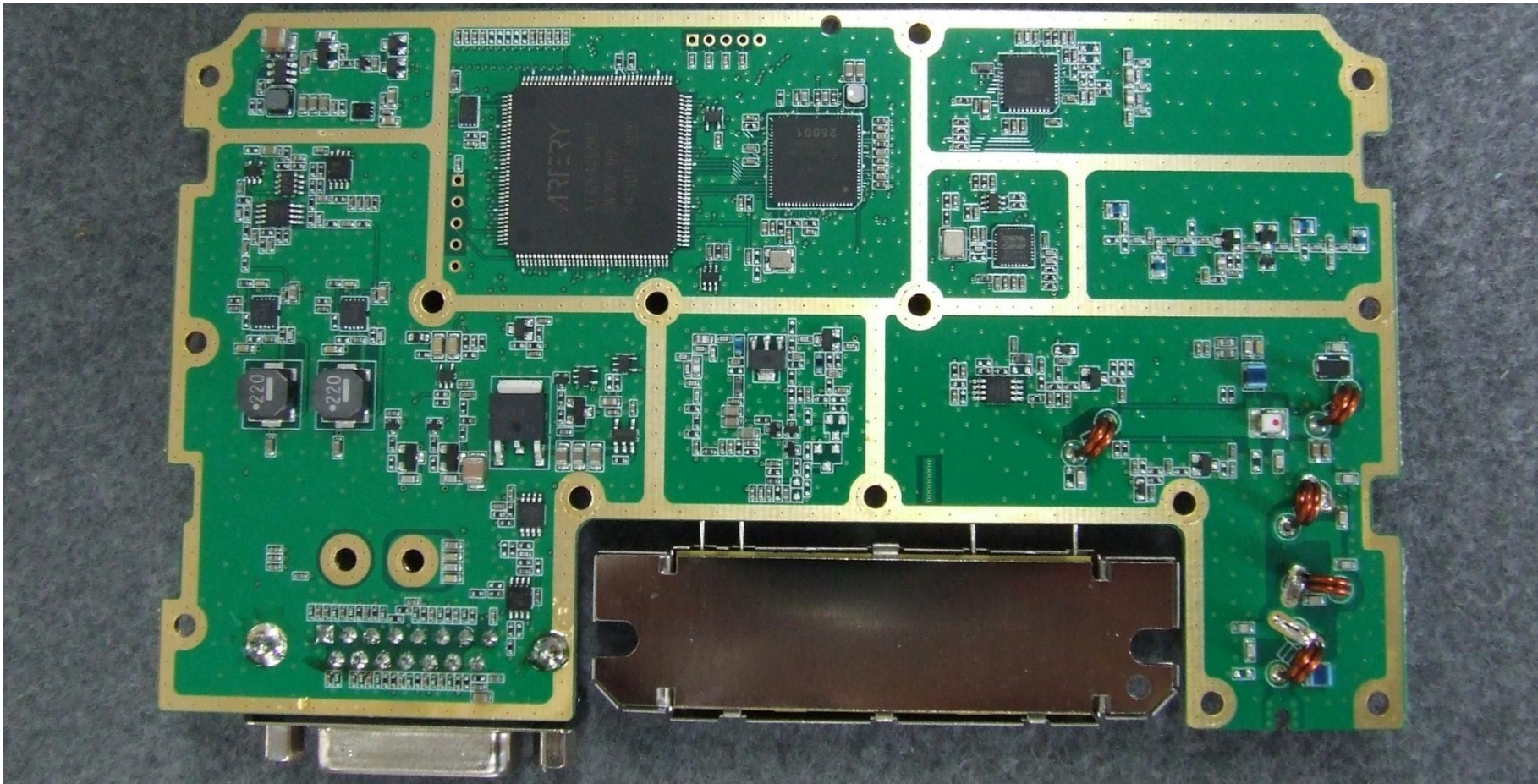
Photograph 2: Radio Main PCB 220-90101-01 bottom
