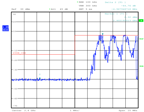
Figure 8.6-4: Conducted spurious emissions at the lower band edge for \pi/4 -DQPSK modulation, hopping on
