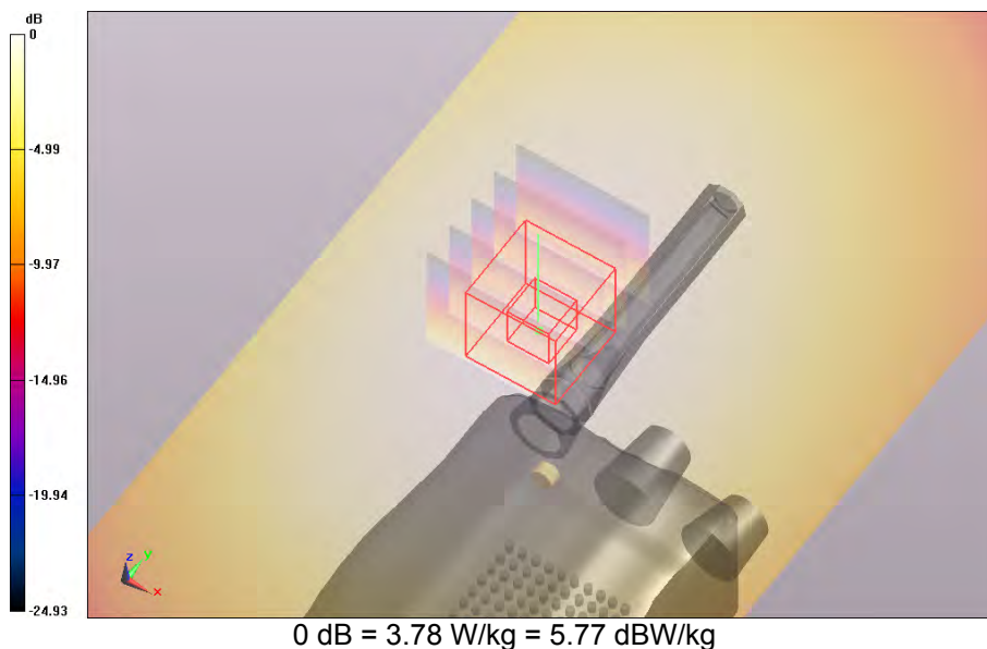
SAR Measurement Plot 60
