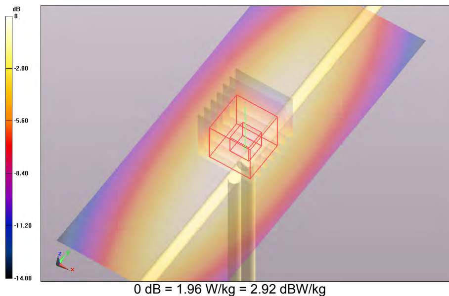
SAR Measurement Plot 42
