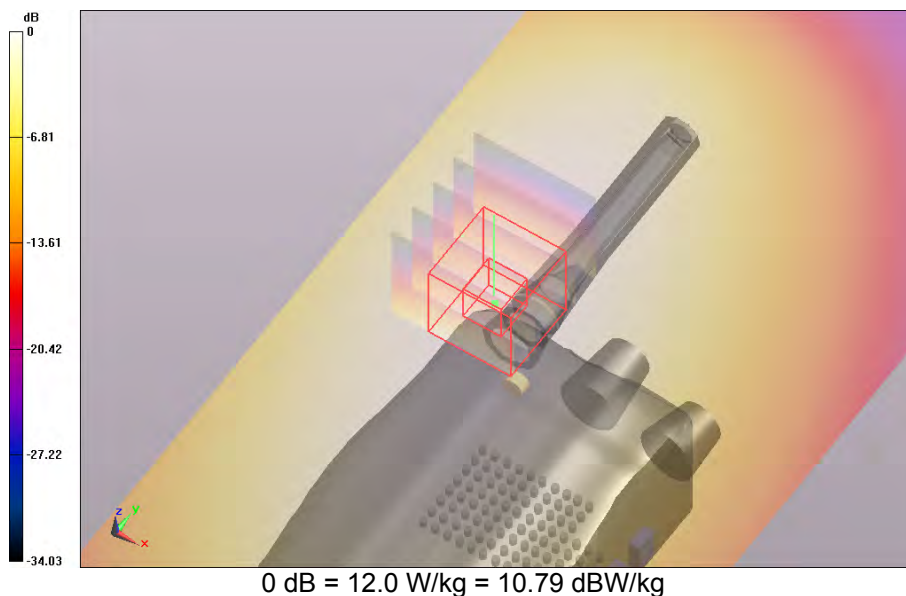
SAR Measurement Plot 58
