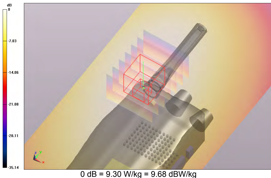
SAR Measurement Plot 50
