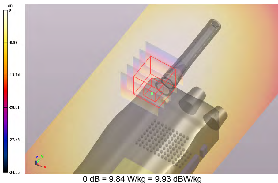
SAR Measurement Plot 63
