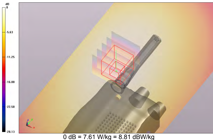
SAR Measurement Plot 59
