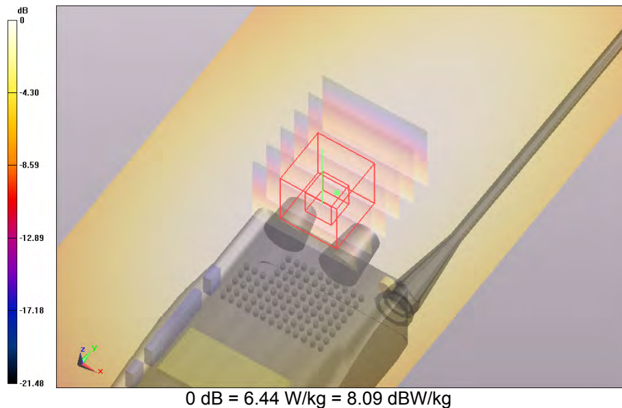
SAR Measurement Plot 83
