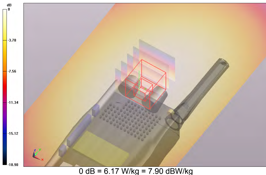
SAR Measurement Plot 89
