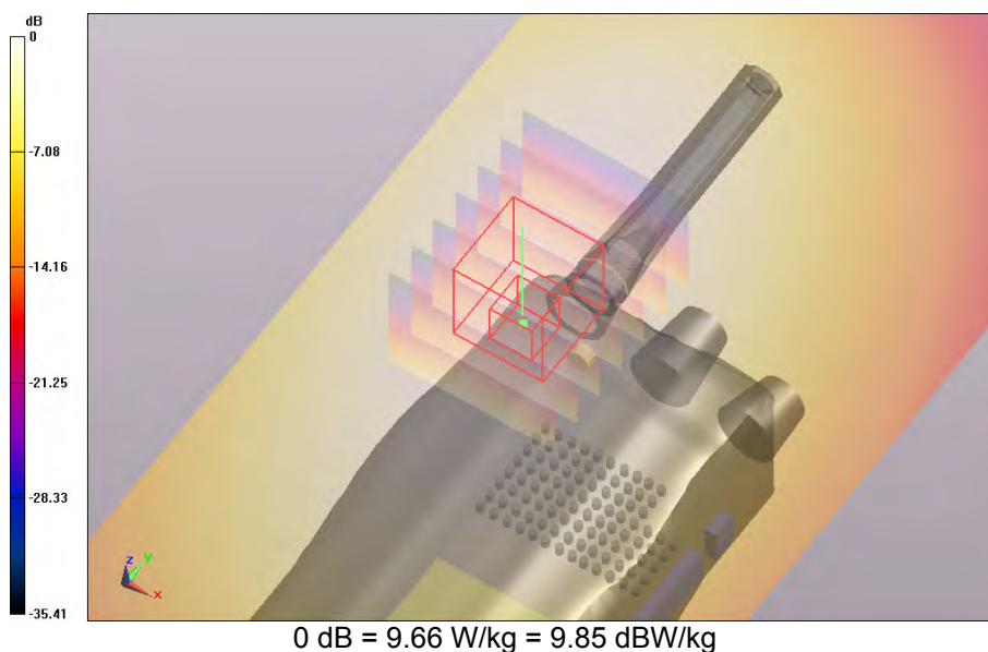
SAR Measurement Plot 62
