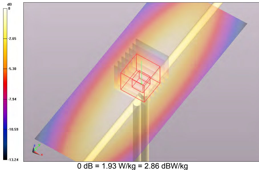
SAR Measurement Plot 43
