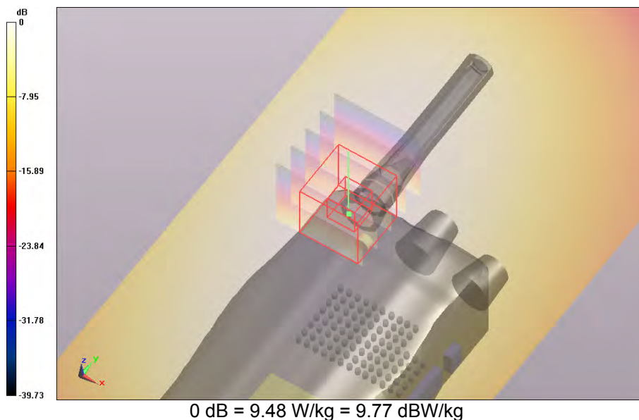
SAR Measurement Plot 73
