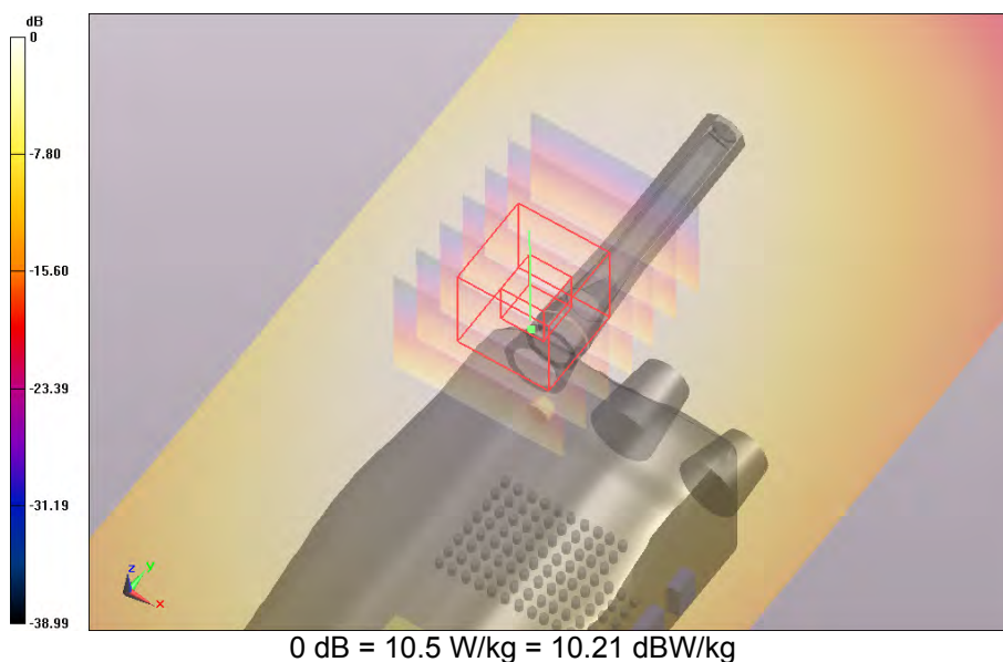
SAR Measurement Plot 49
