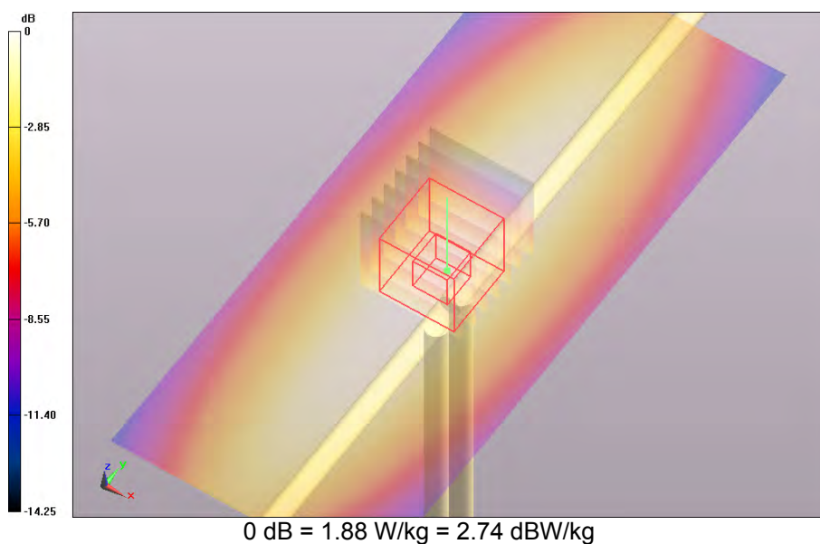
SAR Measurement Plot 44
