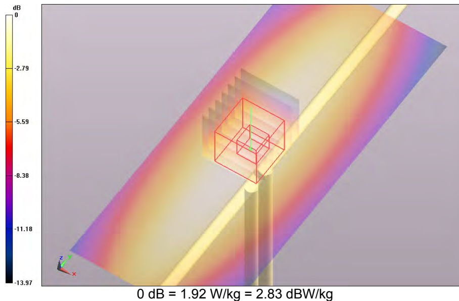
SAR Measurement Plot 77
