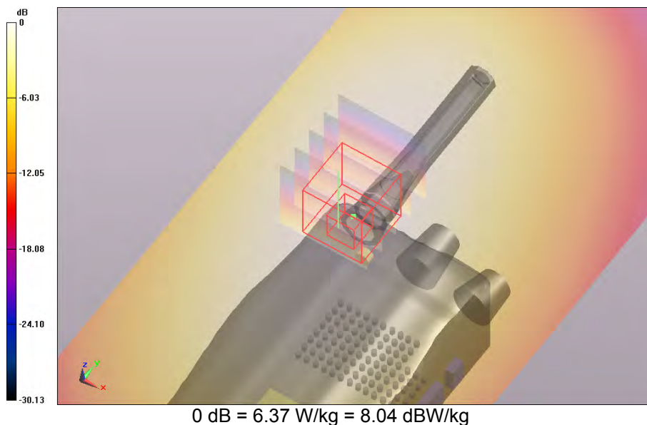
SAR Measurement Plot 52
