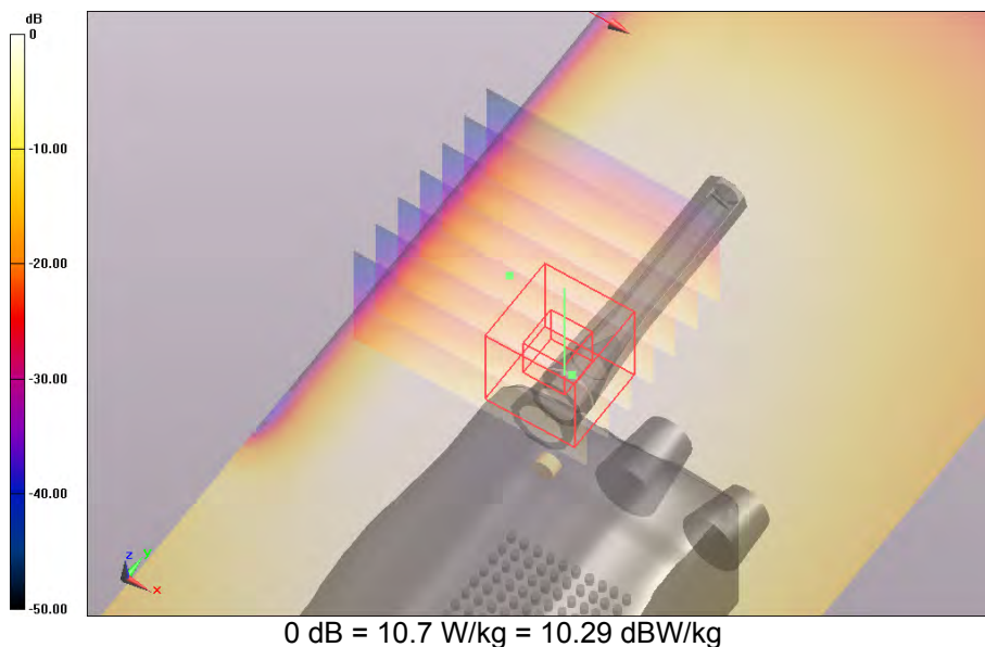
SAR Measurement Plot 75
