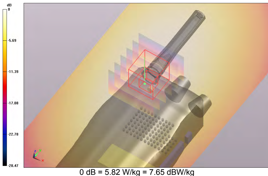
SAR Measurement Plot 68
