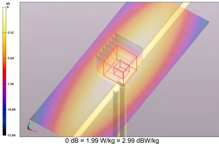
SAR Measurement Plot 87
