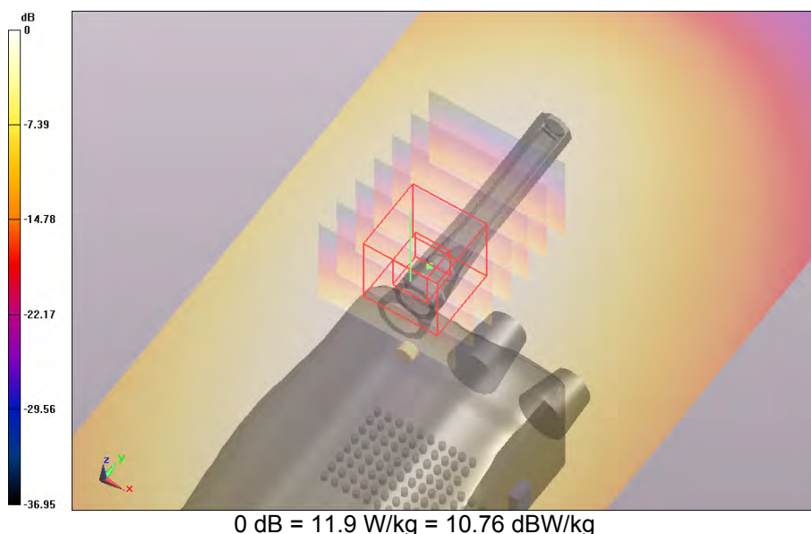
SAR Measurement Plot 76
