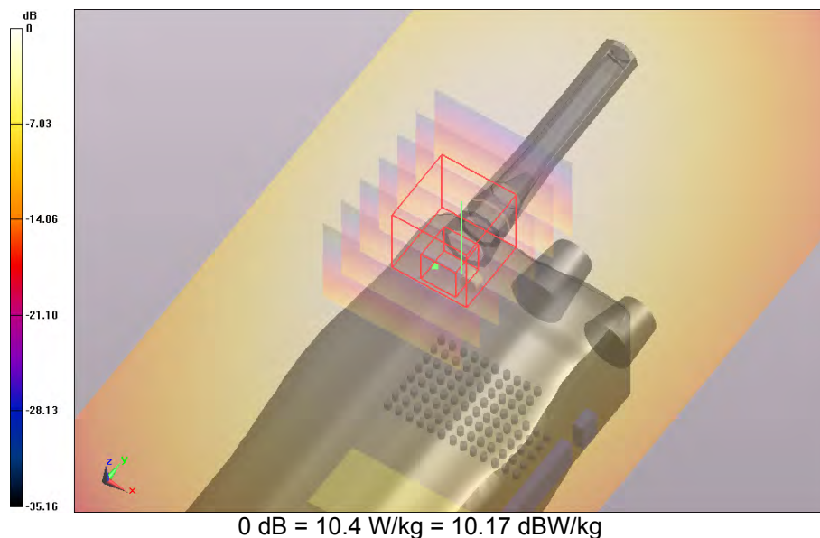
SAR Measurement Plot 65
