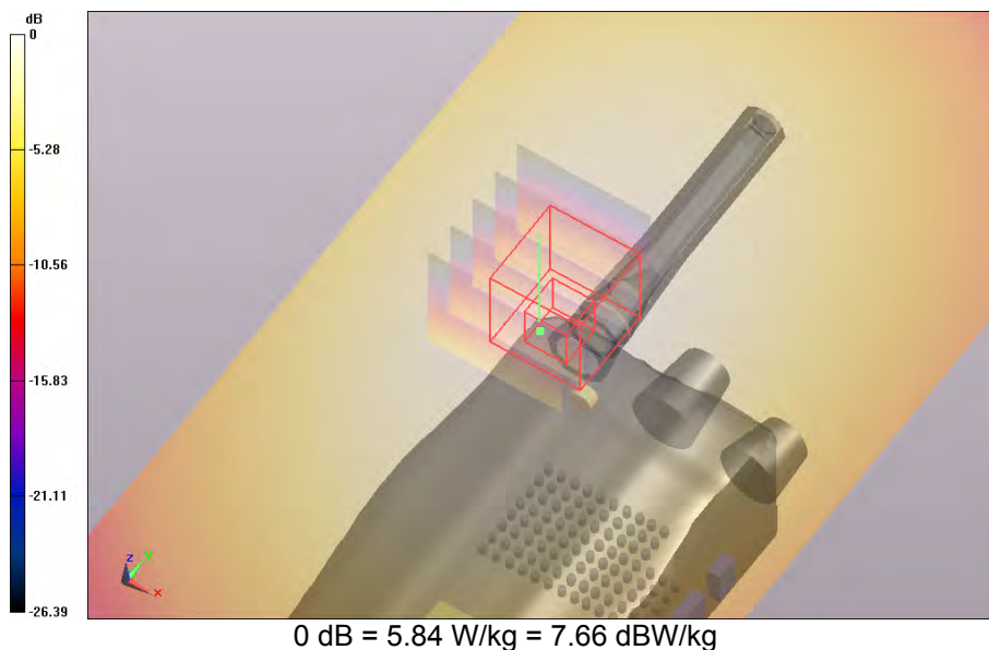
SAR Measurement Plot 69
