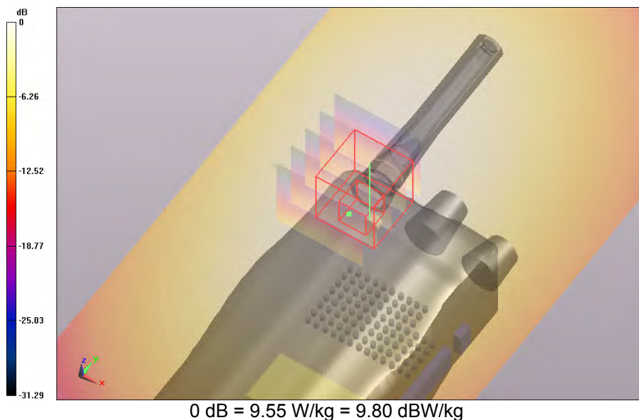
SAR Measurement Plot 67
