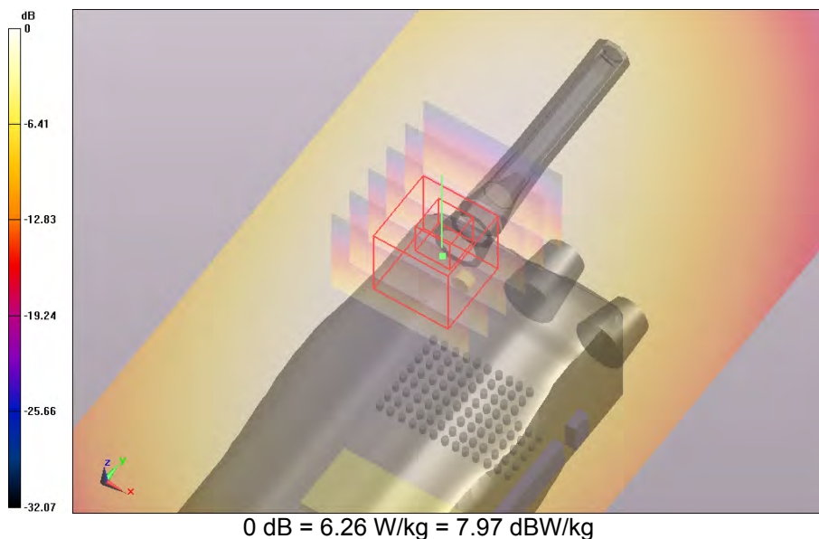
SAR Measurement Plot 56
