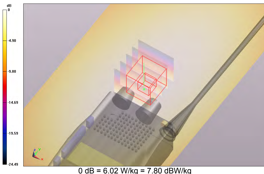
SAR Measurement Plot 85
