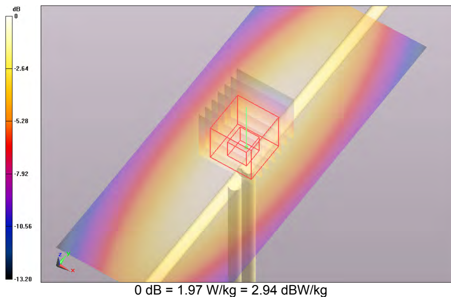
SAR Measurement Plot 78
