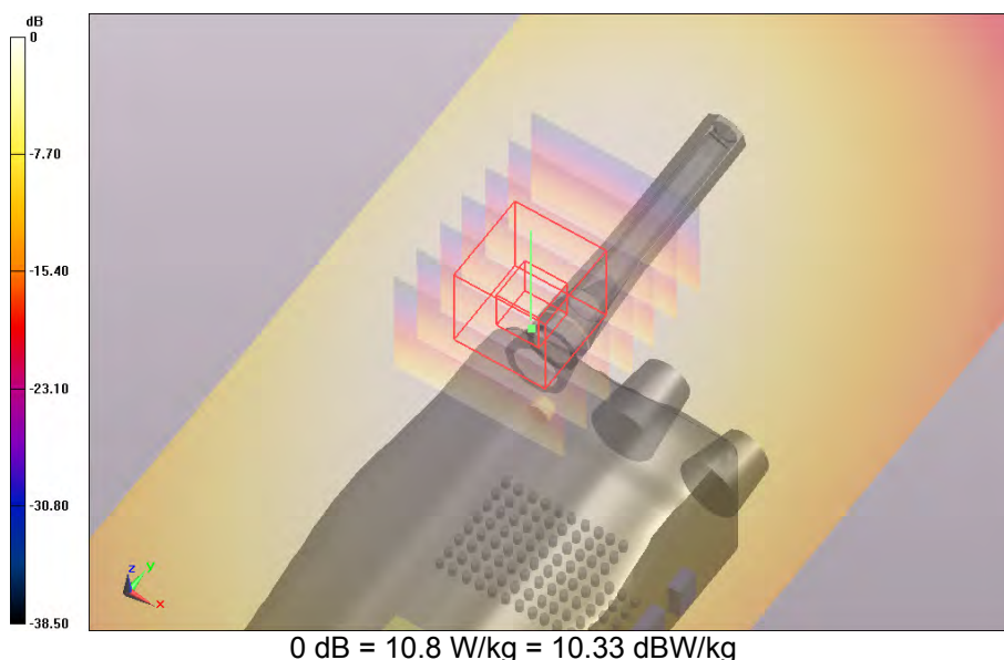
SAR Measurement Plot 61
