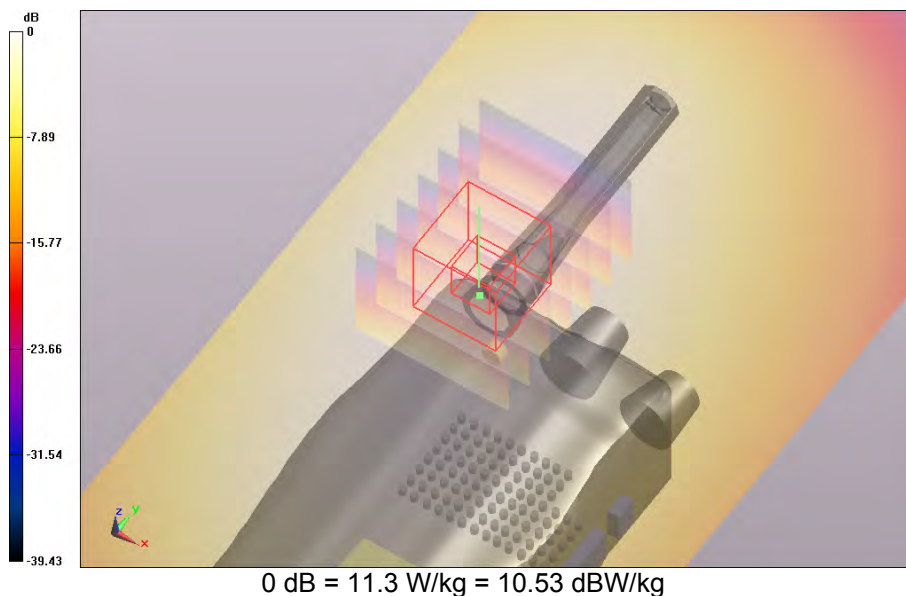
SAR Measurement Plot 53
