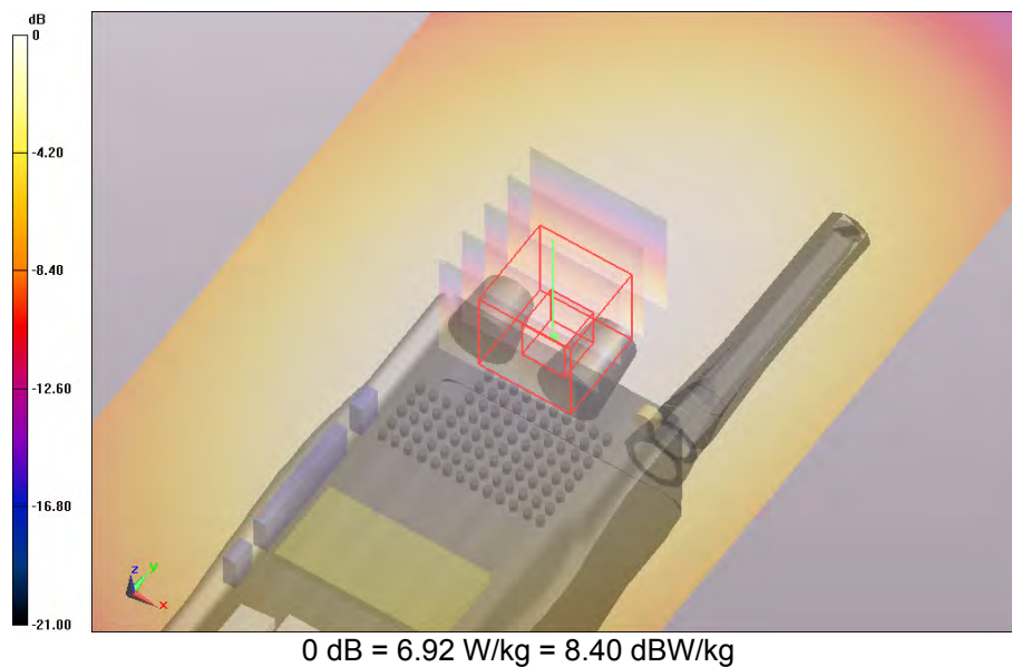
SAR Measurement Plot 88
