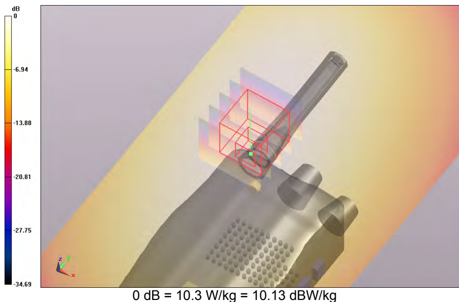
SAR Measurement Plot 51
