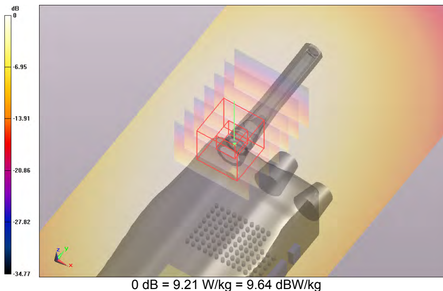
SAR Measurement Plot 72
