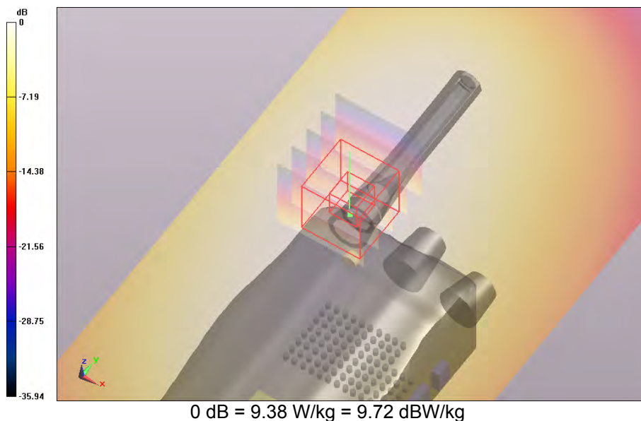
SAR Measurement Plot 55
