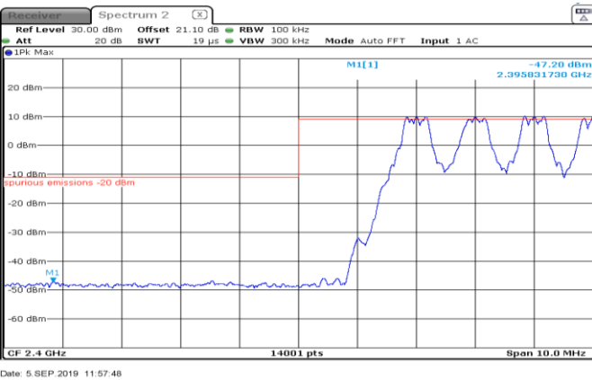
Figure 8.6-6: Conducted spurious emissions at the lower band edge for 8DPSK modulation, hopping on
