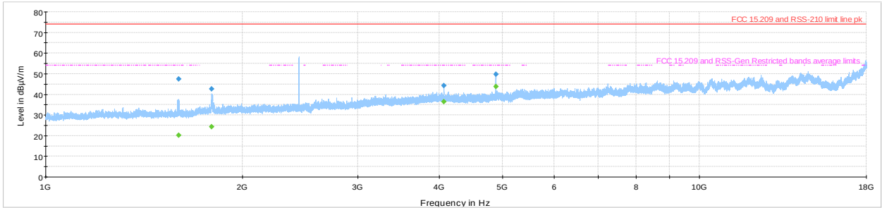
Figure 8.6-30: Radiated spurious emissions within 1-18 GHz, low channel
