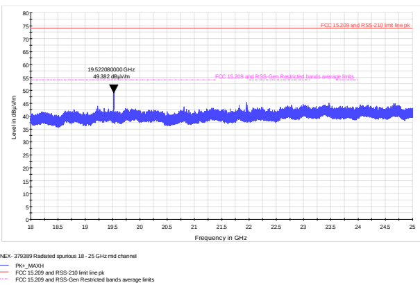
Figure 8.6-34: Radiated spurious emissions above 18 GHz, mid channel
