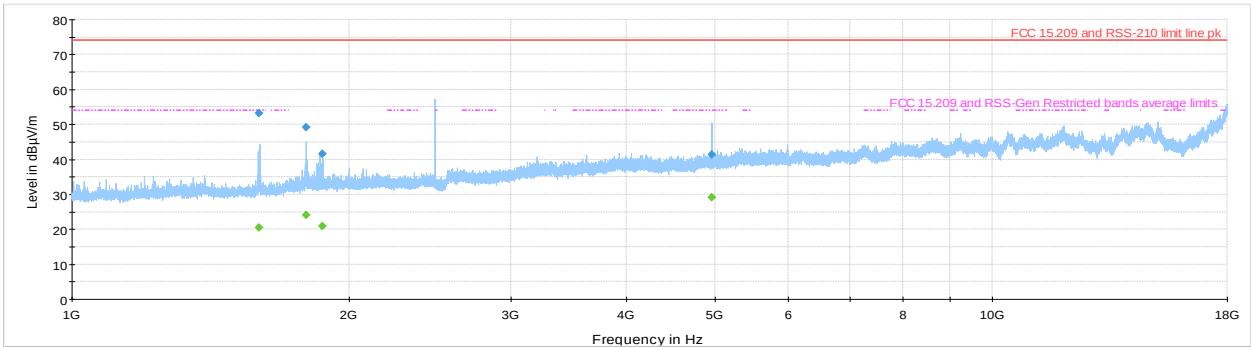
Figure 8.6-31: Radiated spurious emissions within 1-18 GHz, mid channel
