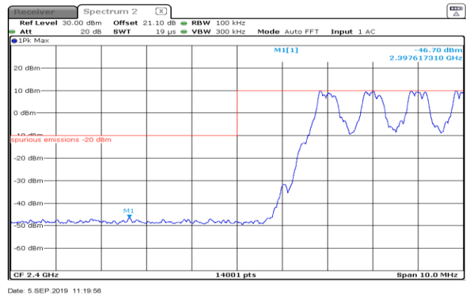
Figure 8.6-2: Conducted spurious emissions at the lower band edge for GFSK modulation, hopping on
