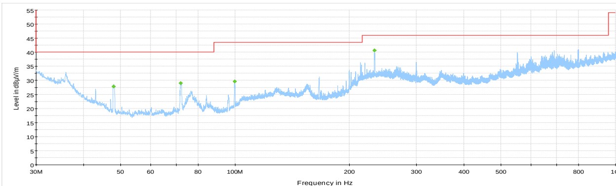
Figure 8.6-28: Radiated spurious emissions below 1 GHz, mid channel
