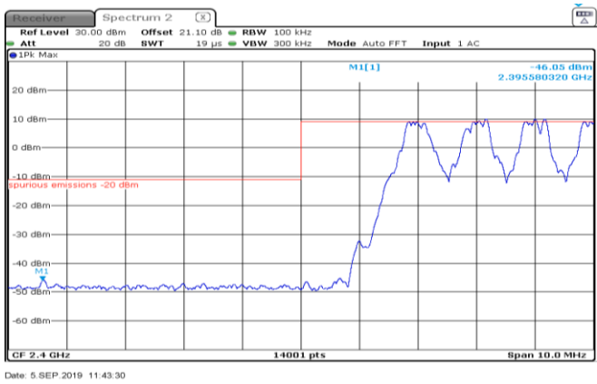
Figure 8.6-4: Conducted spurious emissions at the lower band edge for \pi/4 -DQPSK modulation, hopping on
