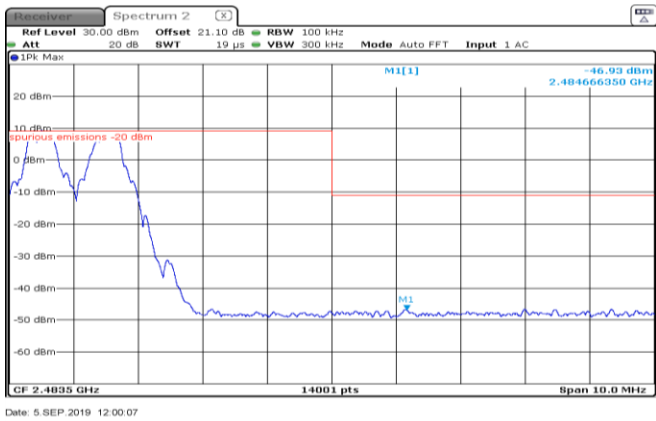
Figure 8.6-14: Conducted spurious emissions at the upper band edge for 8DPSK modulation, hopping on
