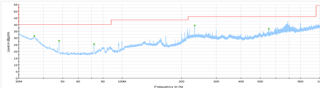
Figure 8.6-27: Radiated spurious emissions below 1 GHz, low channel
