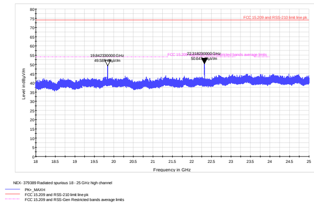
Figure 8.6-35: Radiated spurious emissions above 18 GHz, high channel
