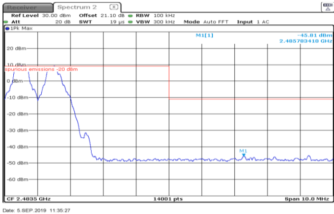
Figure 8.6-12: Conducted spurious emissions at the upper band edge for \pi/4 -DQPSK modulation, hopping on
