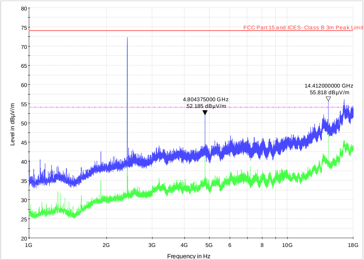
Figure 8.2-2: Radiated spurious emissions above 1 GHz, sample plot
