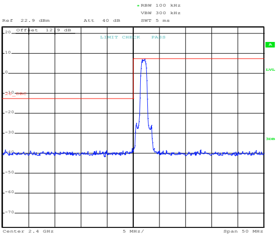
Figure 8.2-4: Radiated spurious band edge emission at 2.4 GHz, GFSK modulation, 20 dBc limit
