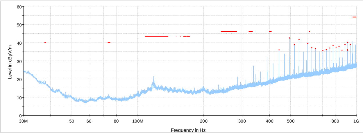
Figure 8.2-1: Radiated spurious emissions below 1 GHz, sample plot
