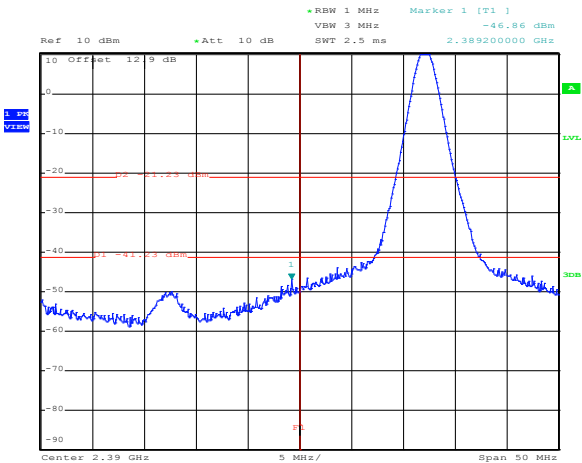
Figure 8.2-3: Radiated spurious band edge emission at 2.39 GHz, GFSK modulation, 15.209 limits
