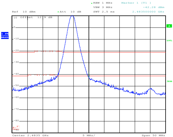
Figure 8.2-9: Radiated spurious band edge emission at 2.4835 GHz, QPSK modulation, 15.209 limits
