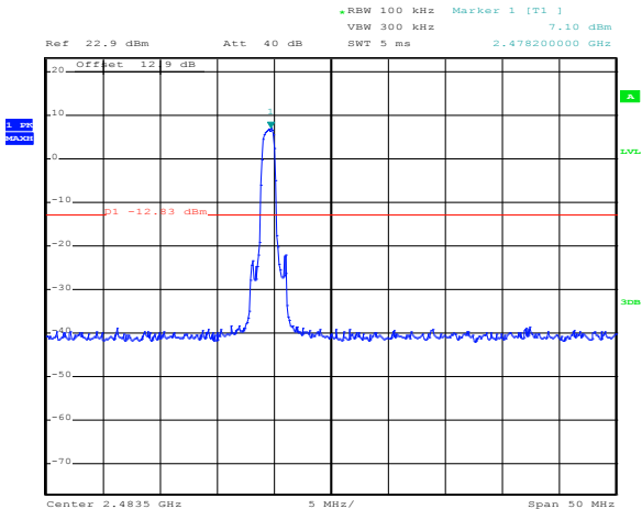
Figure 8.2-10: Radiated spurious band edge emission at 2.4835 GHz, QPSK modulation, 20 dBc limit
