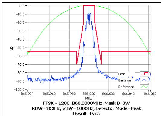
866.00000 MHz 3 W
