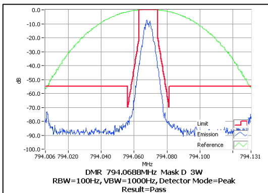
794.06875 MHz 3 W
