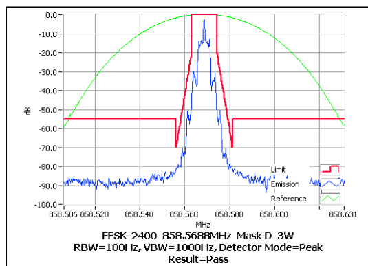
858.56875 MHz 3 W
