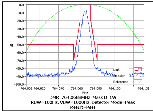
764.06875 MHz 1 W
