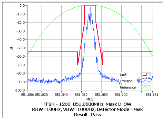
851.06875 MHz 3 W
