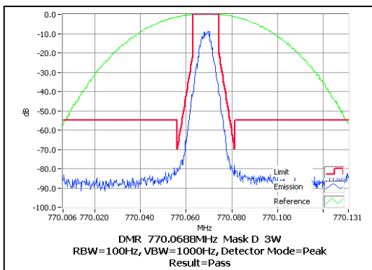
770.06875 MHz 3 W
