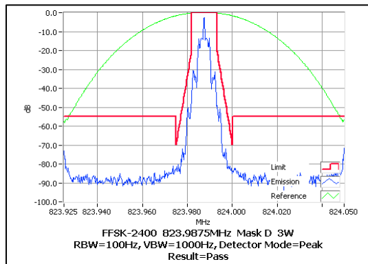
823.98750 MHz 3 W
