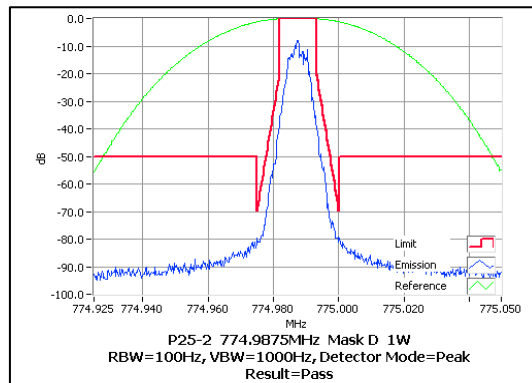
774.98750 MHz 1 W
