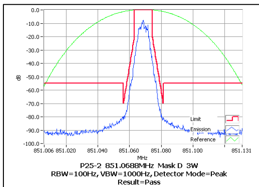
851.06875 MHz 3 W
