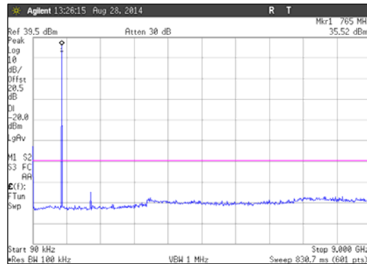
770.06875 MHz
