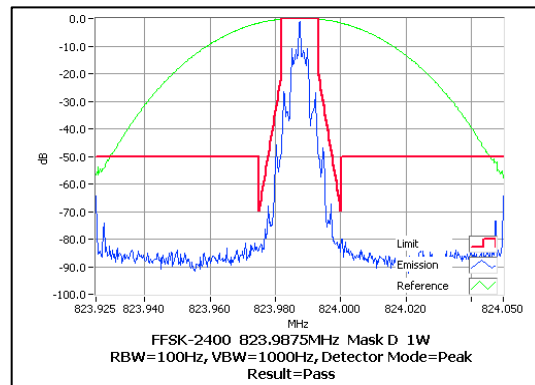
823.98750 MHz 1 W
