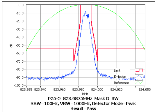
823.98750 MHz 3 W
