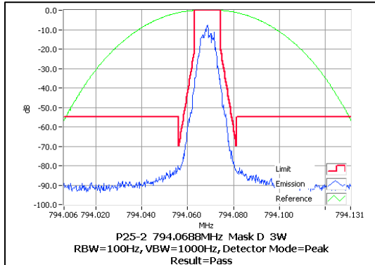
794.06875 MHz 3 W
