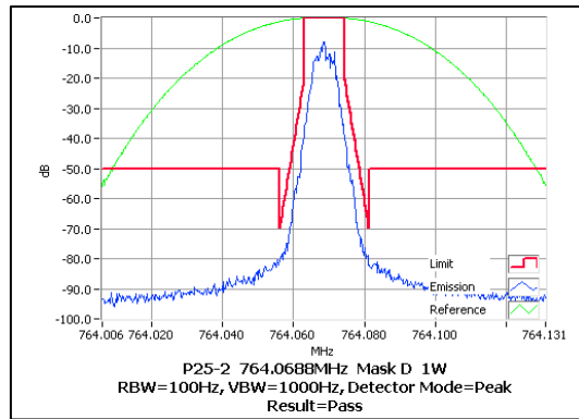
764.06875 MHz 1 W
