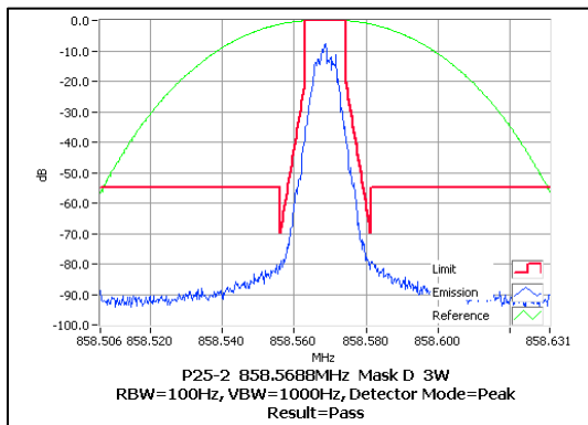
858.56875 MHz 3 W
