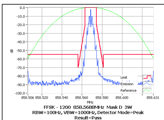
858.56875 MHz 3 W
