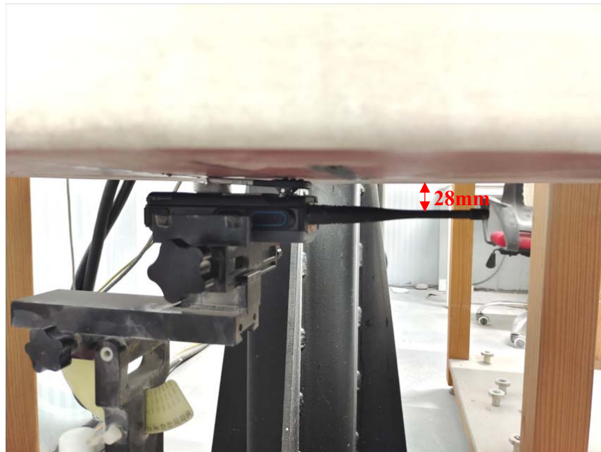
Body Back Setup Photo (0mm) -Antenna 2
