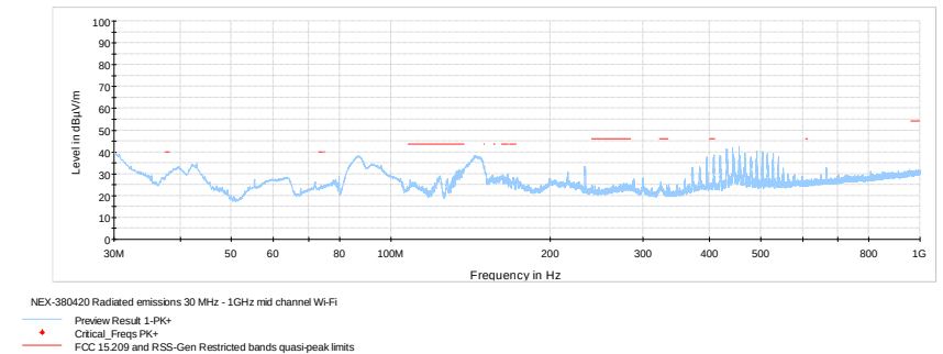
Figure 8.5-14: Radiated spurious emissions below 1 GHz, mid channel
