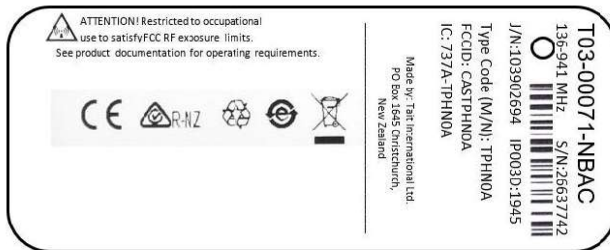
Illustration 02: Compliance Label
