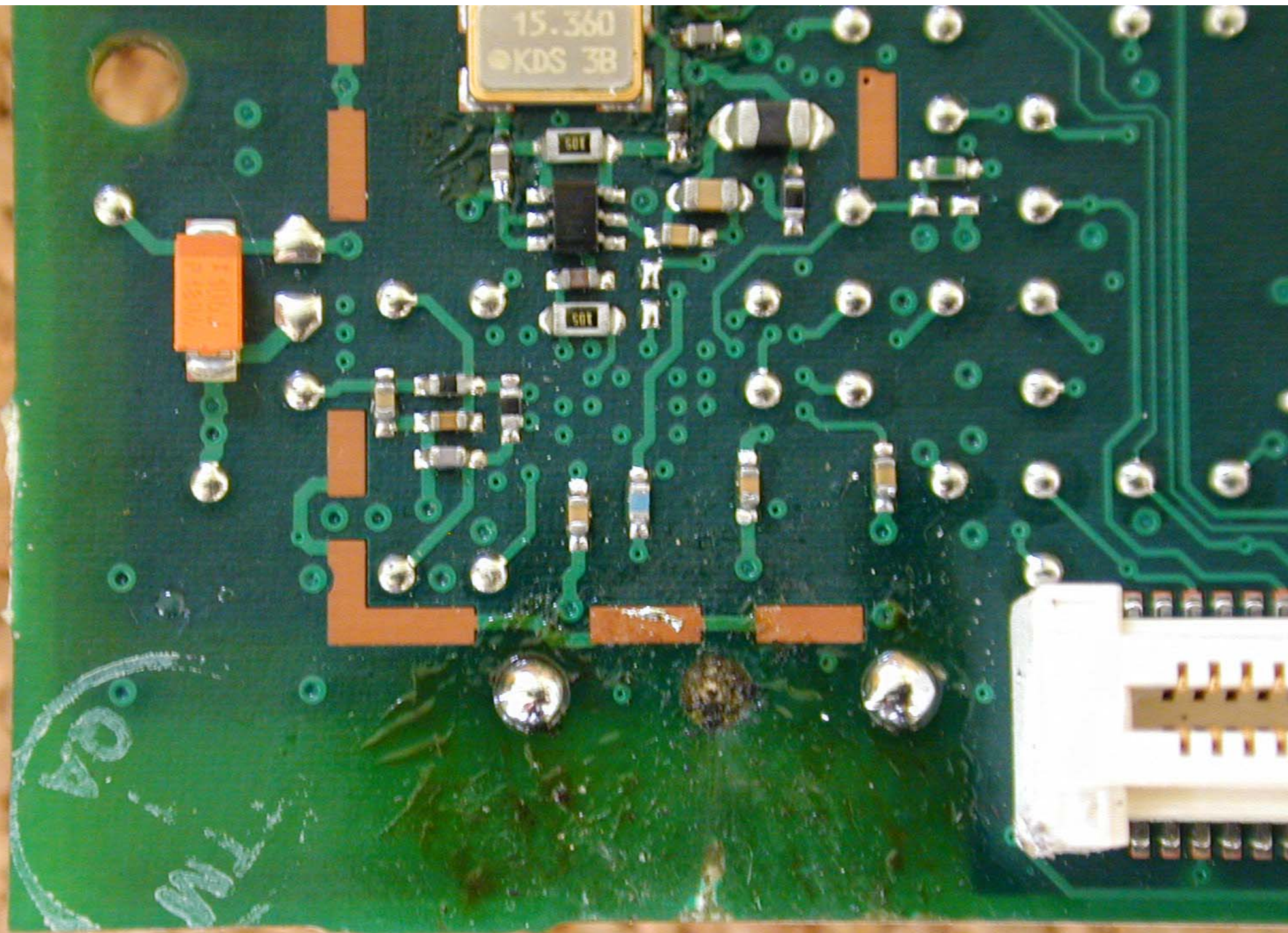
Modified DUT with SMA Adaptor (bottom)
