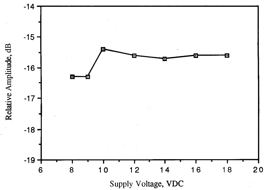
Figure 6.4. Relative emission vs. supply voltage. (310 MHz, CW)
