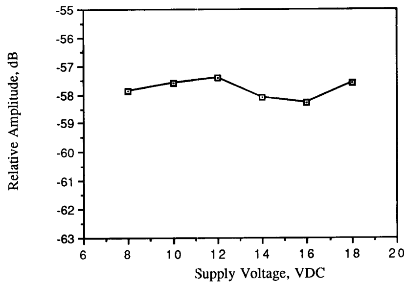
Figure 6.4. Relative emission vs. supply voltage. (310 MHz, continuous pulsed, 30% duty )
