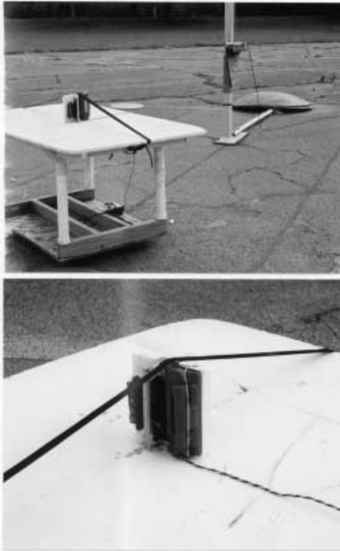
Appendix: Photos of the transmitter on the test table (Open-Site); the transmitter is tested when placed flat, on its side, and on its end. (top) Overall view, (bottom) Close-up.
