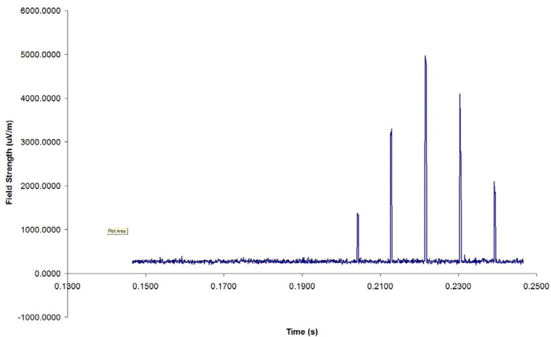
Tuning Pulse 288 MHz, 30% Duty Cycle
