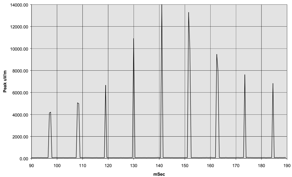
Fine Tune Pulses, 310MHz fundamental Linear Scale
