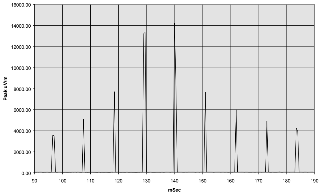
Fine Tune Pulses, 289.5MHz fundamental Linear Scale
