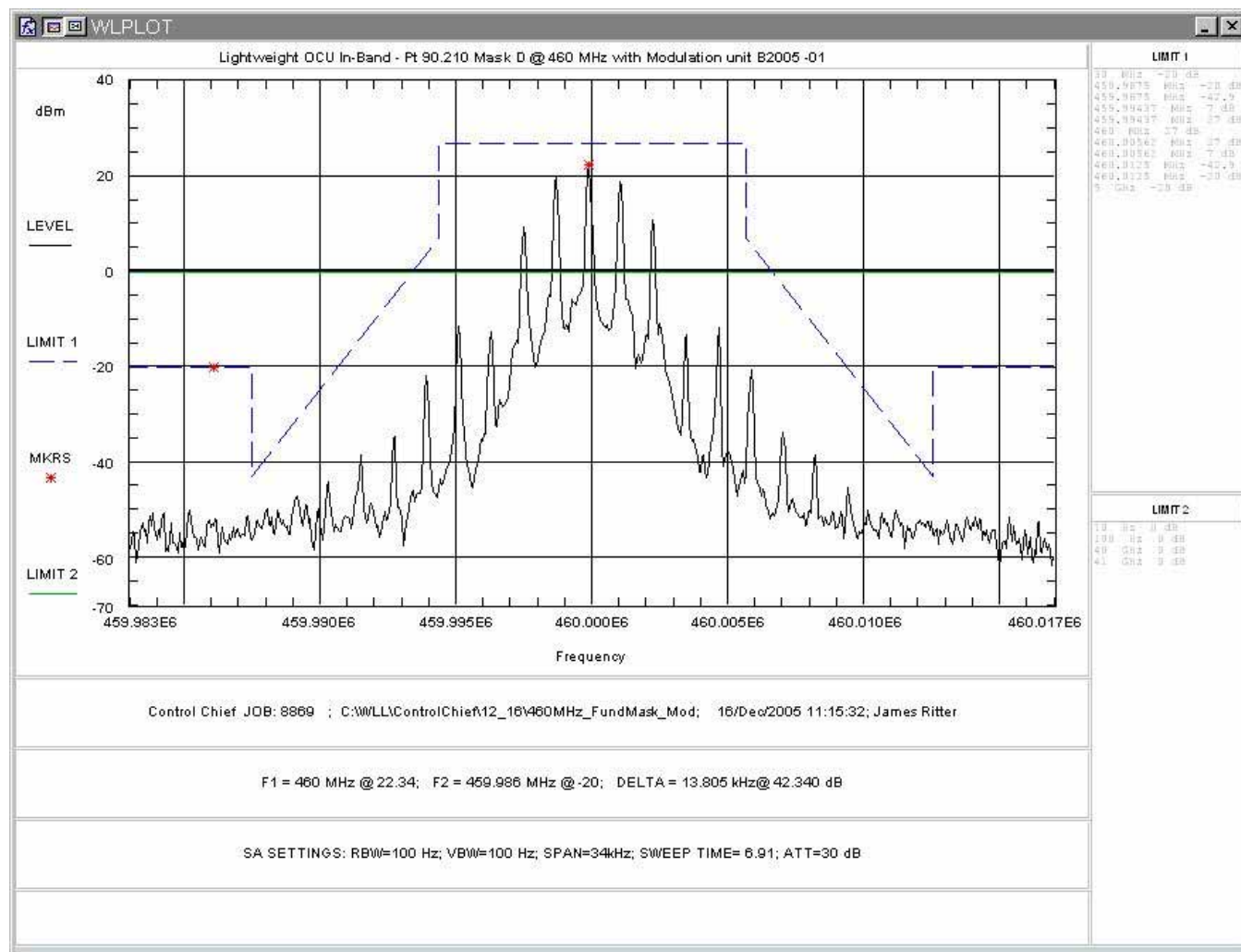
Figure 4-4. Emissions Mask, Mid Channel 460MHz, Modulated Signal
