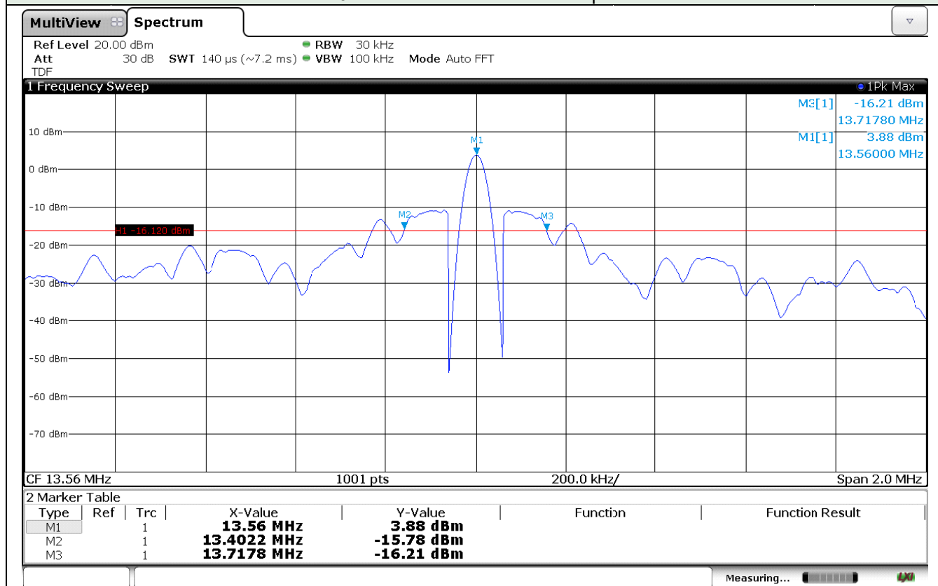
20 dB bandwidth measurement plot
