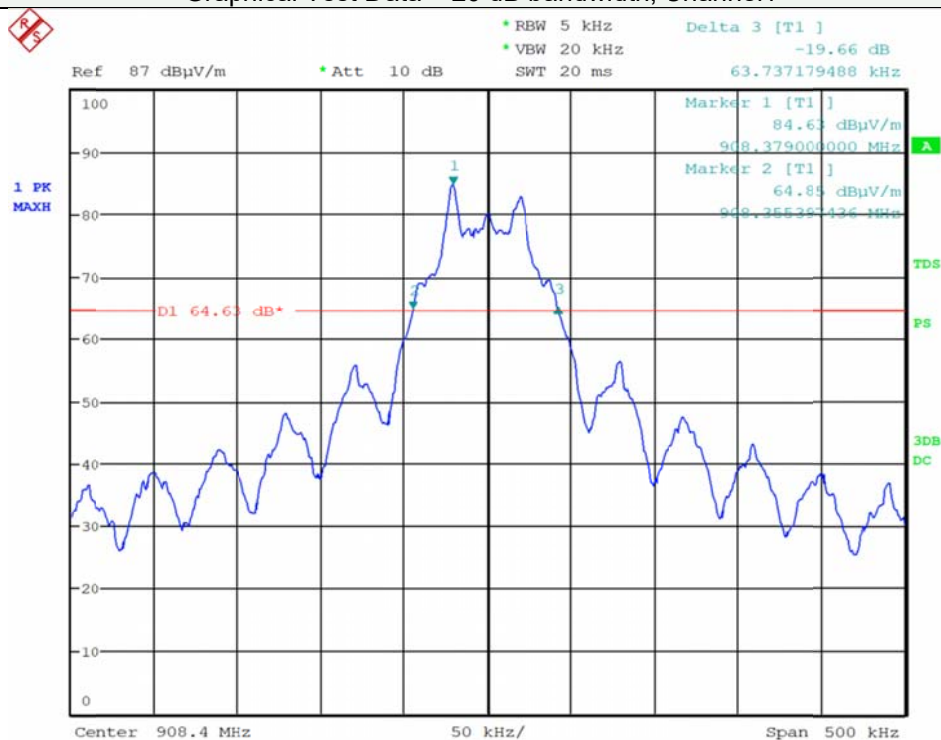
Graphical Test Data – 20 dB bandwidth, Channel1
