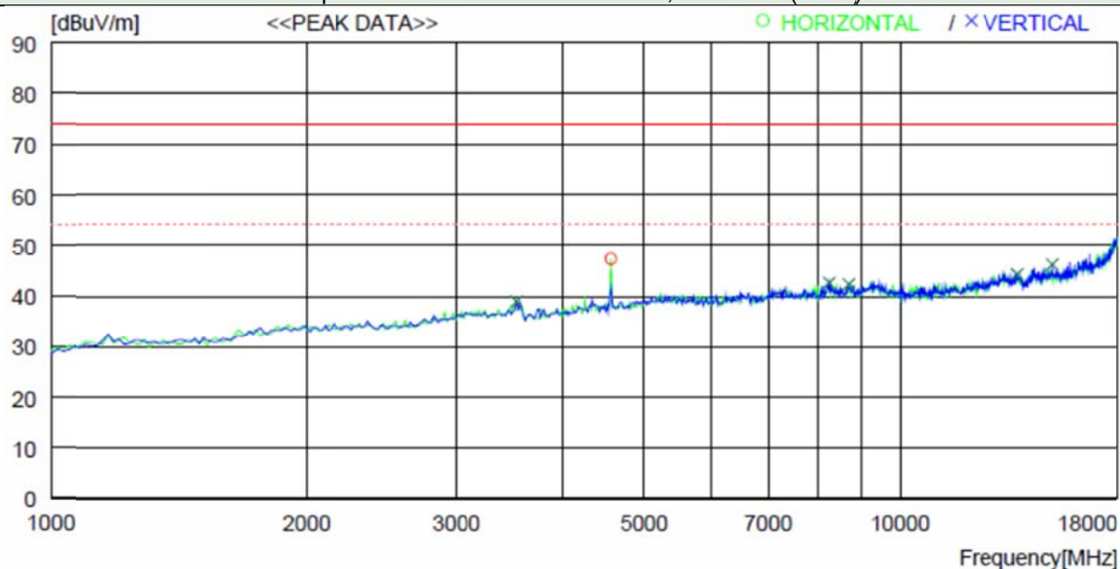
Graphical Test Data – Above 1 GHz, Channel2 (Peak)
