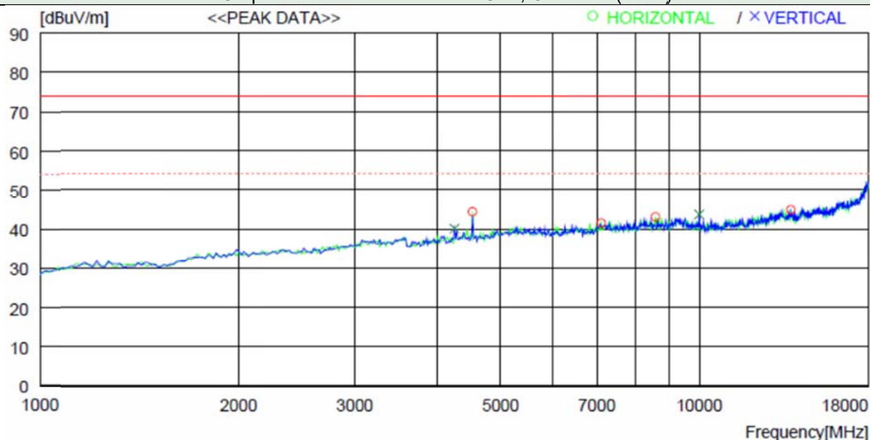
Graphical Test Data – Above 1 GHz, Channel1 (Peak)
