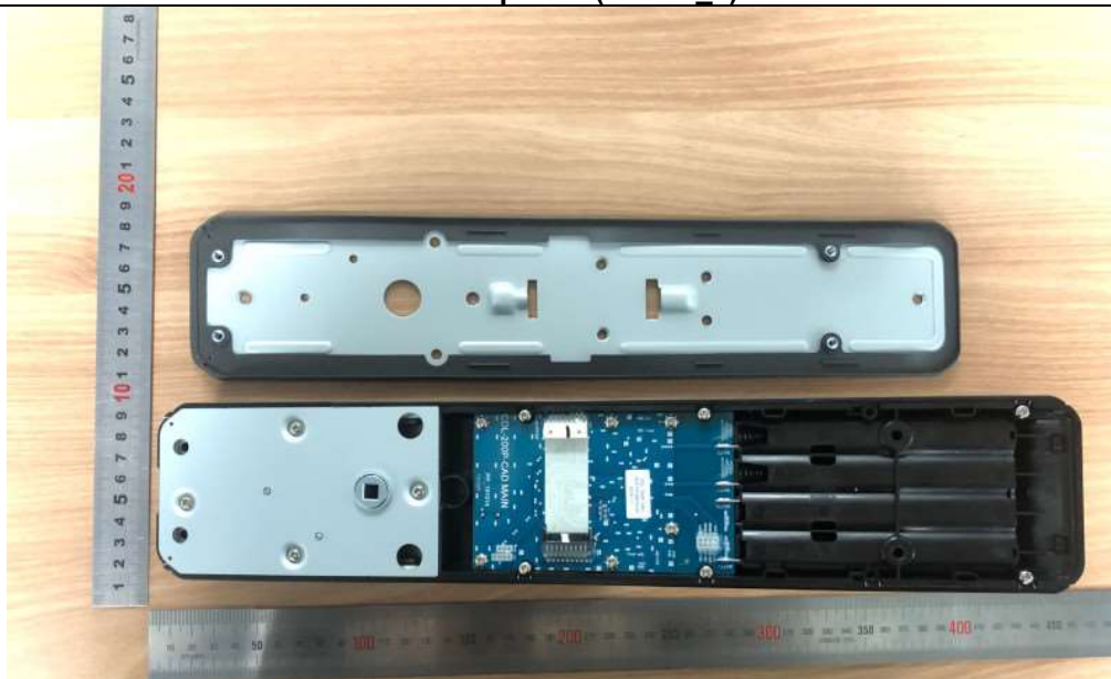
Cover opened (Indoor_1)
