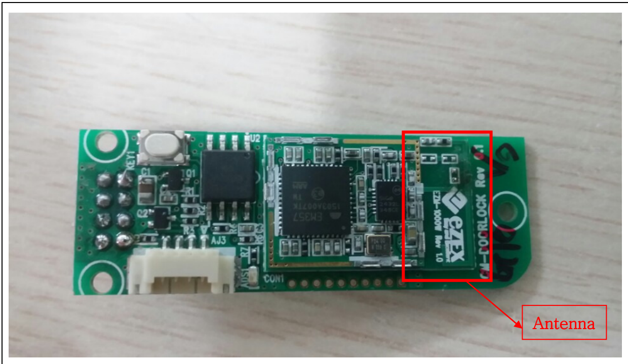
Zigbee Board - Front
