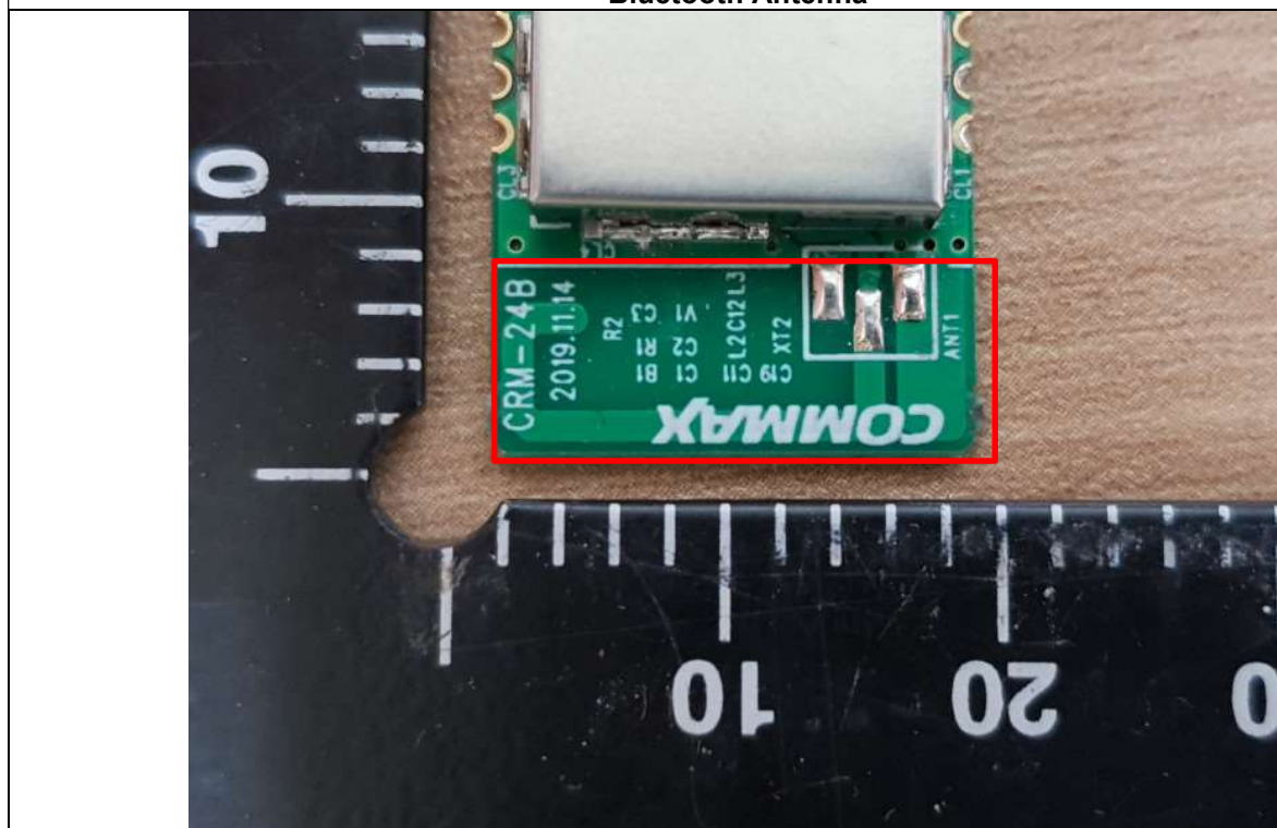
Bluetooth Antenna
