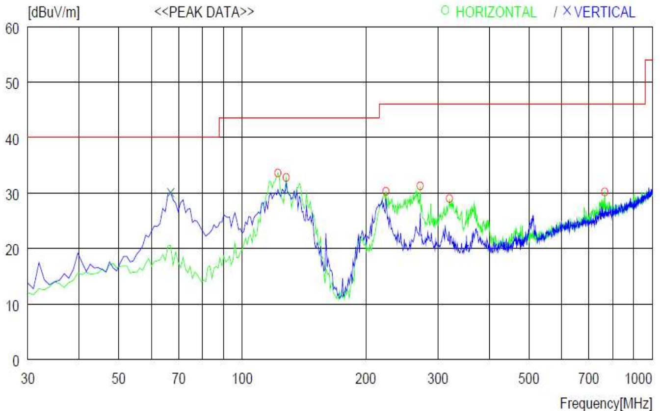
Graphical Test Data – Below 1 GHz – Low Channel (Peak)
