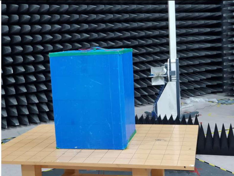
18 GHz – 25 GHz
