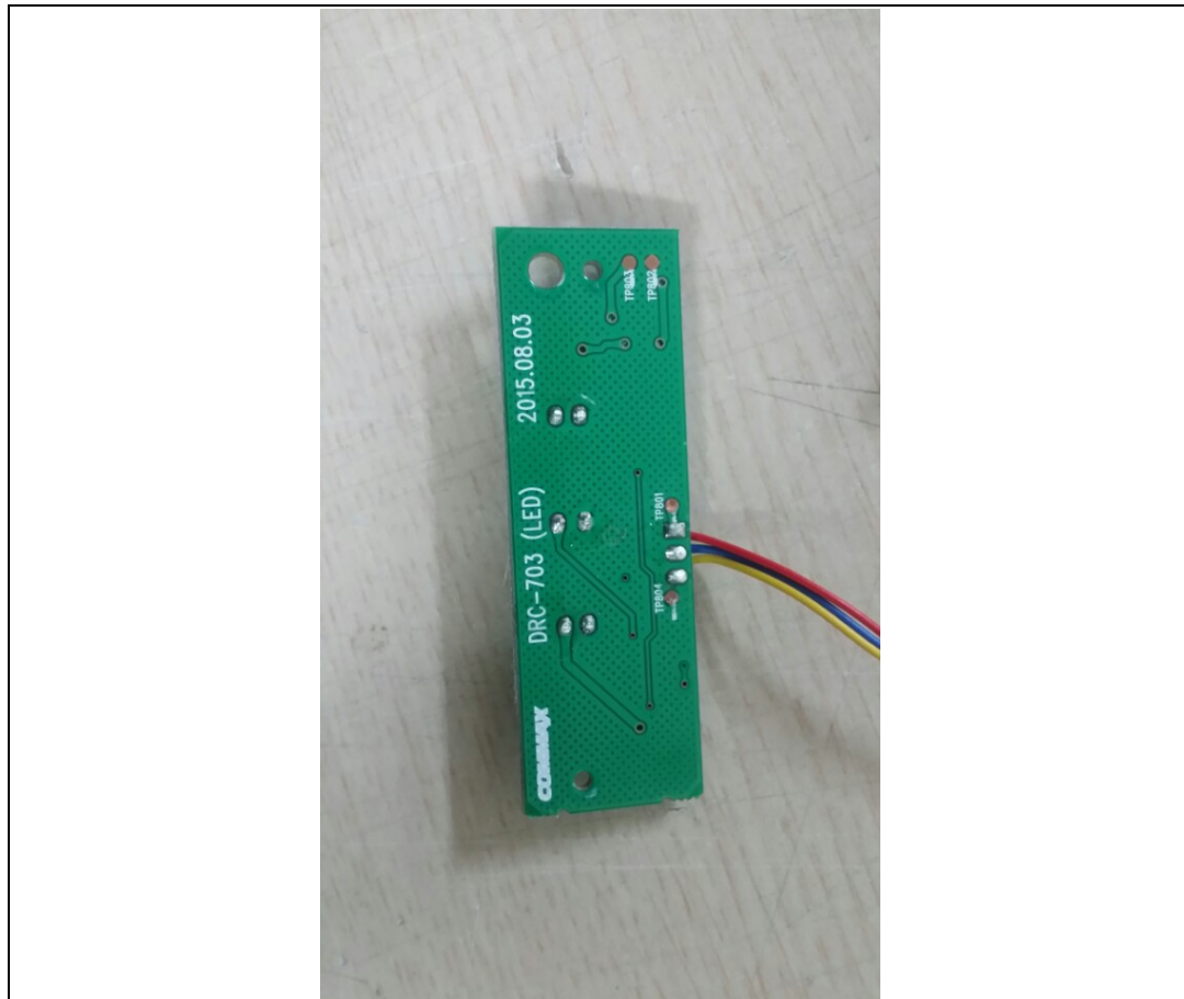
Sub Board - Rear
