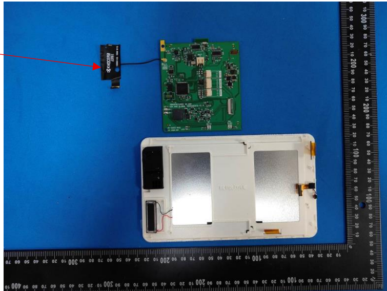
915MHz Antenna
